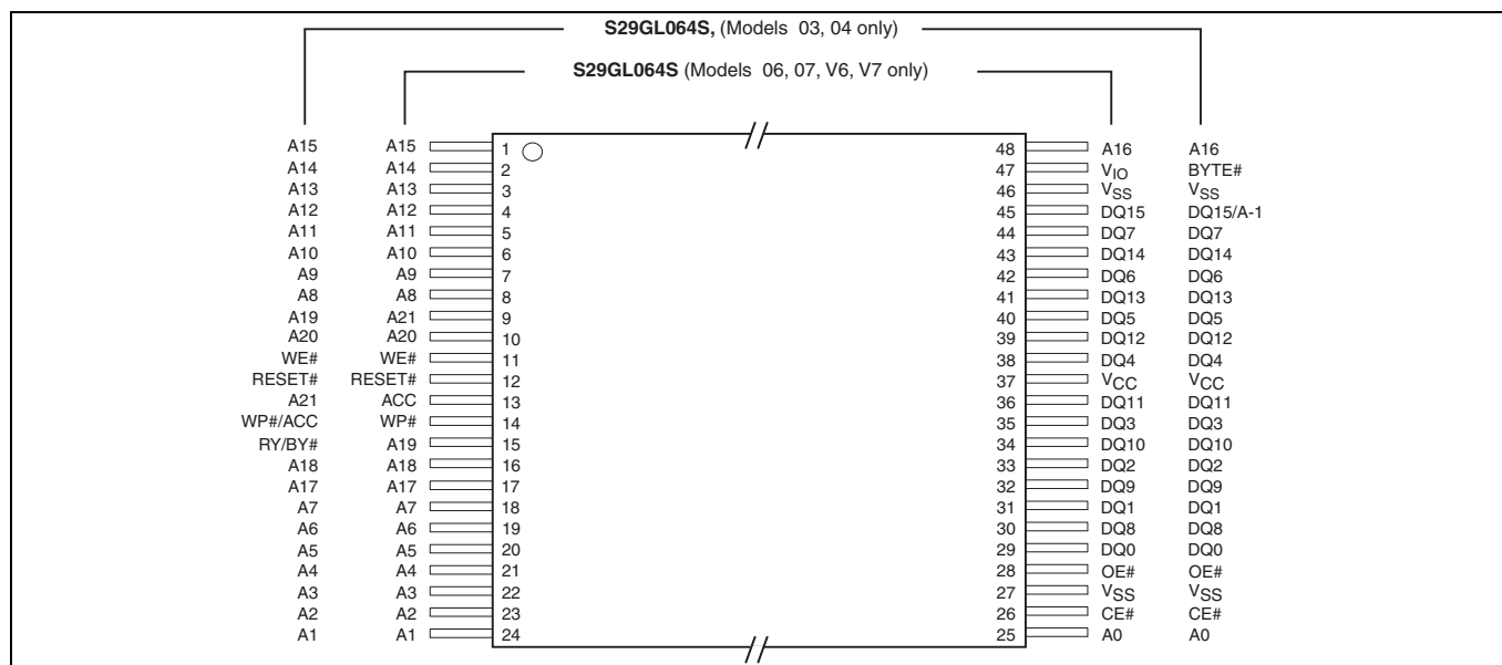
Figure 2 48-lead standard TSOP
