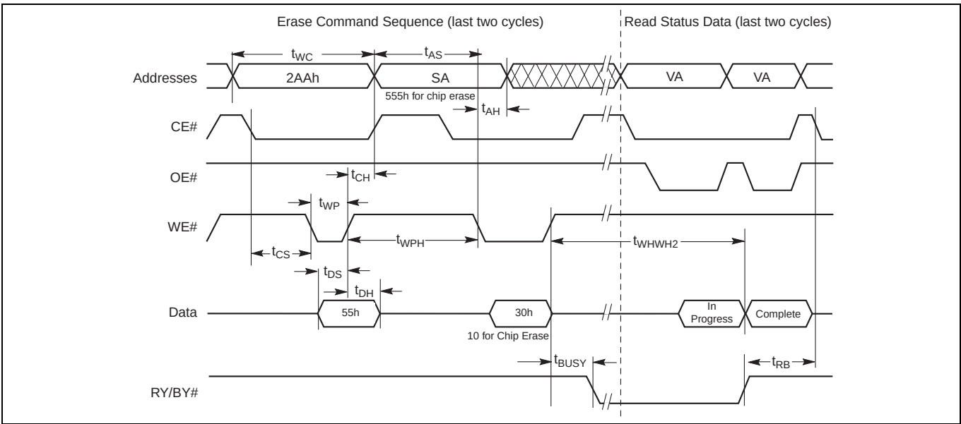
Figure 35 Chip / sector erase operation timings
