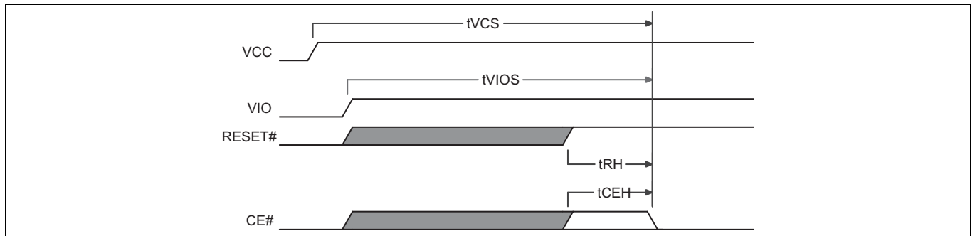
Figure 21 Power-up diagram
