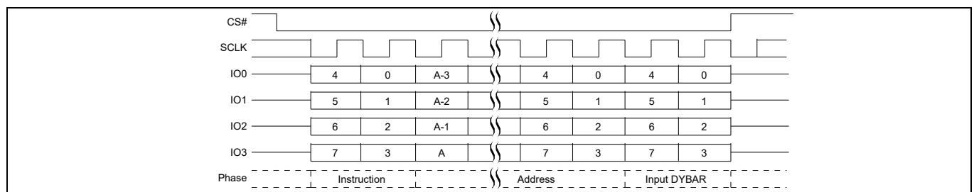
Figure 94 DYBWR QPI mode command sequence [59, 60]
