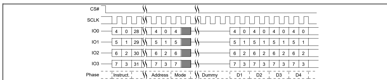
Figure 71 Quad I/O Read command sequence (4-byte address, ECh or EBh [CR2V[7] = 1]) QPI mode
