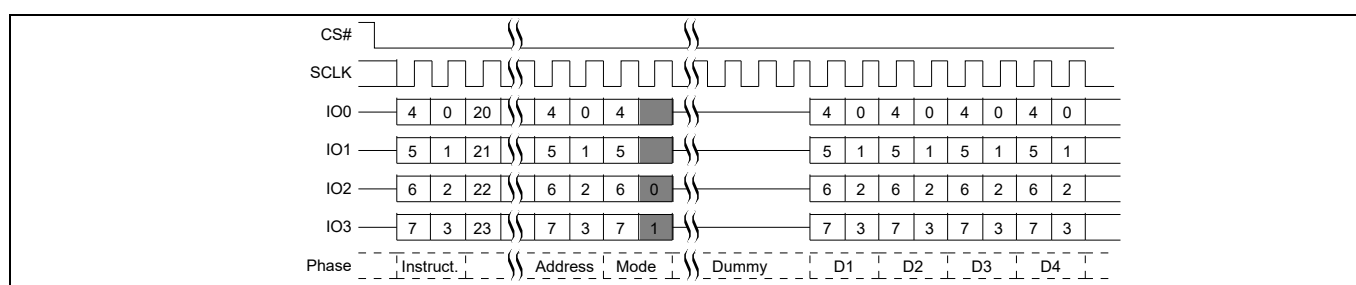
Figure 69 Quad I/O Read command sequence (3-byte address, EBh [CR2V[7] = 0]) QPI mode
