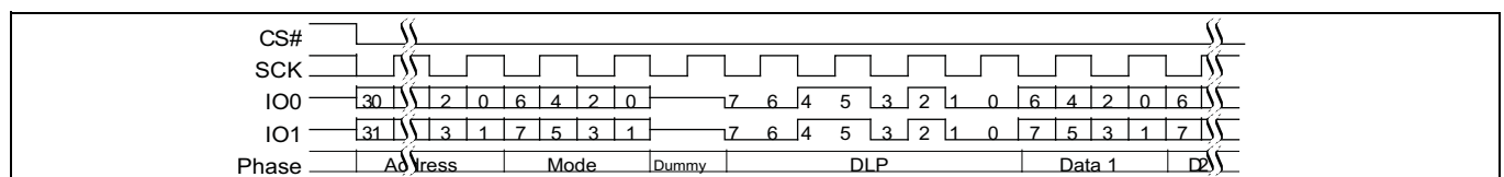
Figure 92 Continuous DDR dual I/O read subsequent access (4-byte address, EHPLC = 01b)
