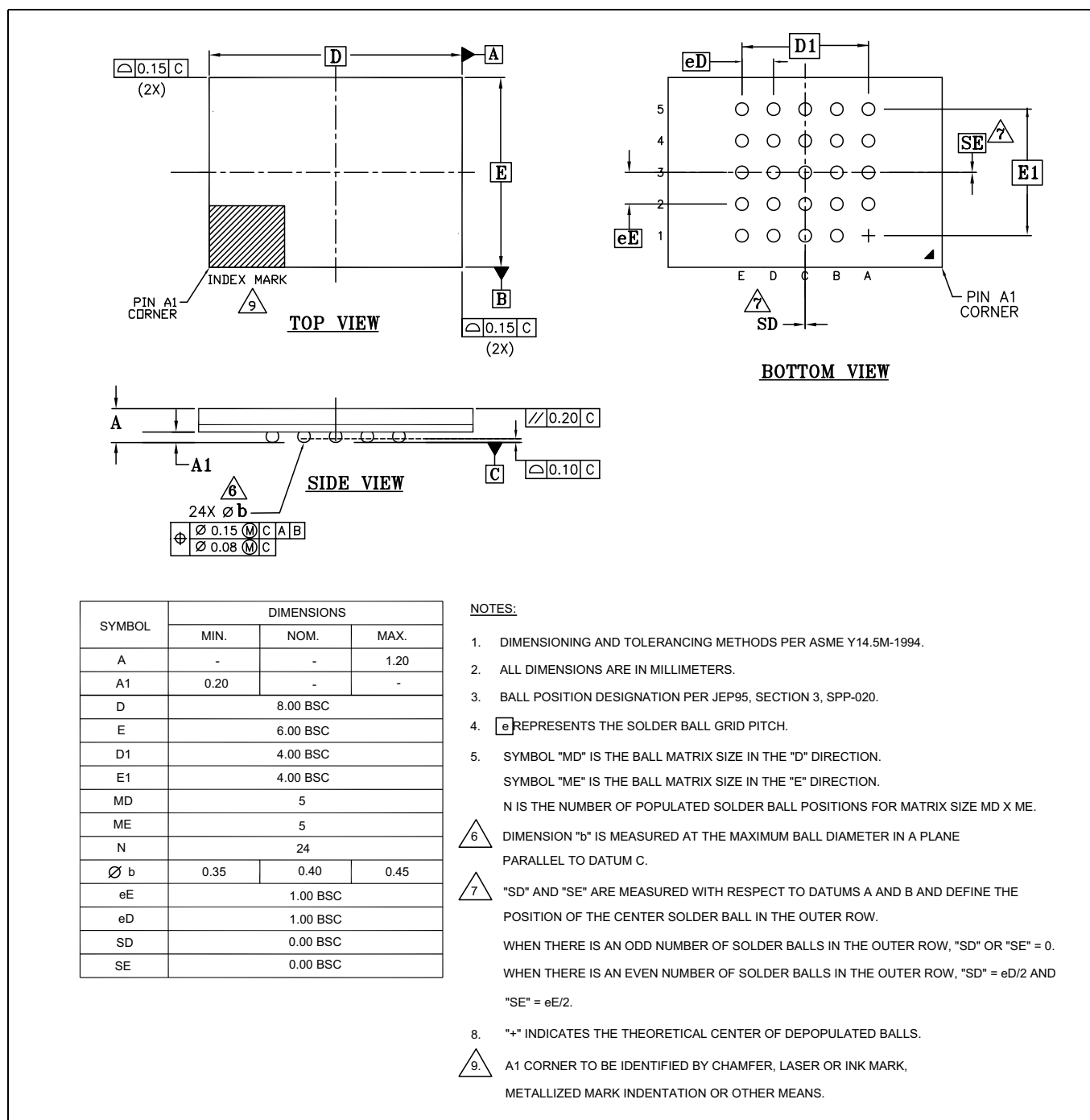
Figure 42 Ball grid array 24-ball 6x8 mm (FAB024)
