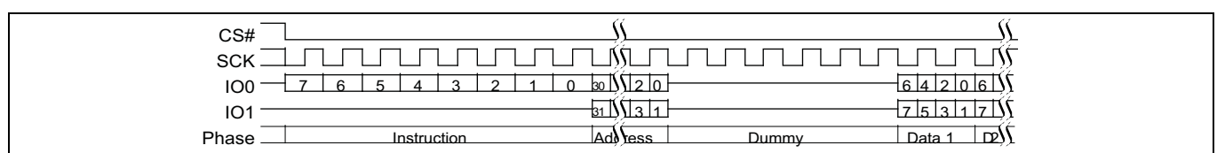
Figure 93 DDR dual I/O read (4-byte address, BEh or BDh [ExtAdd = 1], HPLC = 00b)
