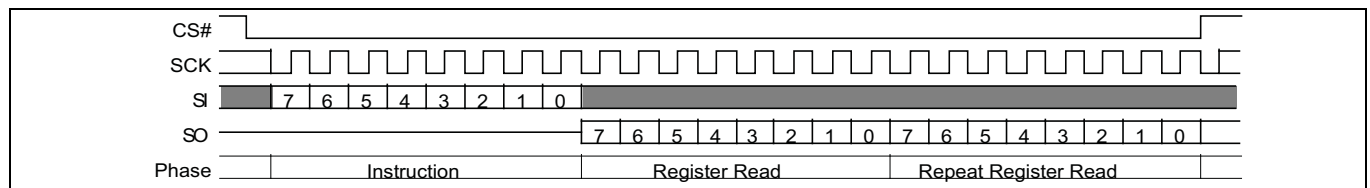
Figure 108 ASPRD command
