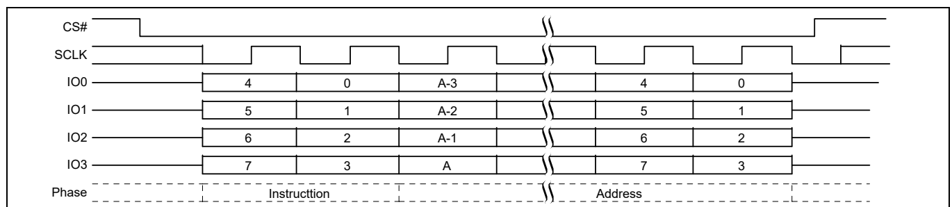
Figure 85 Block Erase (BE D8h or 4BE DCh) QPI mode command sequence [49]
