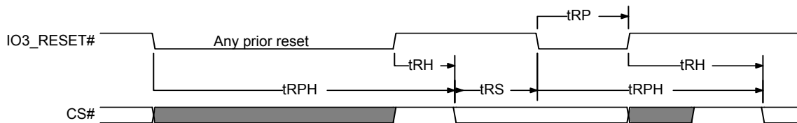
Figure 5.8 Hardware Reset when Quad or QPI Mode is not enabled and IO3 / RESET# is Enabled
