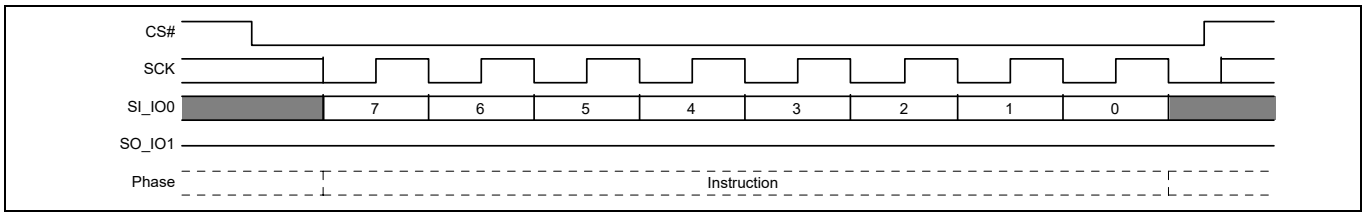
Figure 88 Program or Erase Suspend command sequence
