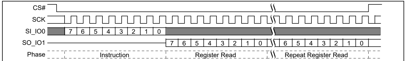
Figure 38 Read Configuration Register (RDCR1) (RDCR2) (RDCR3) command sequence
