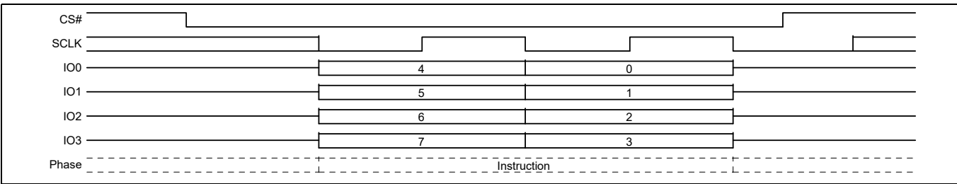
Figure 42 Write Enable (WREN) command sequence QPI mode
