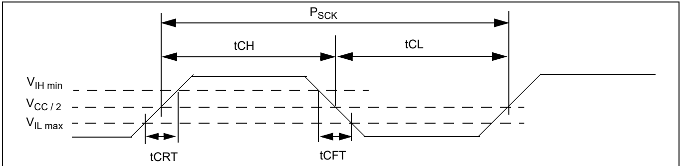
Figure 142 Clock timing
