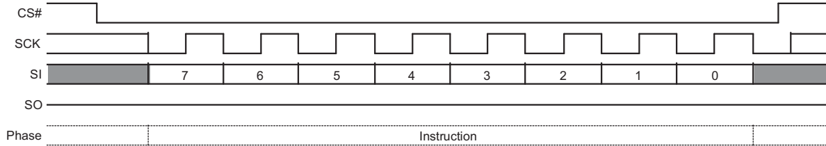
Figure 5. Stand Alone Instruction Command
