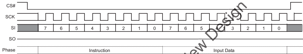
Figure 6. Single Bit Wide Input Command
