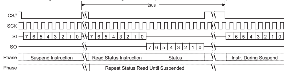
Figure 40. Erase / Program Suspend Command Sequence
