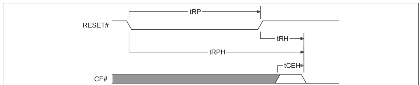
Figure 22 Hardware reset
