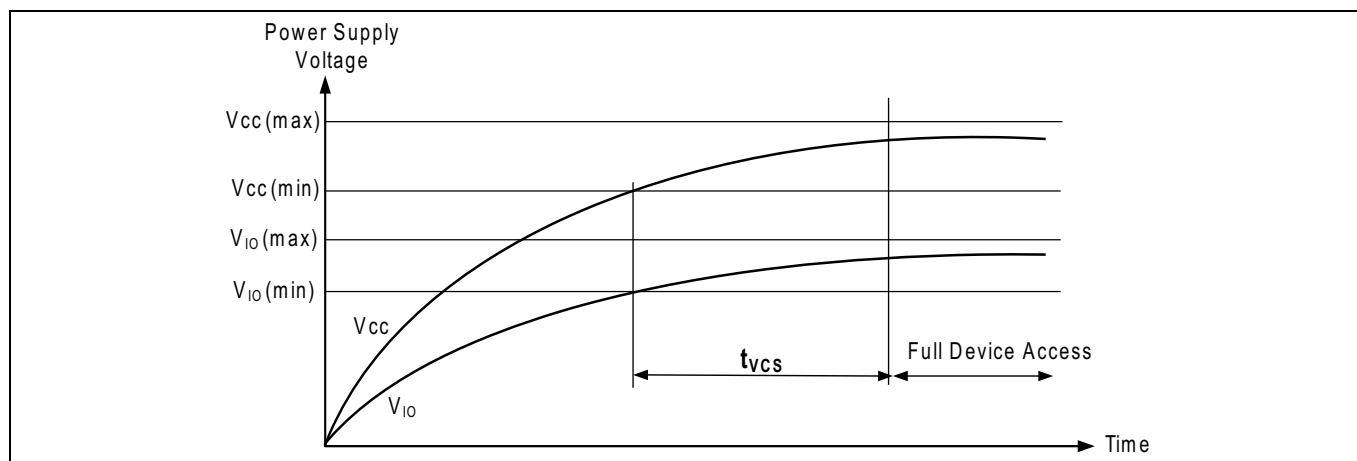
Figure 15 Power-up
