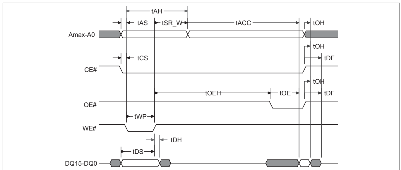
Figure 29 Write to Read ( t_{ACC} ) operation timing diagram
