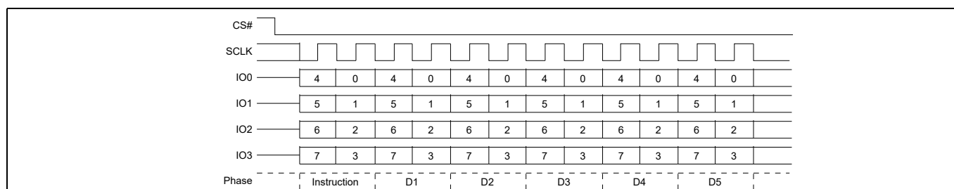
Figure 44 Read Identification (RDID) QPI mode command
