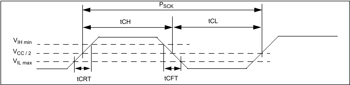
Figure 28 Clock timing
