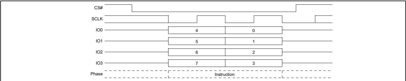
Figure 53 Clear Status Register (CLSR) command sequence QPI mode
