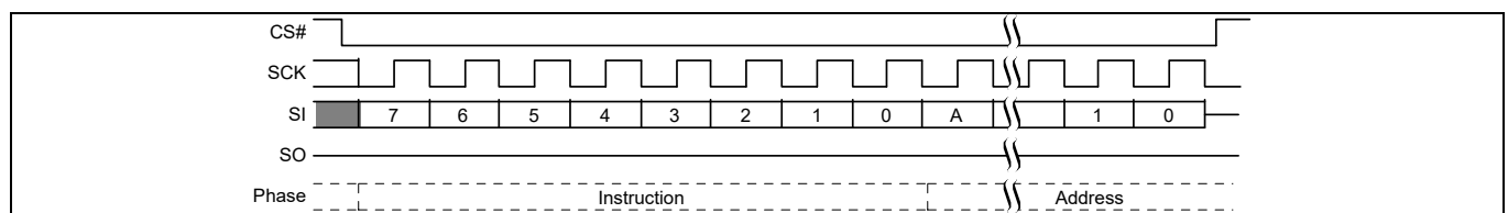
Figure 79 Sector Erase (SE D8h or 4SE DCh) command sequence [54]
