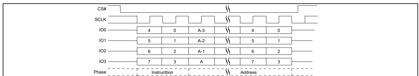
Figure 80 Sector Erase (SE D8h or 4SE DCh) QPI mode command sequence [54]
