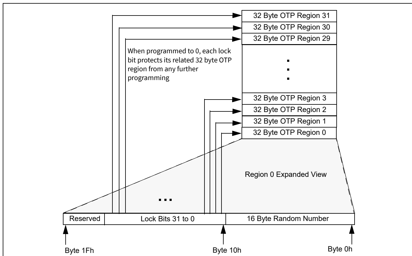
Figure 40 OTP address space
