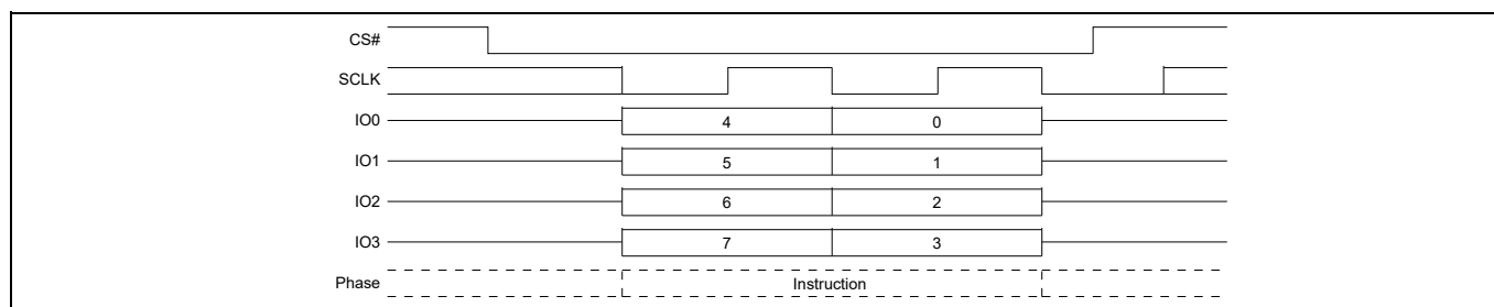
Figure 89 Erase or Program Resume command sequence QPI mode
