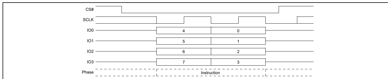
Figure 109 RES command sequence QPI mode
