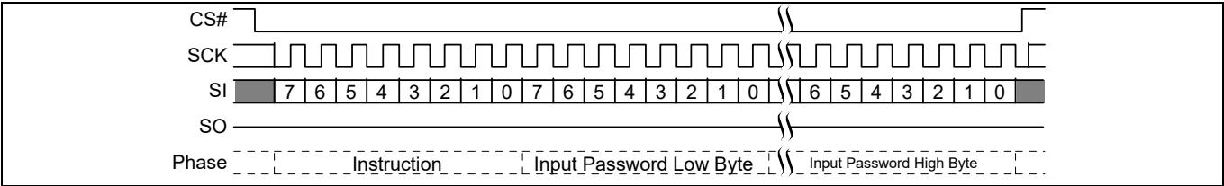
Figure 101 Password Unlock command sequence
