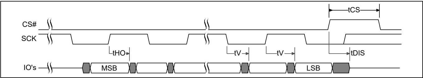
Figure 34 SPI DDR output timing
