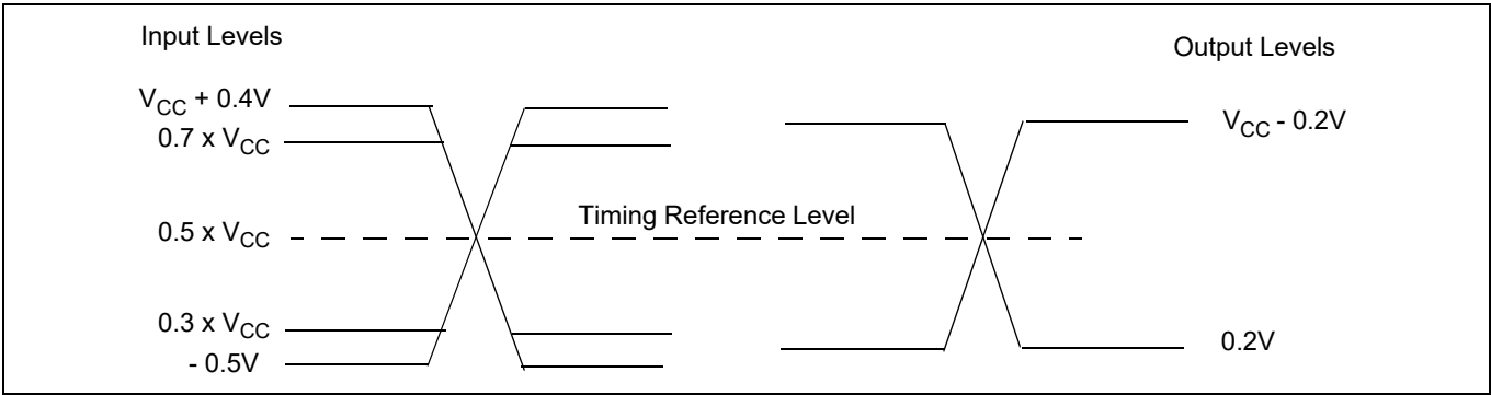
Figure 22 Input, output, and timing reference levels
