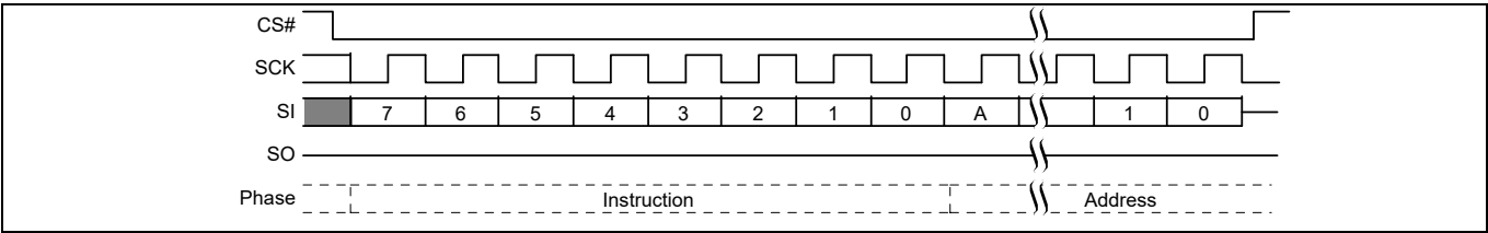
Figure 77 Parameter Sector Erase (P4E 20h or 4P4E 21h) command sequence [53]
