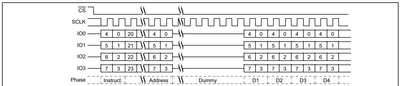
Figure 55 ECCRD (19h), Quad All Mode, CR2[7] = 0, command sequence
