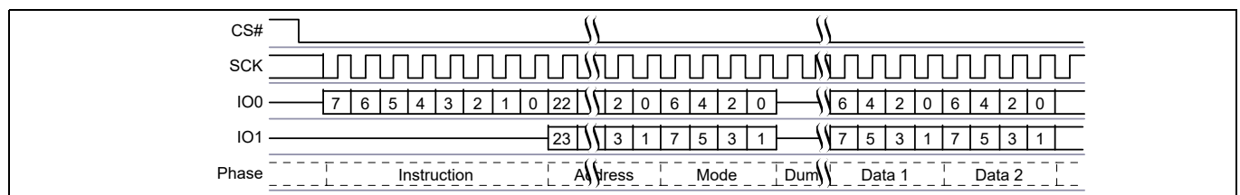
Figure 66 Dual I/O Read command sequence (3-byte address, BBh [CR2V[7] = 0]) [48]
