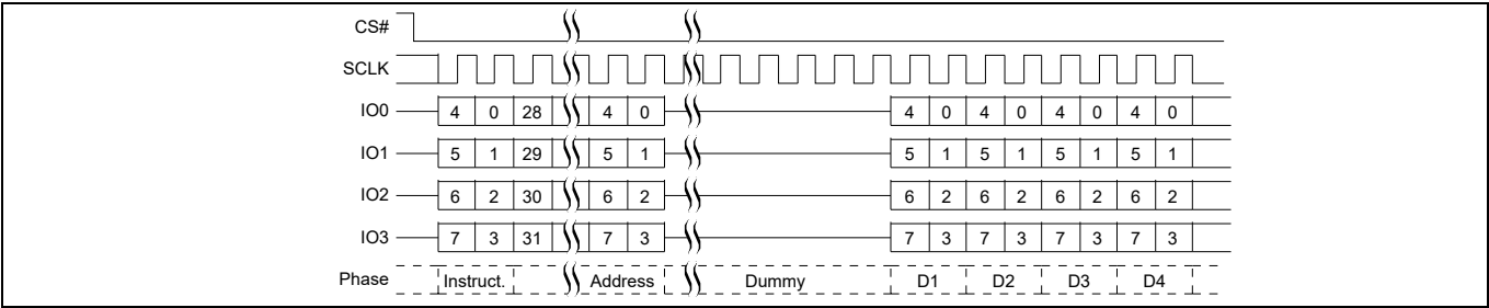
Figure 62 Read Any Register, QPI Mode, CR2[7] = 1 command sequence
