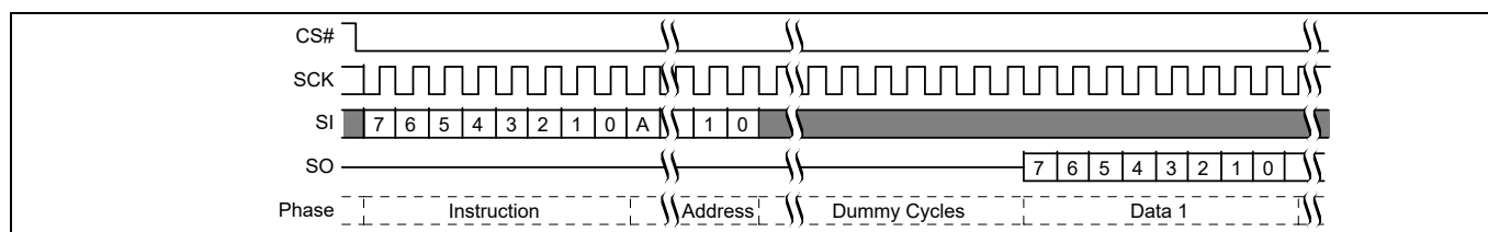
Figure 65 Fast Read (FAST_READ) command sequence (3-byte address, 0Bh [CR2V[7] = 0]) [47]
