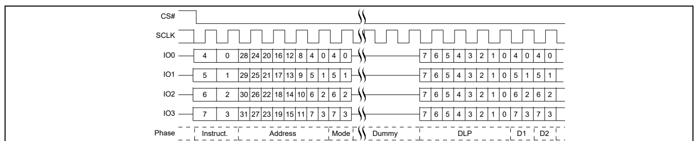
Figure 15 DDR Quad I/O Read in QPI mode
