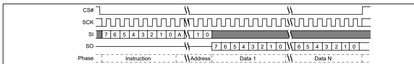
Figure 64 Read command sequence (3-byte address, 03h or 13h) [46]
