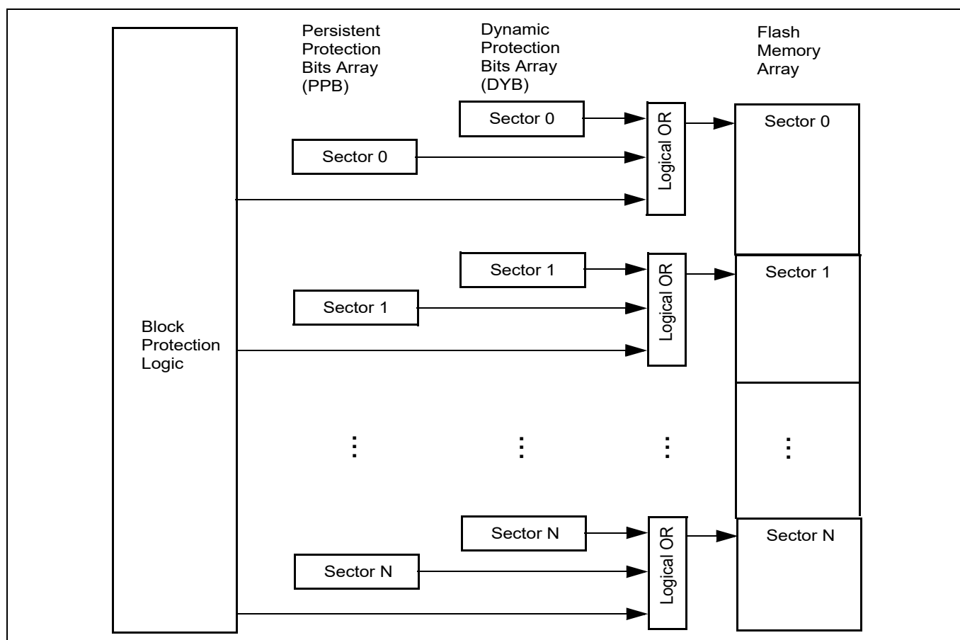
Figure 41 Sector protection control
