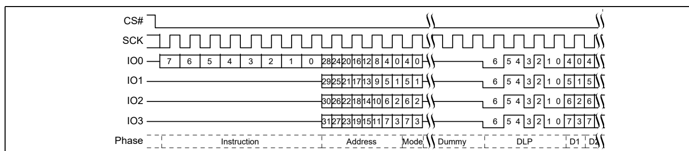
Figure 73 DDR Quad I/O Read initial access (4-byte address, EEh or EDh [CR2V[7] = 1]) [49]
