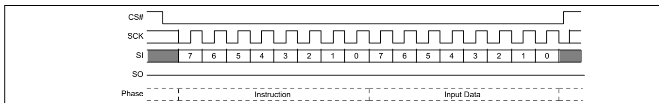
Figure 57 Write VDLR (WVDLR) command sequence
