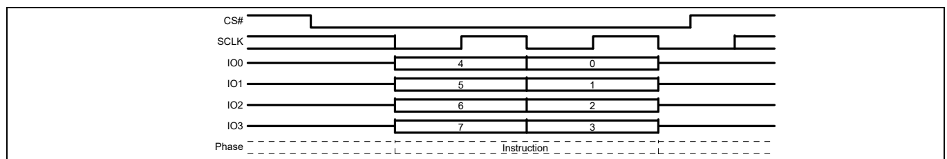
Figure 103 Software Reset command sequence QPI mode
