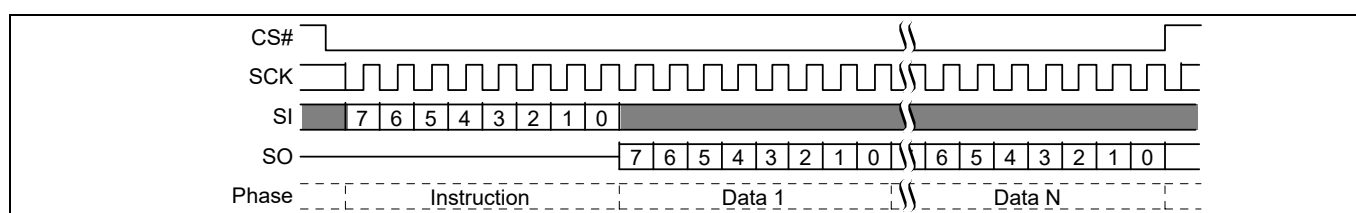
Figure 43 Read Identification (RDID) command sequence
