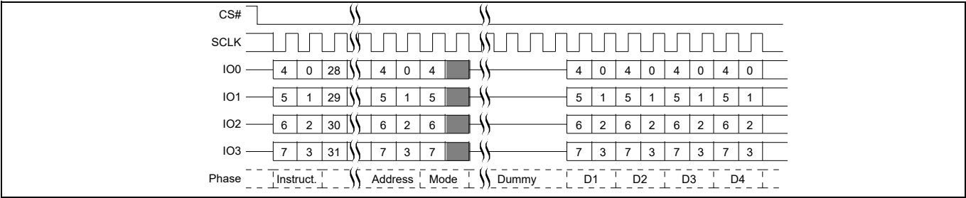
Figure 71 Quad I/O Read command sequence (4-byte address, ECh or EBh [CR2V[7] = 1]) QPI mode
