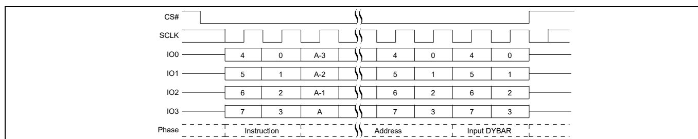
Figure 94 DYBWR QPI mode command sequence [59, 60]
