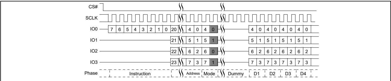
Figure 68 Quad I/O Read command sequence (3-byte address, EBh [CR2V[7] = 0])
