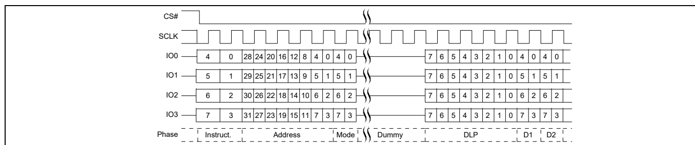
Figure 74 DDR Quad I/O Read initial access (4-byte address, EEh or EDh [CR2V[7] = 1]) QPI mode [50]
