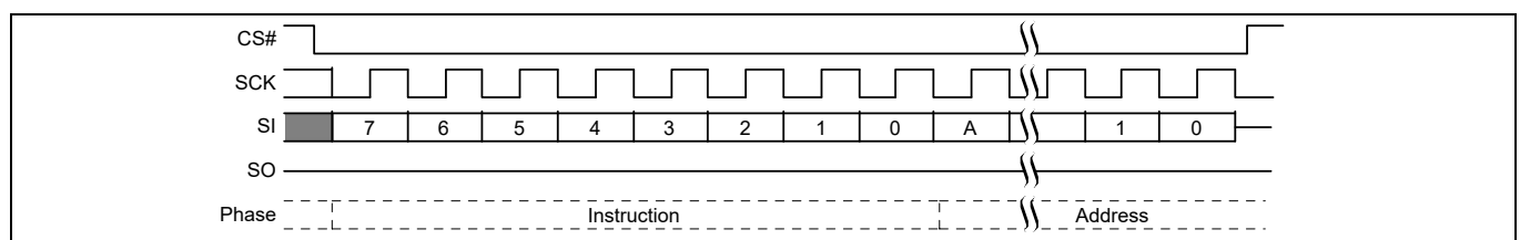
Figure 96 PPBP command sequence [63, 64]
