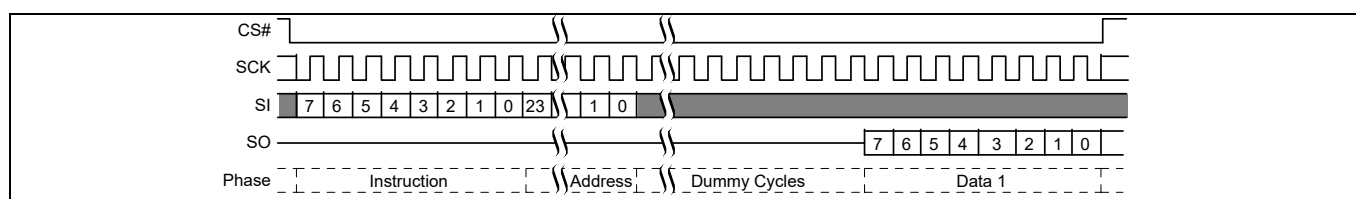
Figure 46 RSFDP command sequence
