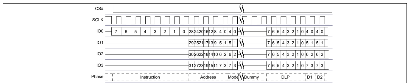
Figure 14 DDR Quad I/O Read
