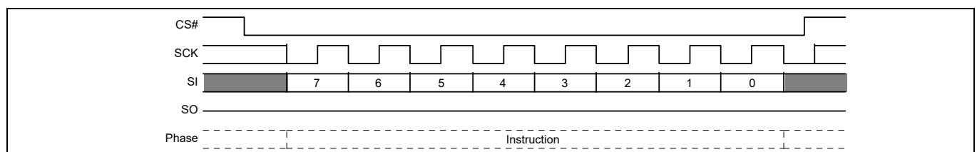
Figure 102 Software Reset command sequence
