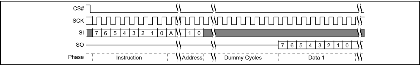
Figure 60 Read Any Register Read command sequence [45]
