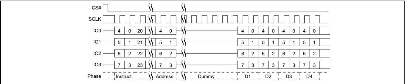
Figure 61 Read Any Register, QPI Mode, CR2[7] = 0, command sequence
