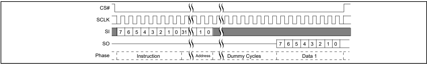
Figure 10 Single Bit Wide I/O command with latency
