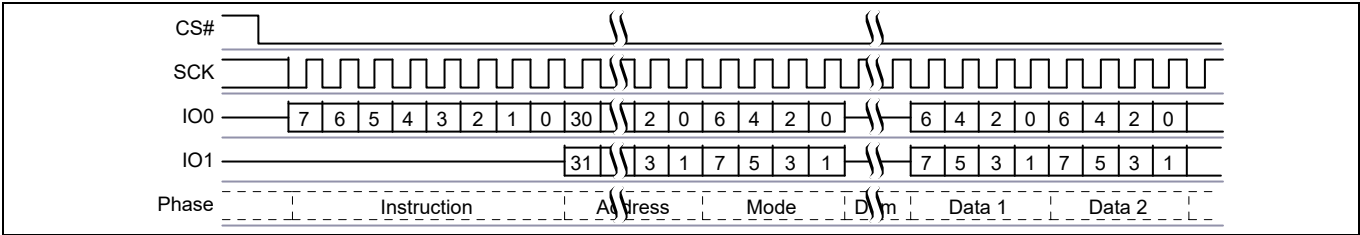
Figure 11 Dual I/O command
