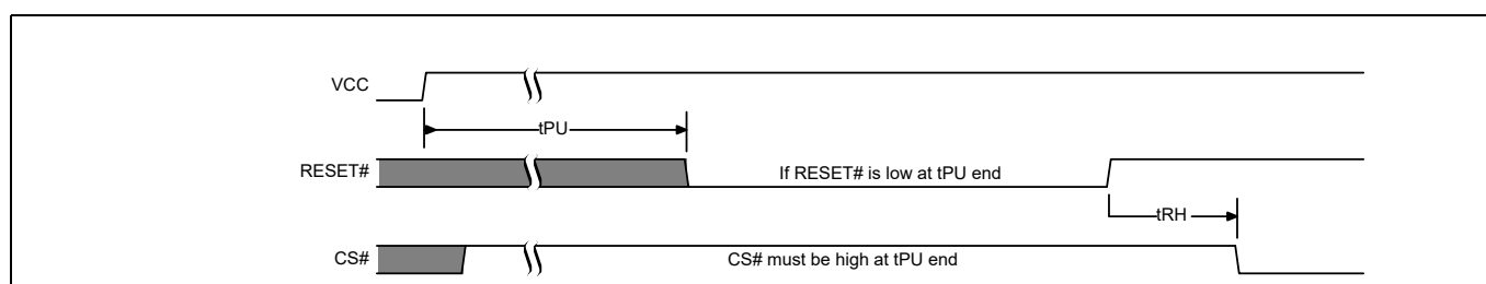
Figure 23 Reset LOW at the end of POR
