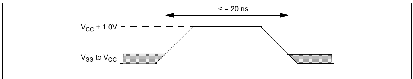
Figure 17 Maximum positive overshoot waveform
