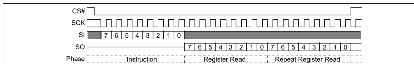
Figure 58 DLP Read (DLPRD) command sequence
