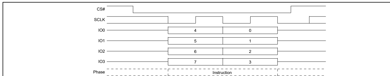
Figure 51 Write Disable (WRDI) command sequence QPI mode
