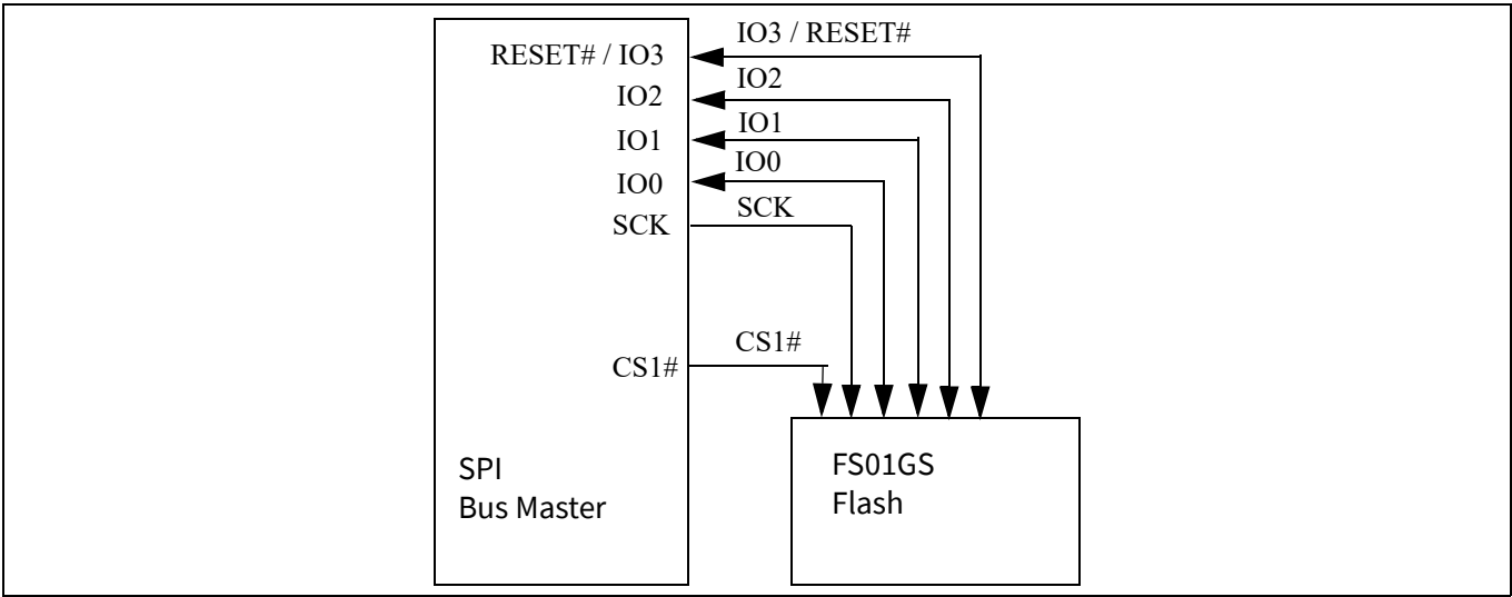
Figure 3 Bus master and memory devices on the SPI bus - Quad bit data path
