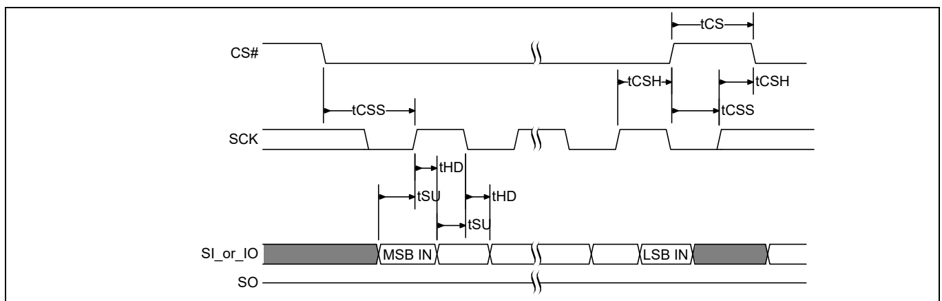
Figure 33 SPI DDR input timing
