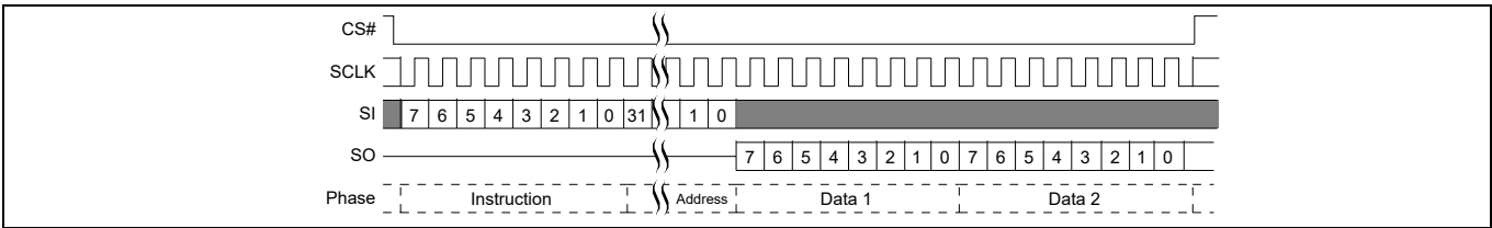
Figure 9 Single Bit Wide I/O command without latency
