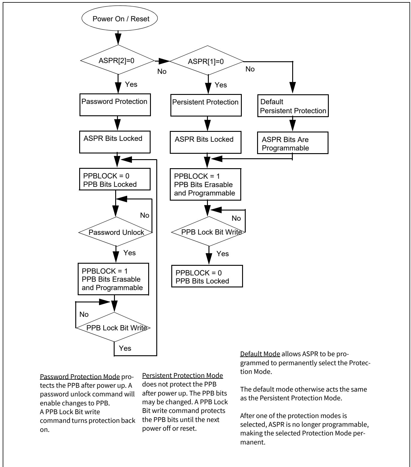
Figure 42 Advanced sector protection overview
