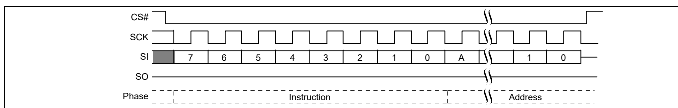
Figure 83 EES command sequence [56]
