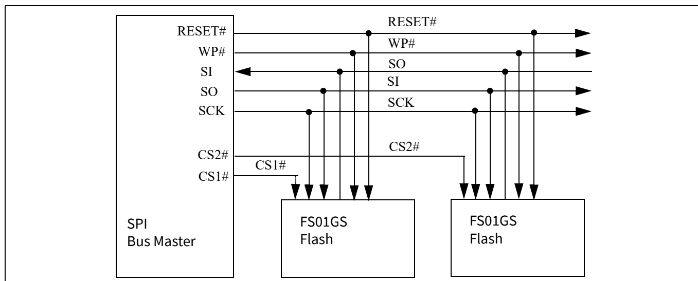
Figure 1 Bus master and memory devices on the SPI bus - Single bit data path
