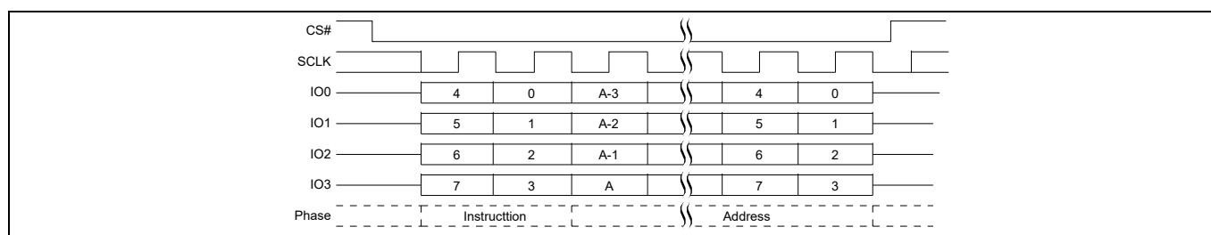
Figure 82 Bulk Erase Addressed command sequence QPI mode [55]
