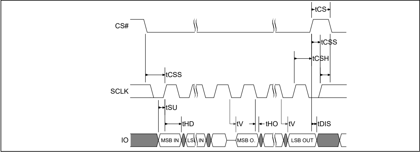
Figure 31 SPI SDR MIO timing
