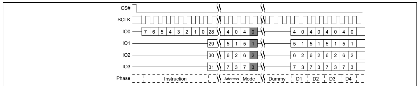
Figure 12 Quad I/O command
