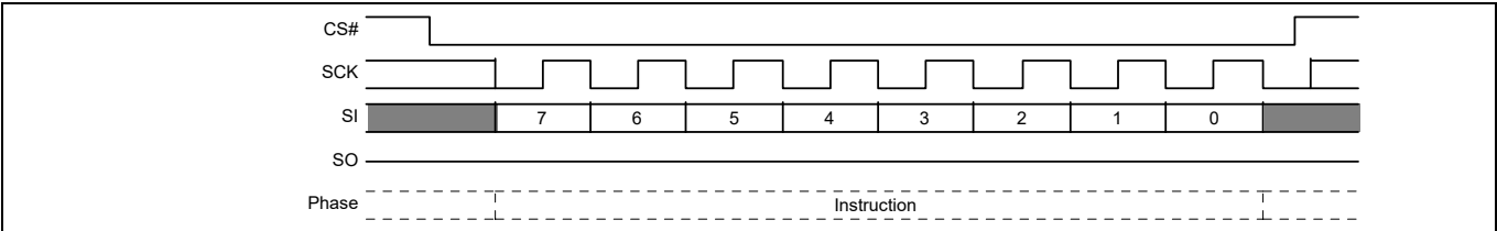
Figure 52 Clear Status Register (CLSR) command sequence
