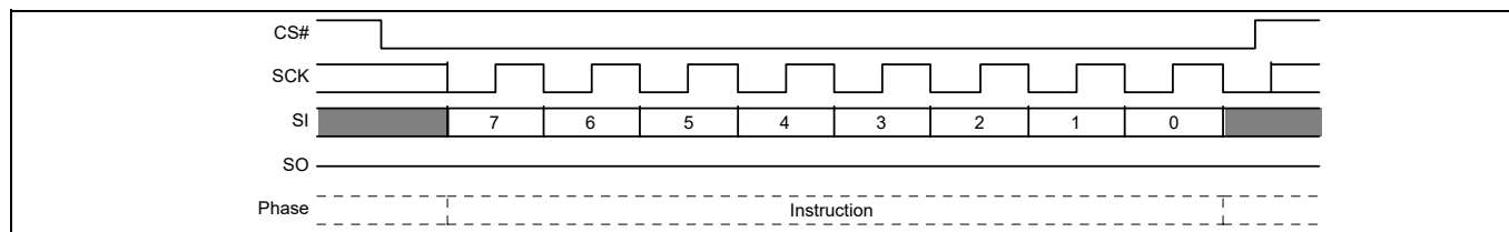
Figure 88 Erase or Program Resume command sequence
