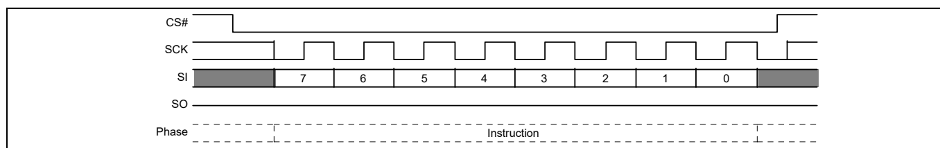
Figure 104 Mode Bit Reset command sequence
