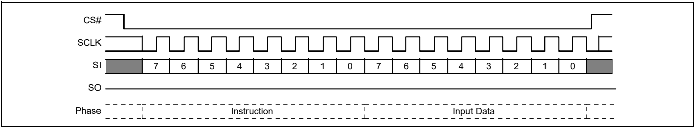
Figure 7 Single Bit Wide Input command
