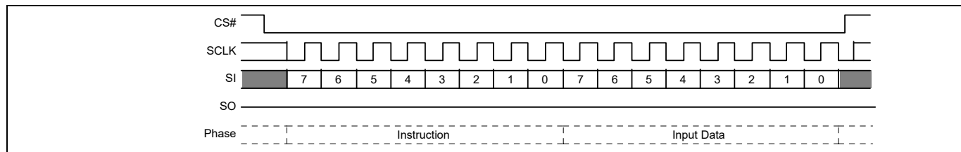
Figure 63 Set Burst Length command sequence
