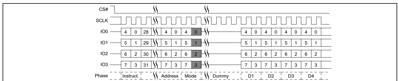
Figure 13 Quad I/O Read command in QPI mode
