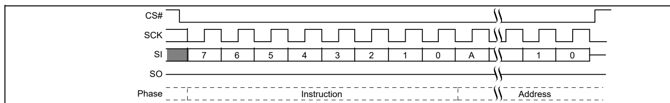
Figure 81 Bulk Erase Addressed command sequence [55]
