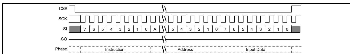
Figure 93 DYBWR command sequence [59, 60]
