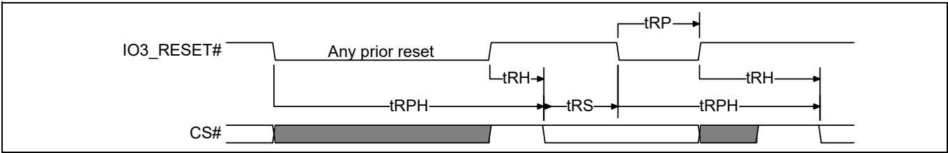
Figure 26 Hardware Reset when Quad mode is not enabled and IO3 / Reset# is enabled
