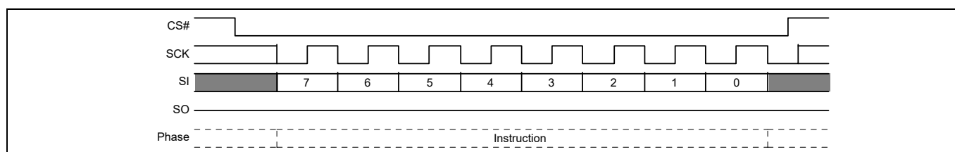
Figure 97 PPB Erase command sequence
