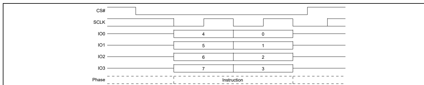
Figure 105 Mode Bit Reset command sequence QPI mode
