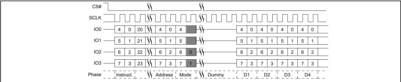
Figure 69 Quad I/O Read command sequence (3-byte address, EBh [CR2V[7] = 0]) QPI mode
