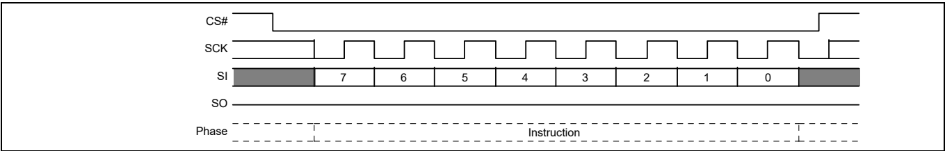
Figure 86 Erase or Program Suspend command sequence
