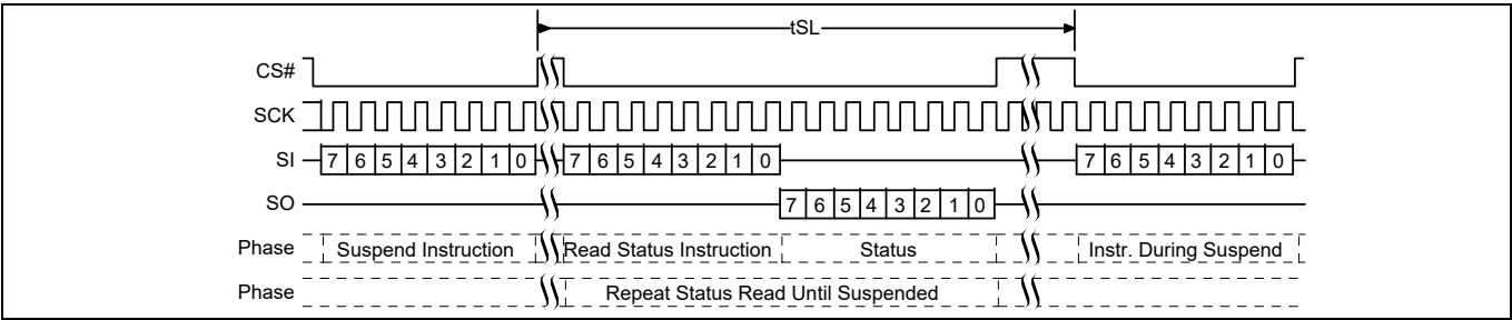
Figure 85 Program or Erase Suspend command sequence
