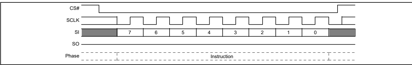
Figure 106 Deep Power-down command sequence
