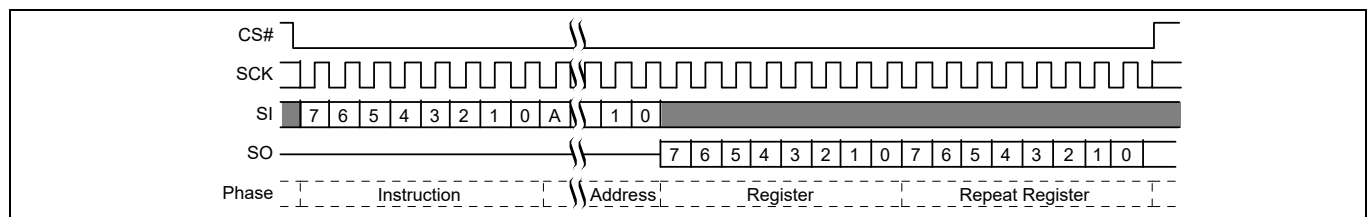
Figure 95 PPBRD command sequence [61, 62]
