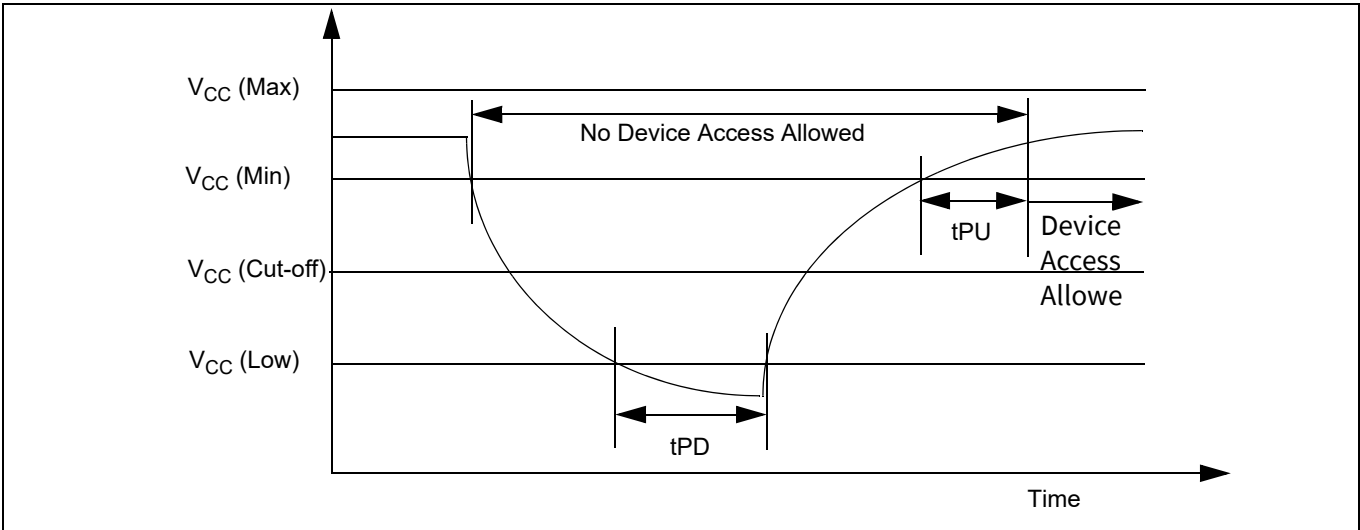
Figure 19 Power-down and voltage drop
