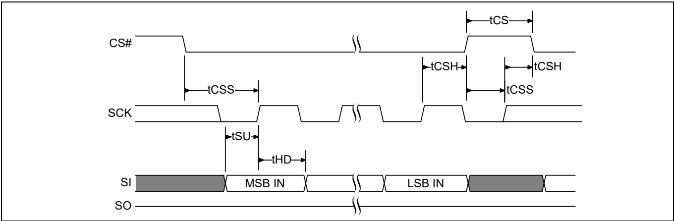
Figure 29 SPI single bit input timing
