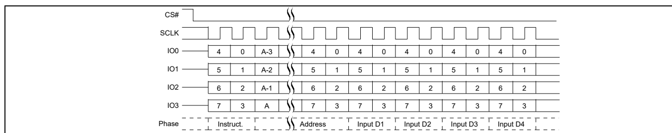
Figure 76 Page Program (PP 02h or 4PP 12h) QPI mode command sequence [52]
