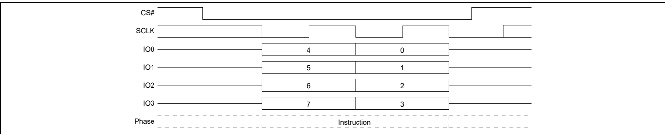
Figure 107 DPD command sequence QPI mode
