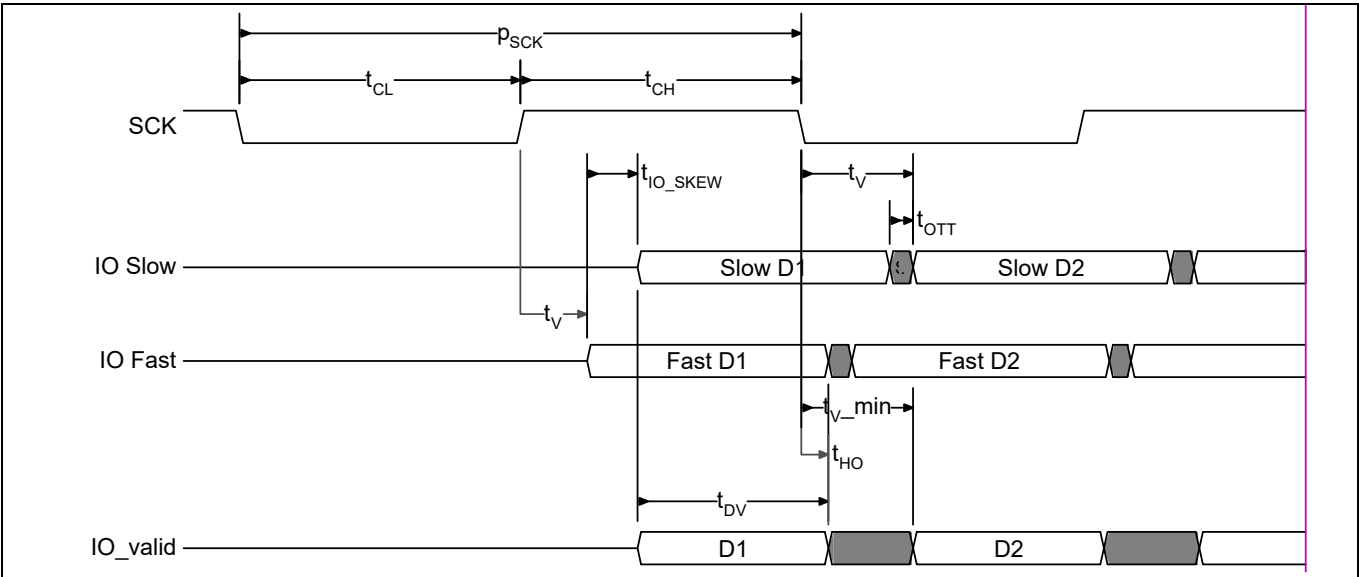
Figure 35 SPI DDR data valid window
