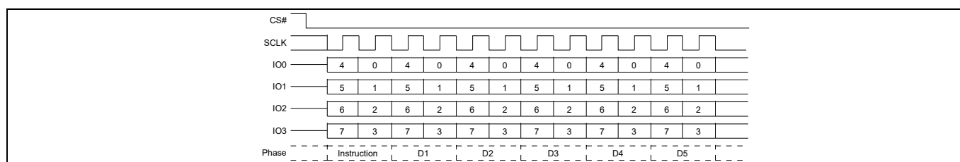
Figure 45 Read Quad Identification (RDQID) command sequence
