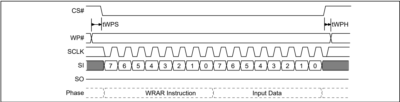
Figure 32 WP# input timing
