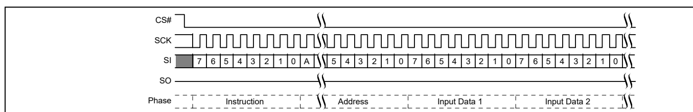
Figure 75 Page Program (PP 02h or 4PP 12h) command sequence [51]
