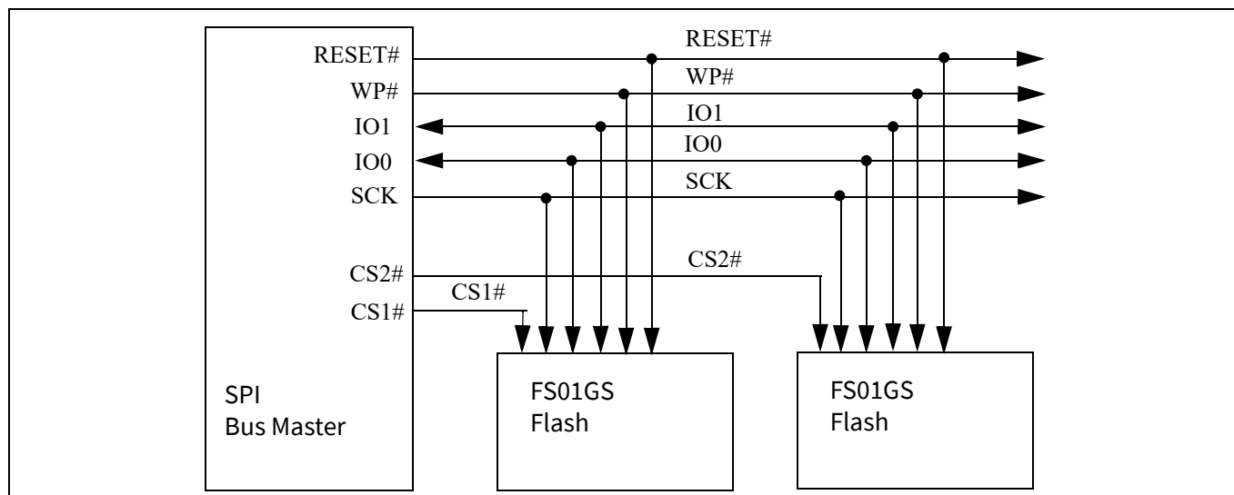
Figure 2 Bus master and memory devices on the SPI bus - Dual bit data path
