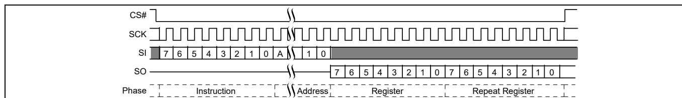
Figure 91 DYBRD command sequence [57, 58]
