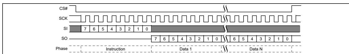
Figure 100 Password Read command sequence
