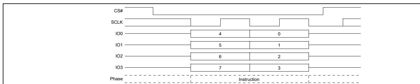
Figure 49 Write Enable (WREN) command sequence QPI mode
