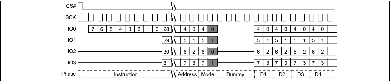
Figure 70 Quad I/O Read command sequence (4-byte address, ECh or EBh [CR2V[7] = 1])
