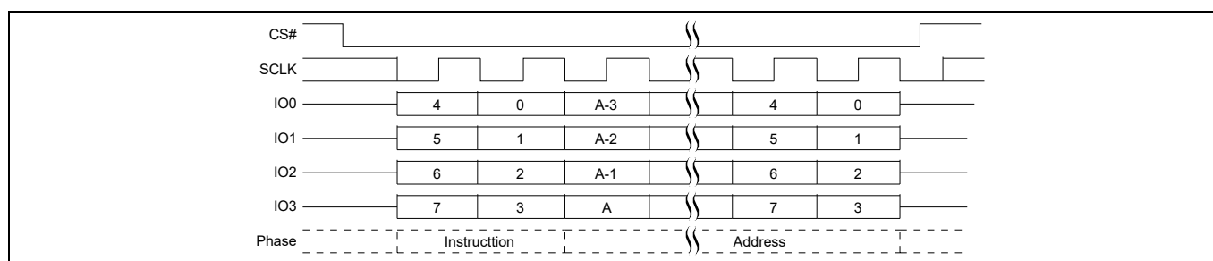
Figure 84 EES QPI mode command sequence [56]
