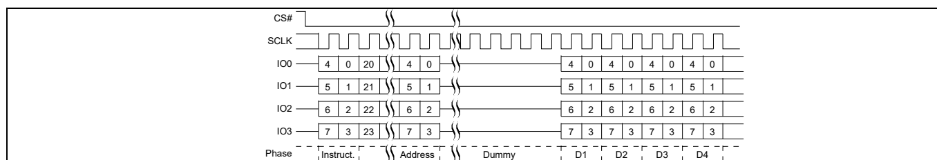
Figure 47 RSFDP QPI mode command sequence
