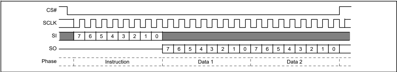
Figure 8 Single Bit Wide Output command
