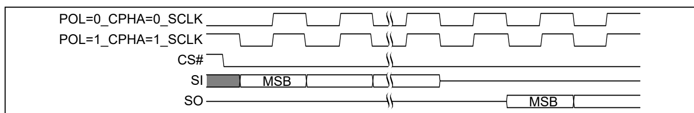
Figure 4 SPI SDR modes supported
