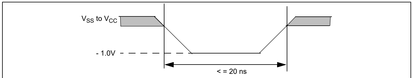
Figure 16 Maximum negative overshoot waveform
