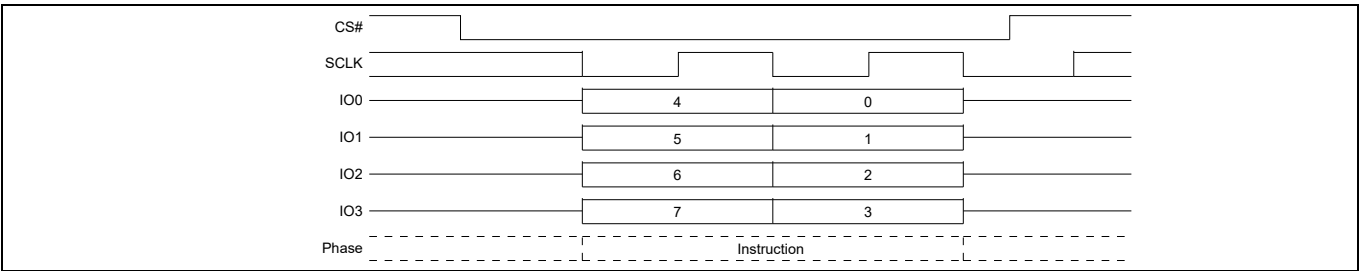
Figure 87 Erase or Program Suspend command sequence QPI mode
