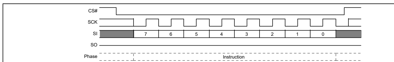
Figure 50 Write Disable (WRDI) command sequence
