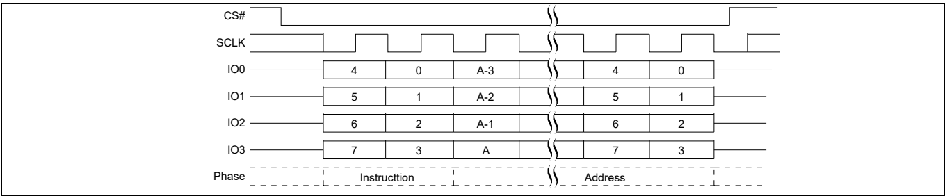
Figure 78 Parameter Sector Erase (P4E 20h or 4P4E 21h) QPI mode command sequence [53]
