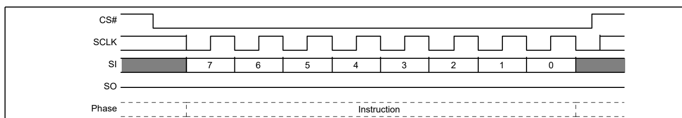
Figure 6 Standalone Instruction command
