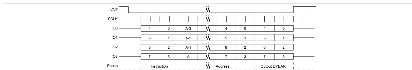
Figure 92 DYBRD QPI mode command sequence [57, 58]
