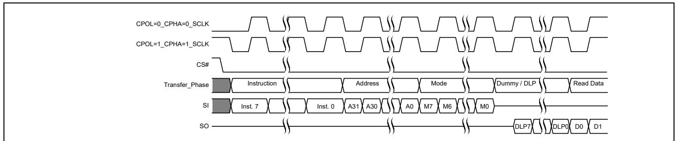
Figure 5 SPI DDR modes supported
