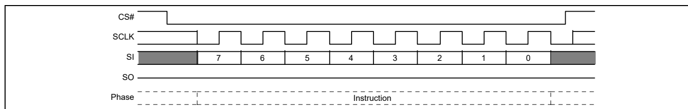
Figure 108 Release from Deep Power-down command sequence
