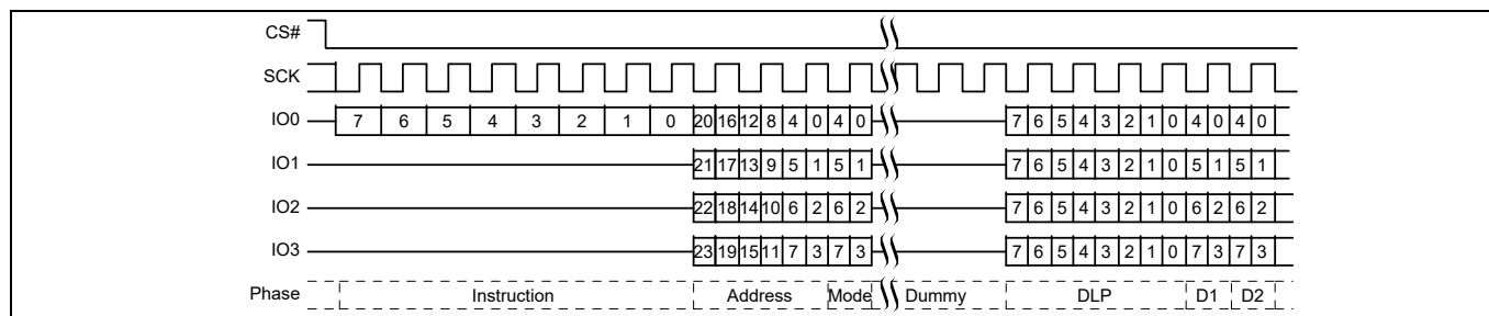
Figure 72 DDR Quad I/O Read initial access (3-byte address, EDh [CR2V[7] = 0])
