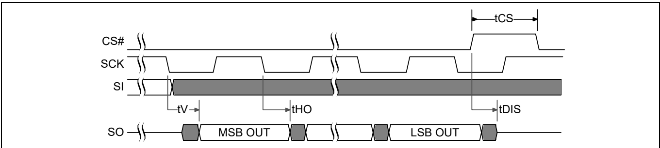
Figure 30 SPI single bit output timing
