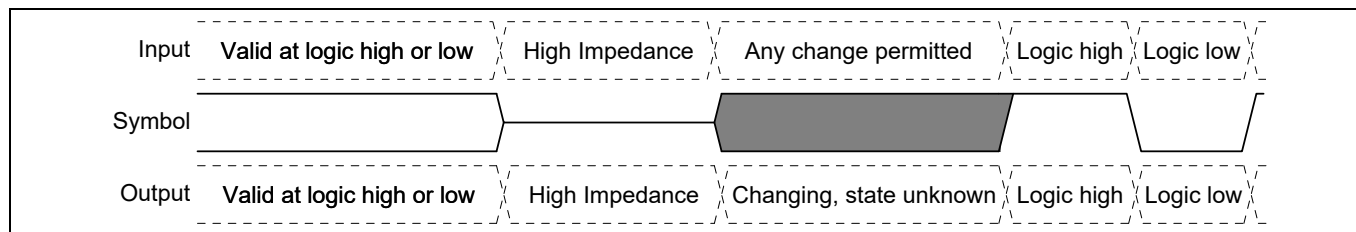
Figure 20 Waveform element meanings
