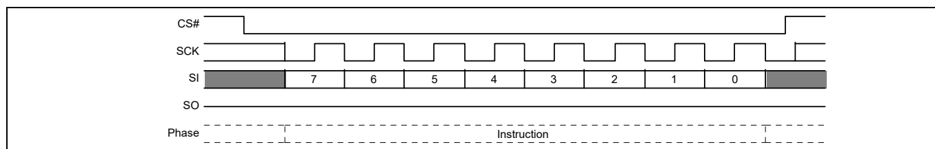
Figure 48 Write Enable (WREN) command sequence
