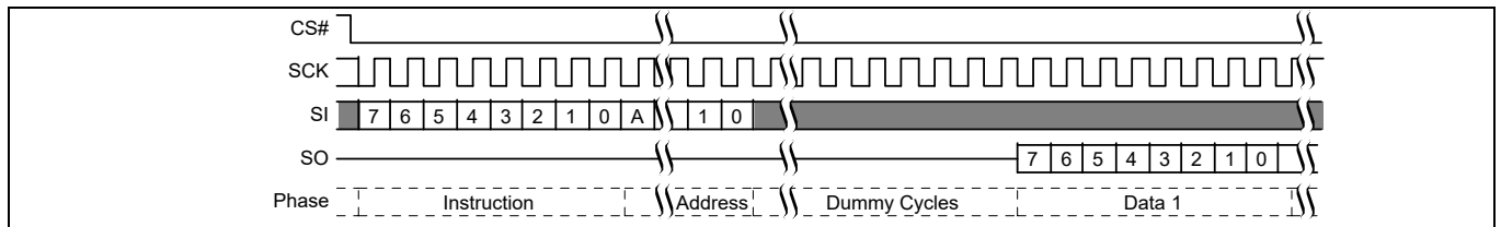
Figure 54 ECC Status Register Read command sequence [43, 44]
