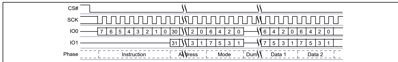
Figure 67 Dual I/O Read command sequence (4-byte address, BBh [CR2V[7] = 1])
