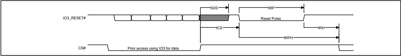
Figure 27 Hardware Reset when Quad mode and IO3 / Reset# are enabled
