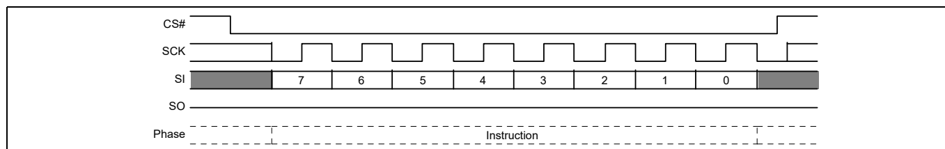
Figure 99 PPB Lock Bit Write command sequence
