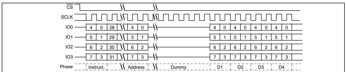
Figure 56 ECCRD (19h), Quad All Mode, CR2[7] = 1, or 4EECRD (18h) command sequence
