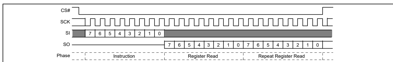
Figure 98 PPB Lock Register Read command sequence
