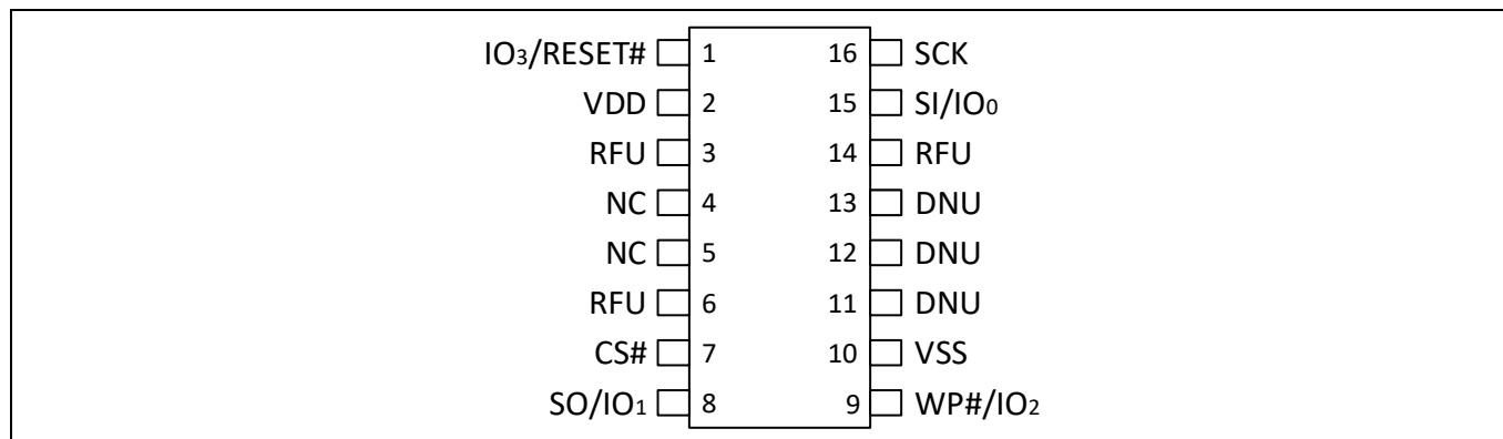
Figure 36 16-lead SOIC package, Top view [34]
