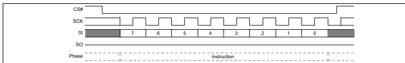
Figure 59 Enter 4 Byte Address Mode (4BAM B7h) command sequence
