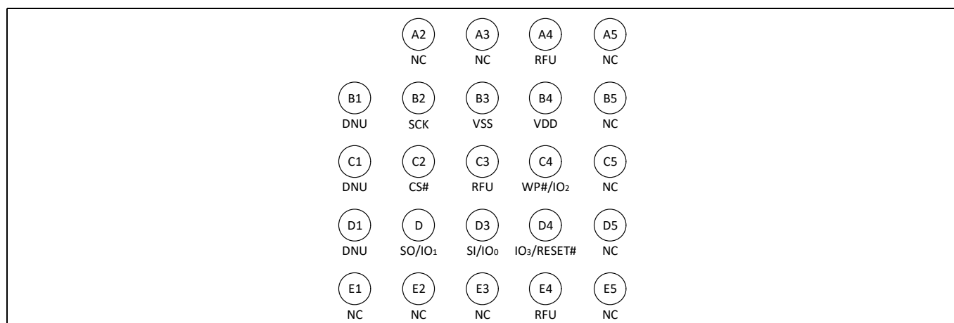
Figure 37 24-ball BGA, 5x5 ball footprint (ZSA024), Top view [35, 36]
