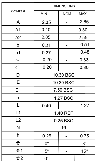
Figure 40 SOIC 16-lead, 300-mil body width (S03016)
