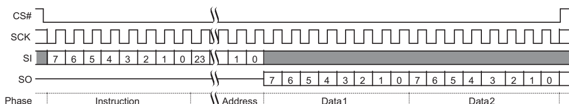
Figure 45. Read Data Command Sequence
