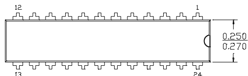
24-Lead (300-Mil) PDIP P13
