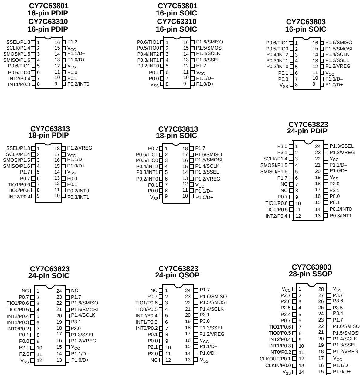
Figure 5-1. Package Configurations
