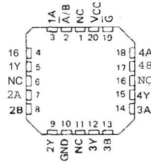
SN54157, SN54S157, SN54LS158, SN54S158 ... FK PACKAGE (TOP VIEW)
