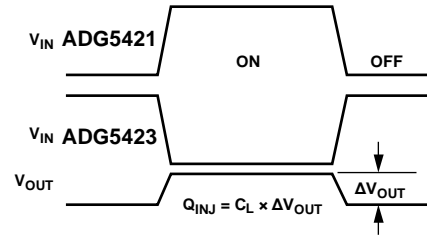
Figure 31. Charge Injection
