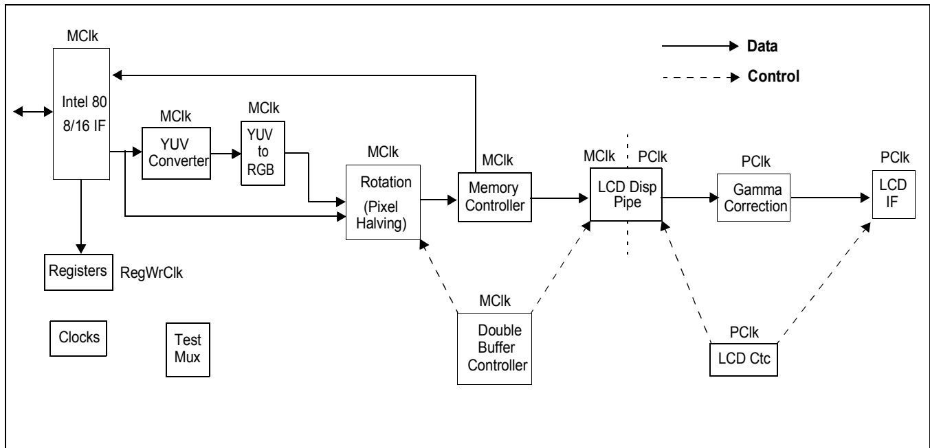
Figure 3-1: Block Diagram
