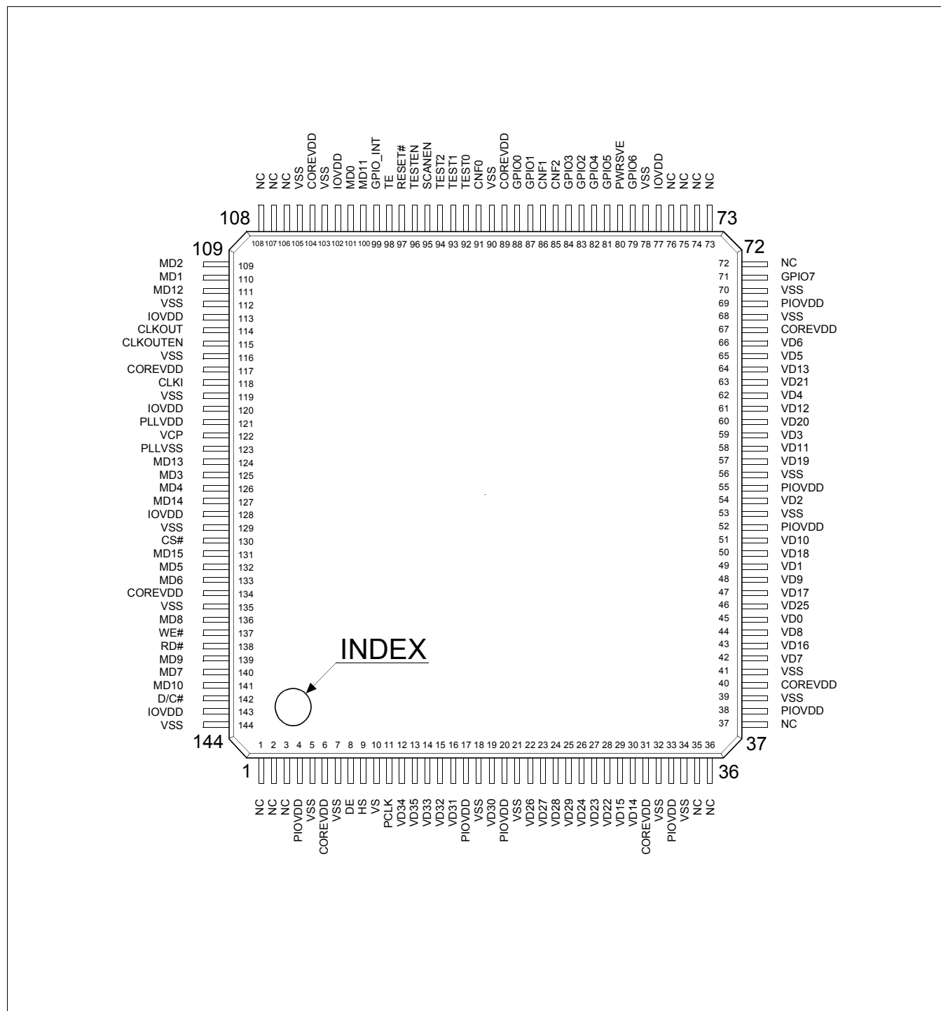
Figure 4-1: S1D13742 QFP20 Pinout (Top View)
