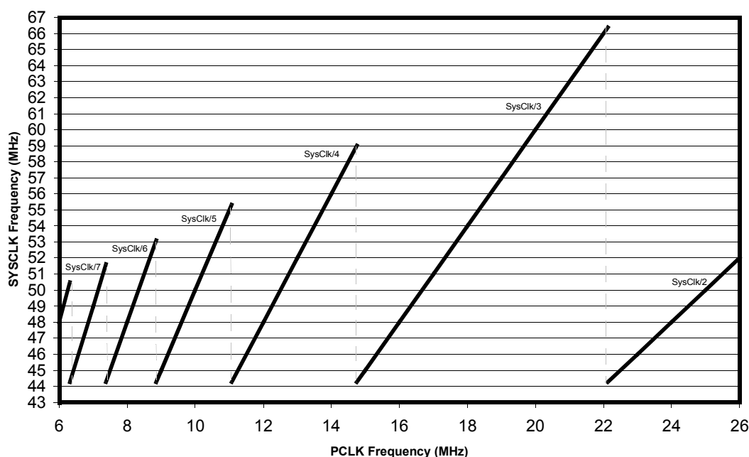
Figure 8-3: Setting of SYSCLK For a Desired PCLK
