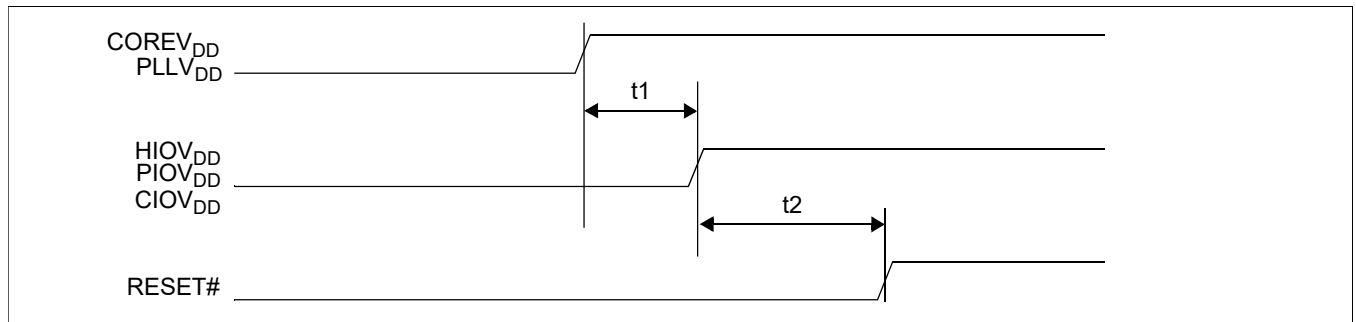
Figure 7-4: Power-On Sequence
