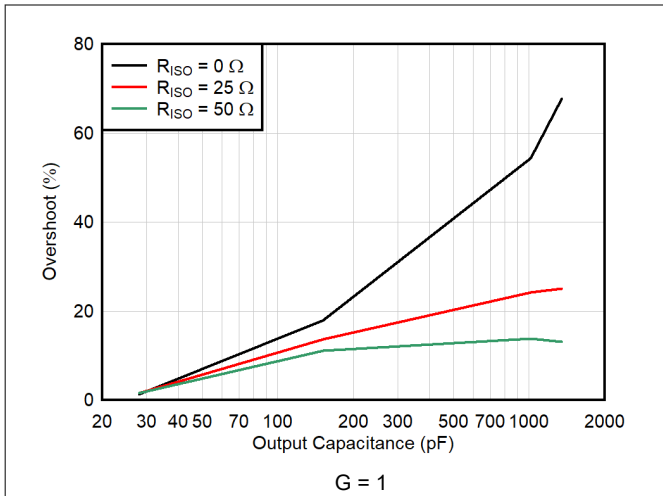
Figure 6-31. Small-Signal Overshoot vs Capacitive Load (10-mV Step)
