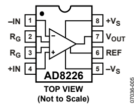
Figure 60. Pinout Diagram
