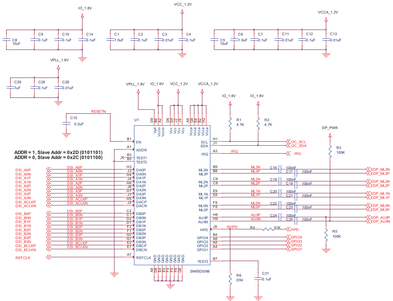
Figure 9-1. Typical Implementation
