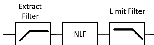
Figure 13. Treble Enhancement
