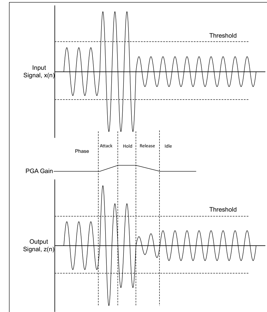
Figure 17. ALC Operation
