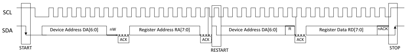
Figure 27. Read Cycle
