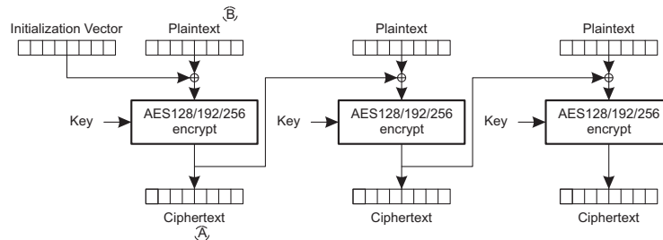
Figure 14-8. CBC Encryption
