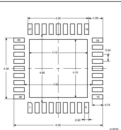
Figure 35. Recommended footprint (dimensions in mm) (1)(2)(3)
