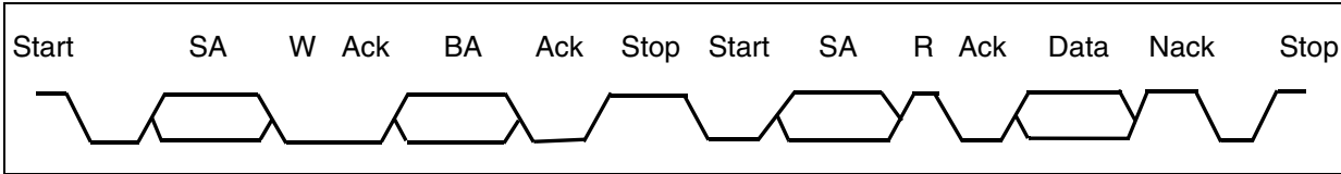
Figure 78. Sequential Read
