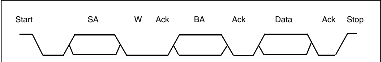
Figure 74. Page Write
