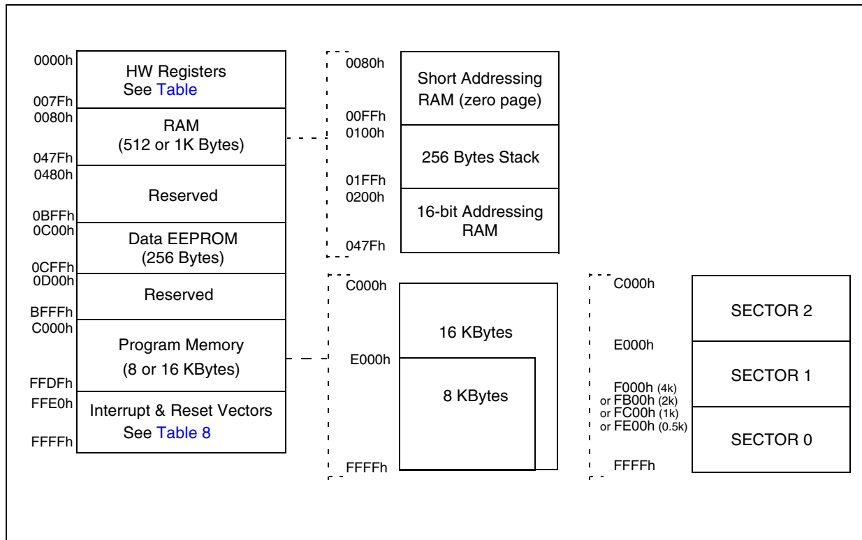
Figure 5. Memory Map
