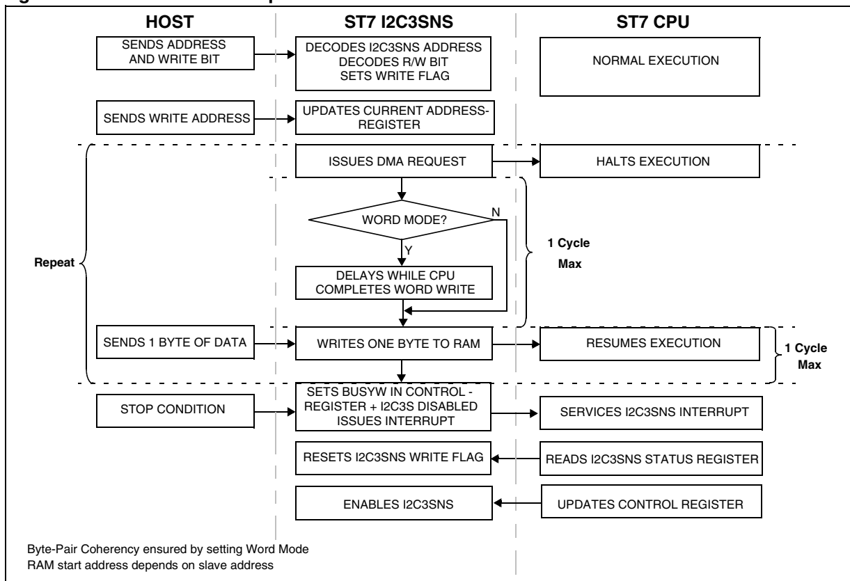
Figure 70. 16-bit Word Write Operation Flowchart
