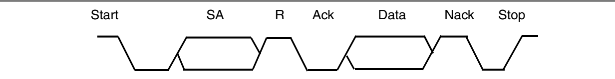
Figure 76. Random Read (Dummy write + restart + current address read)
