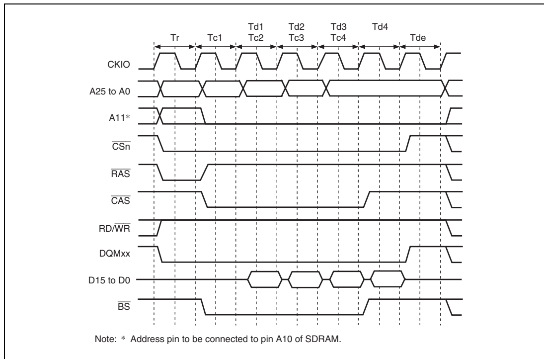
Figure 7.17 Burst Read Timing (No Auto Precharge)
