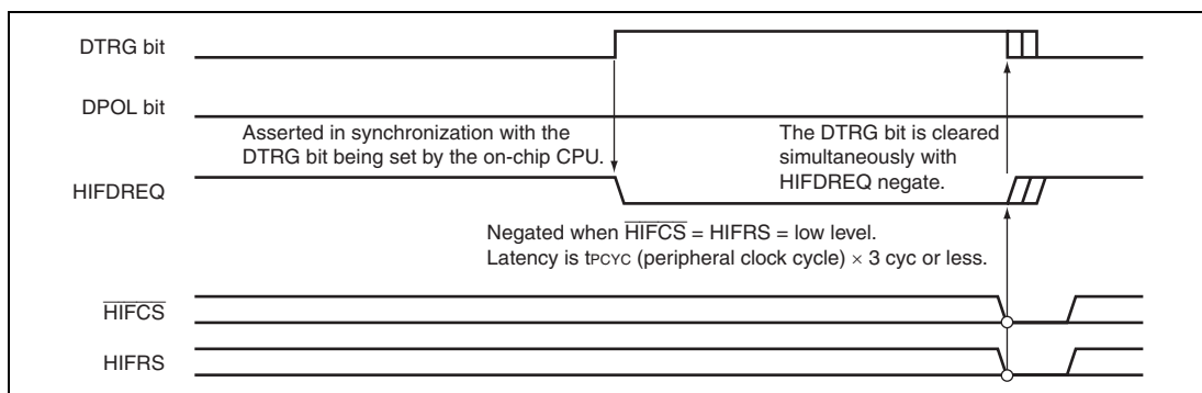
Figure 15.8 HIFDREQ Timing (When DMD = 0 and DPOL = 0)
