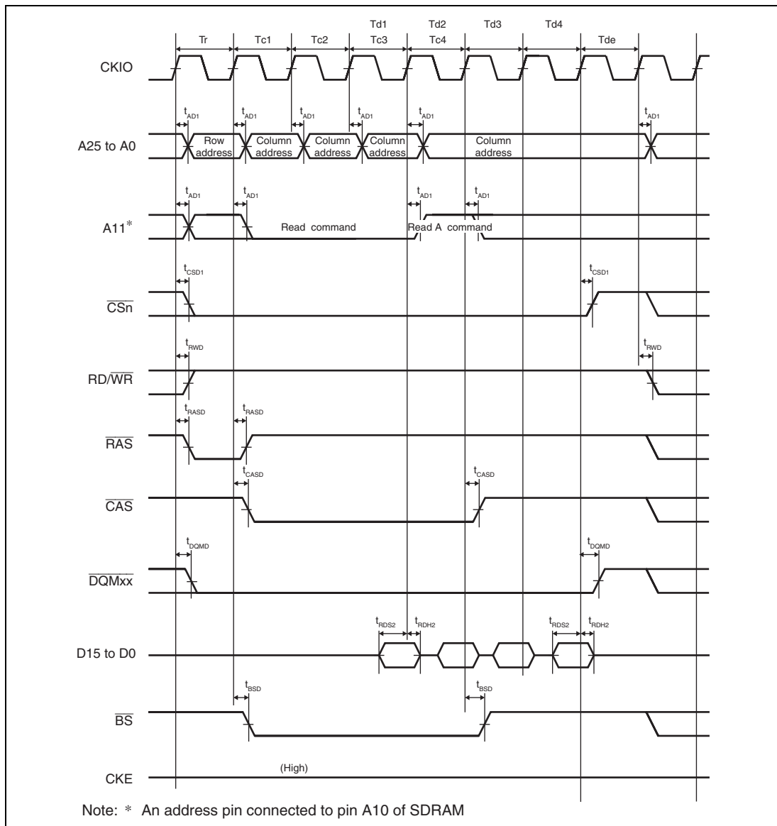
Figure 21.18 Synchronous DRAM Burst Read Bus Cycle (Single Read × 4) (Auto-Precharge, CAS Latency = 2, WTRCD = 0 Cycle, WTRP = 1 Cycle)
