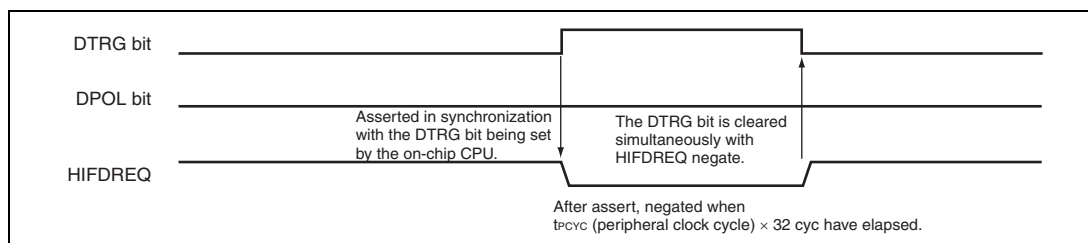
Figure 15.10 HIFDREQ Timing (When DMD = 1 and DPOL = 0)
