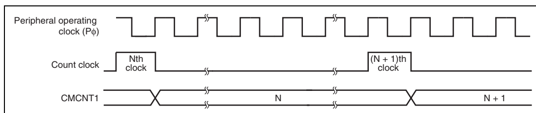
Figure 13.3 Count Timing
