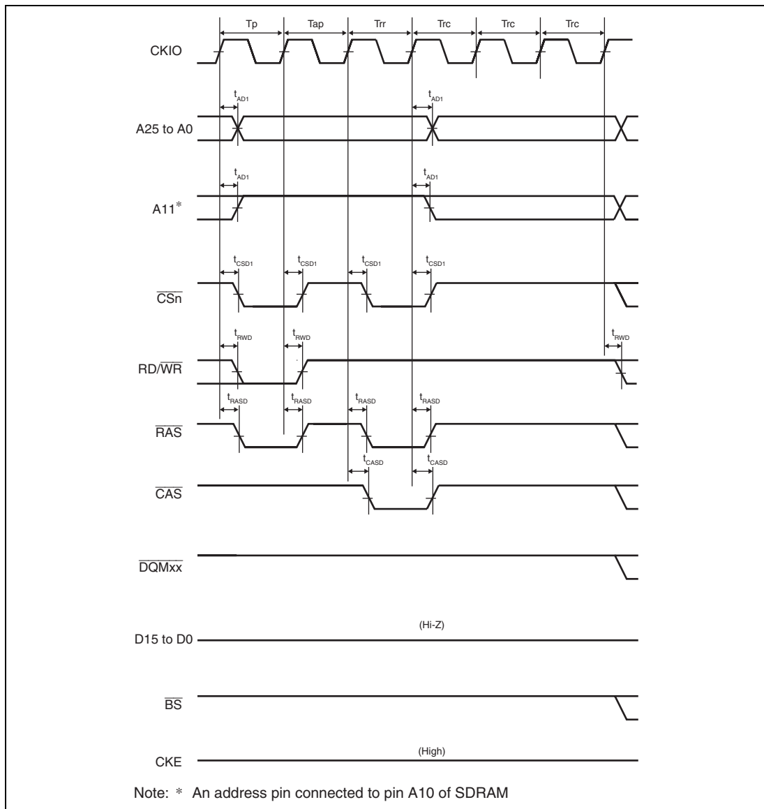
Figure 21.30 Synchronous DRAM Auto-Refreshing Timing (WTRP = 1 Cycle, WTRC = 3 Cycles)
