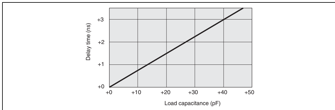
Figure 21.55 Load Capacitance versus Delay Time
