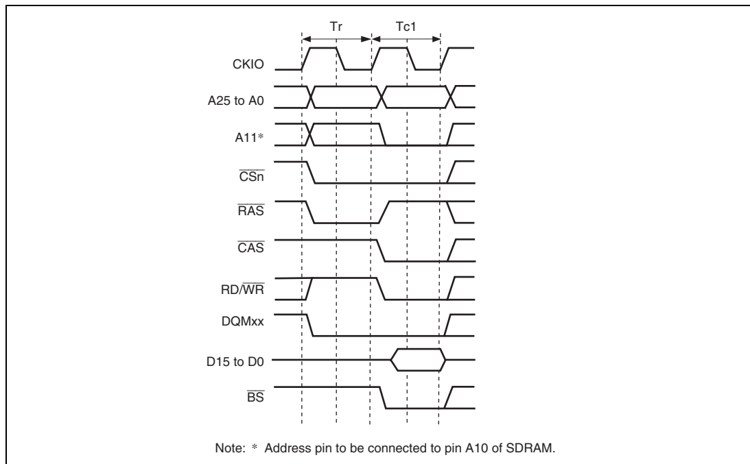
Figure 7.20 Single Write Timing (No Auto Precharge)
