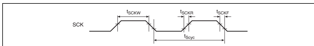
Figure 21.37 SCK Input Clock Timing
