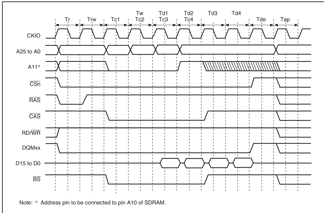
Figure 7.13 Burst Read Wait Specification Timing (Auto Precharge)
