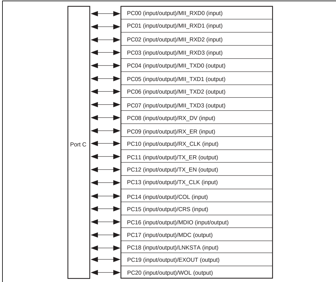
Figure 17.3 Port C
