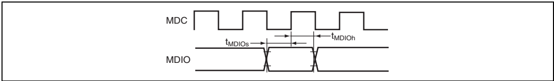
Figure 21.47 MDIO Input Timing
