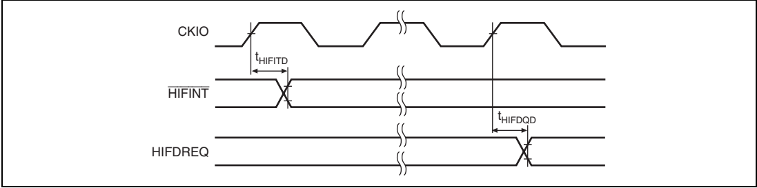
Figure 21.41 \overline{\text{HIFINT}} and HIFDREQ Timing
