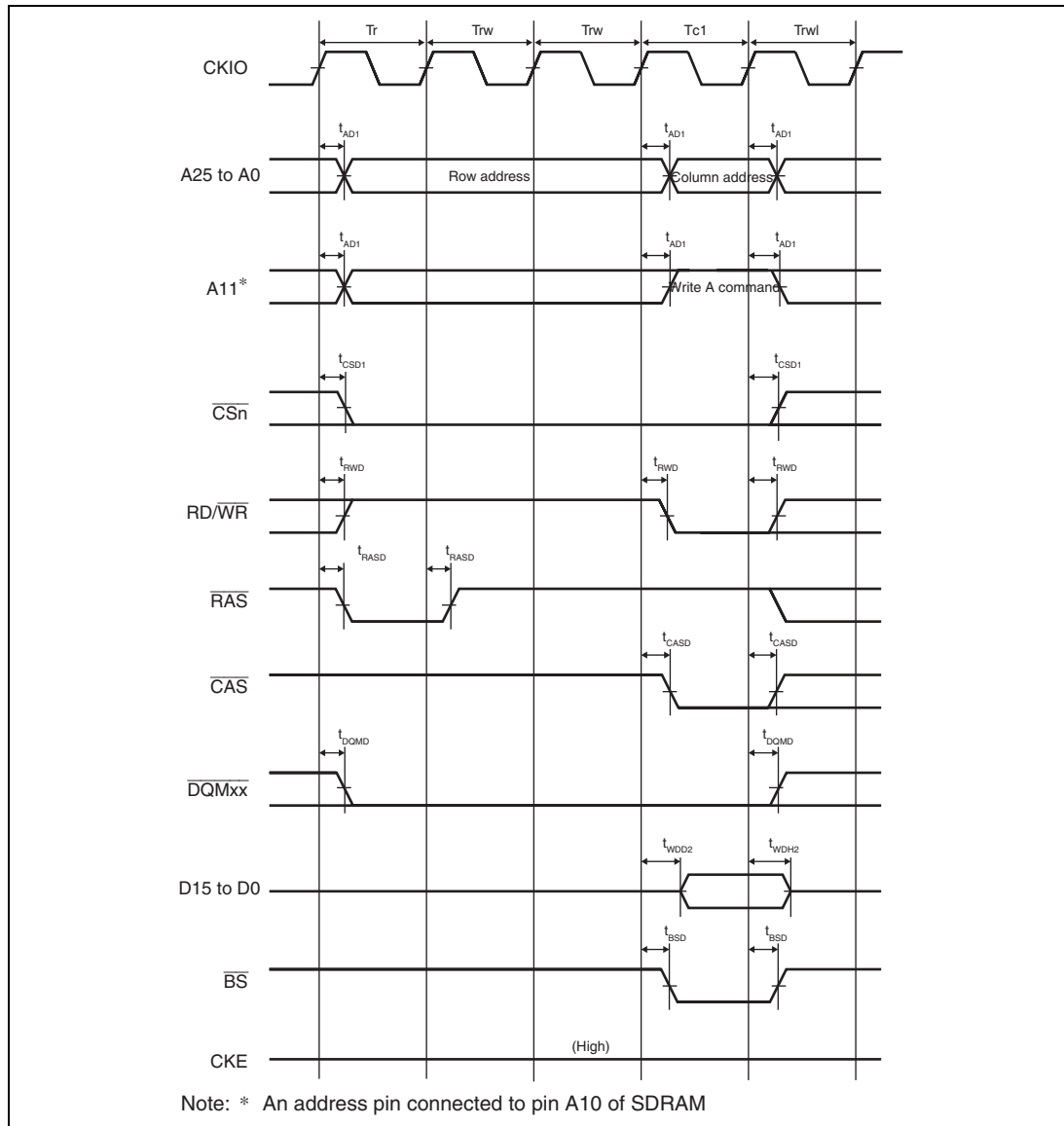
Figure 21.21 Synchronous DRAM Single Write Bus Cycle (Auto-Precharge, WTRCD = 2 Cycles, TRWL = 1 Cycle)
