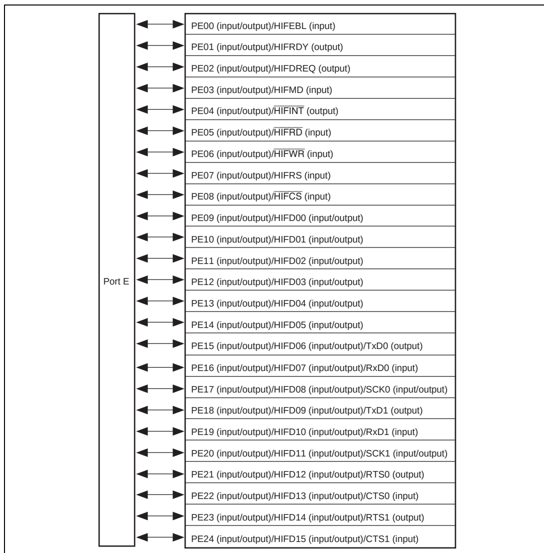
Figure 17.5 Port E
