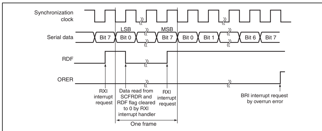
Figure 14.17 Example of SCIF Receive Operation
