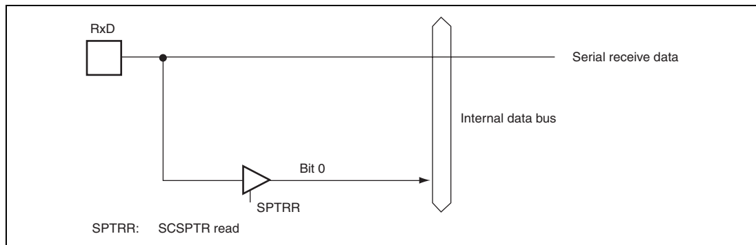
Figure 14.23 SPBDT bit and RxD Pin
