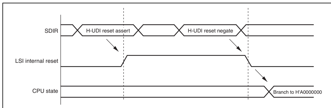
Figure 19.4 H-UDI Reset
