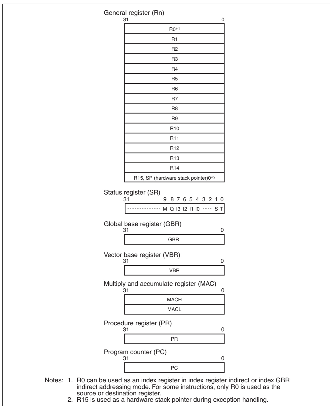
Figure 2.1 CPU Internal Register Configuration
