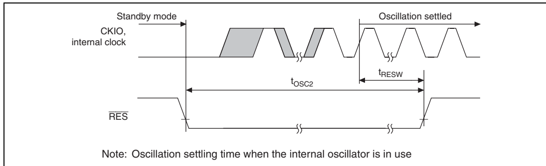
Figure 21.4 Oscillation Settling Timing after Standby Mode (By Reset)
