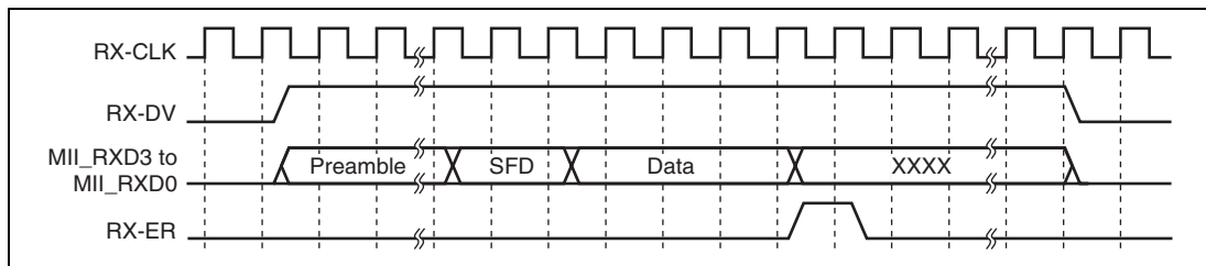
Figure 11.4 (5) MII Frame Receive Timing (Reception Error (1))
