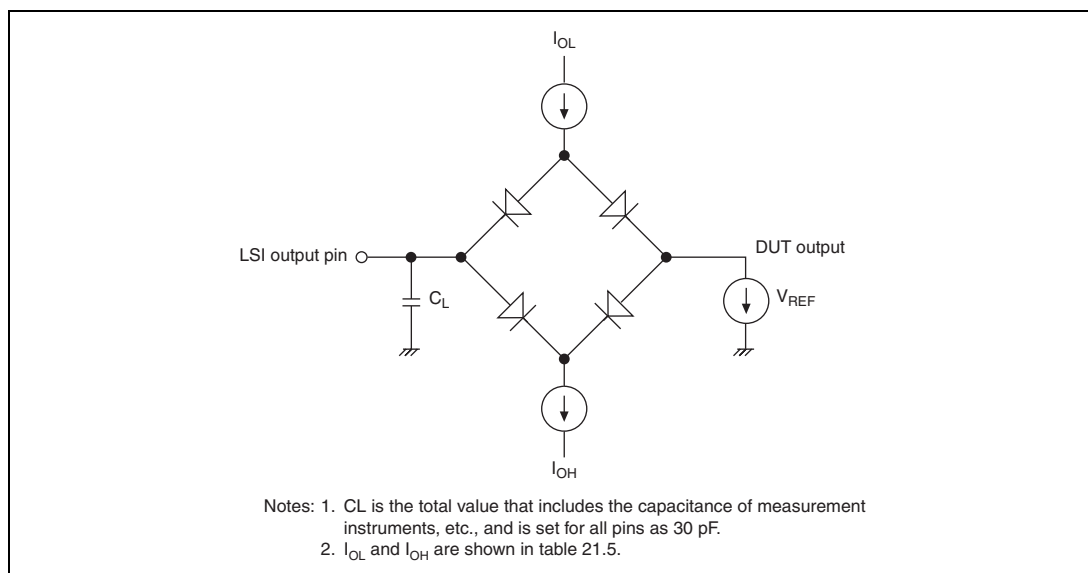
Figure 21.54 Output Load Circuit
