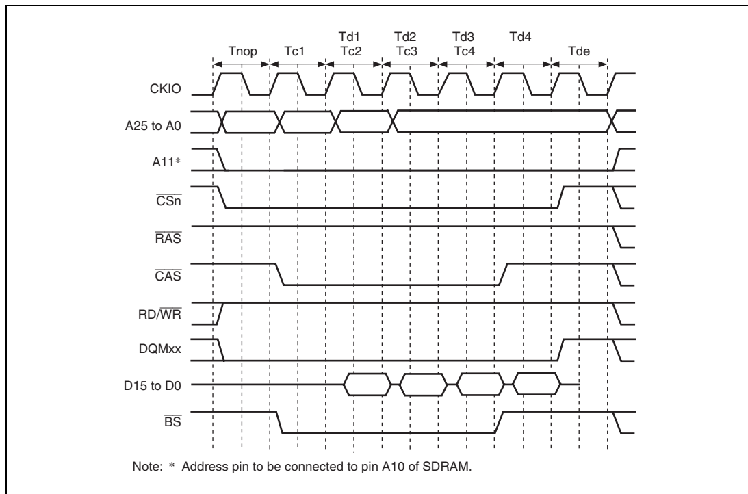
Figure 7.18 Burst Read Timing (Bank Active, Same Row Address)
