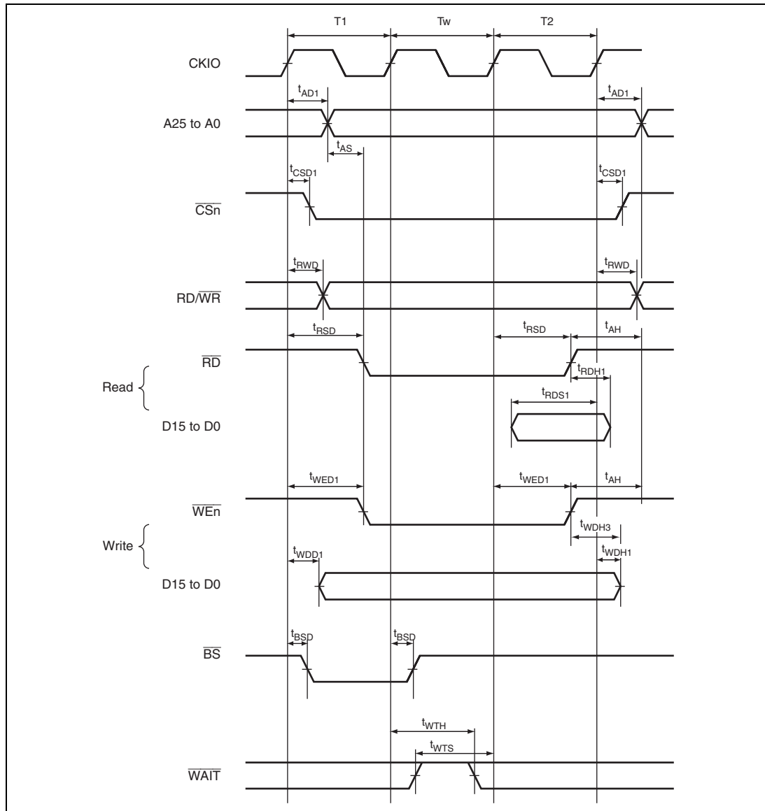
Figure 21.11 Basic Bus Timing: One Software Wait Cycle
