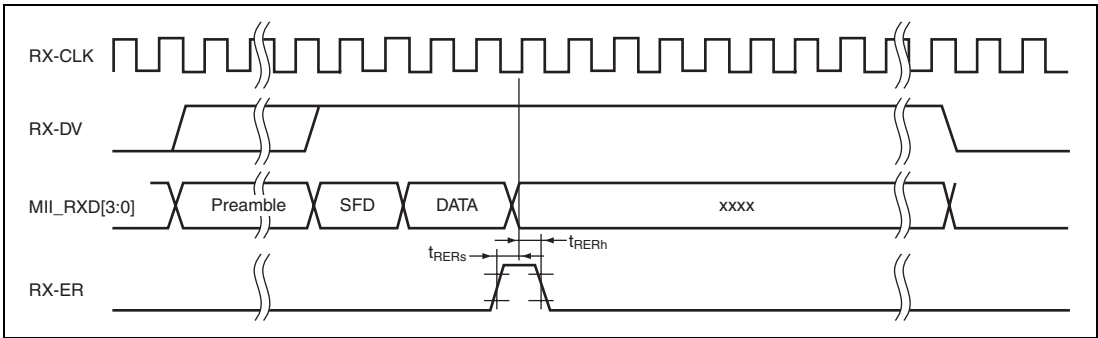
Figure 21.46 MII Reception Timing (Error Occurred)
