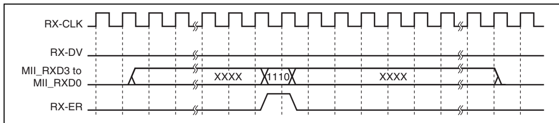
Figure 11.4 (6) MII Frame Receive Timing (Reception Error (2))
