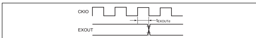
Figure 21.50 EXOUT Output Timing
