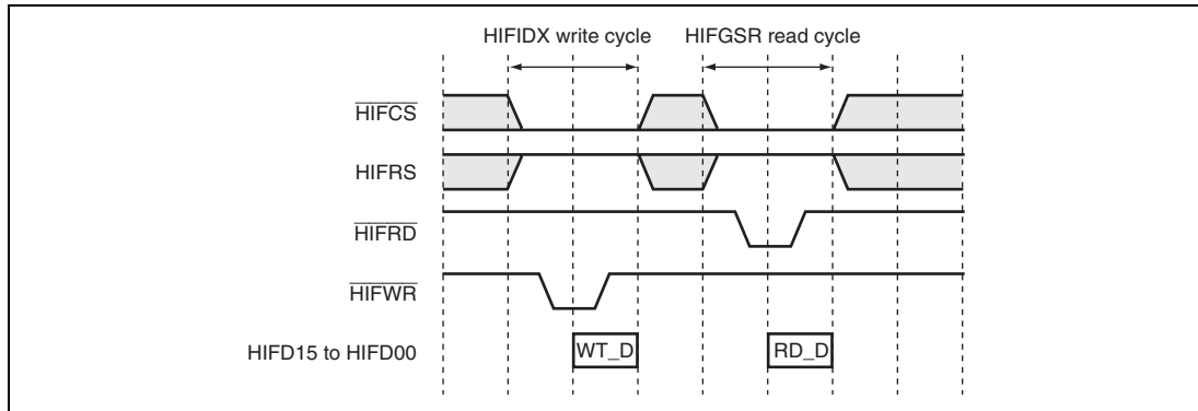
Figure 15.4 HIFIDX Write and HIFGSR Read
