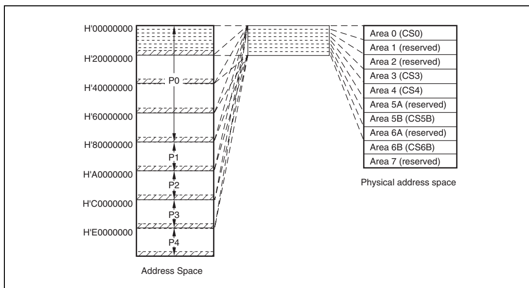
Figure 7.2 Address Space
