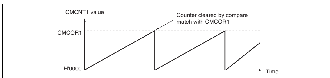
Figure 13.2 Counter Operation
