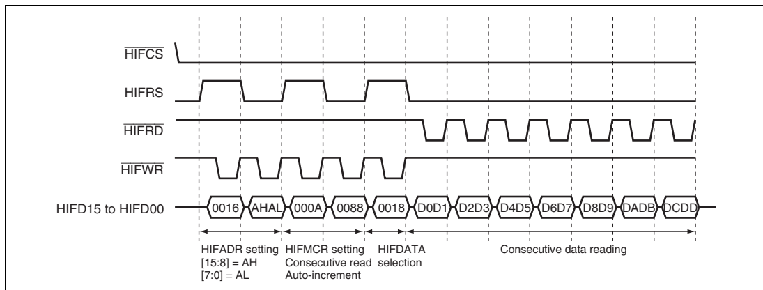
Figure 15.7 Consecutive Data Reading from HIFRAM
