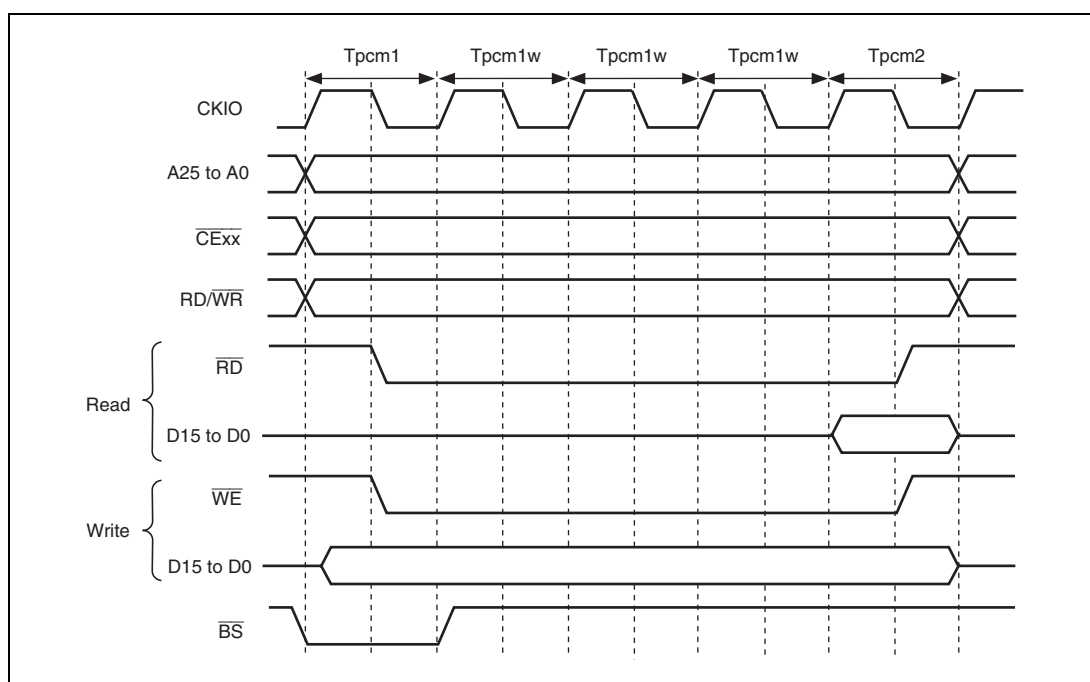
Figure 7.31 Basic Access Timing for PCMCIA Memory Card Interface
