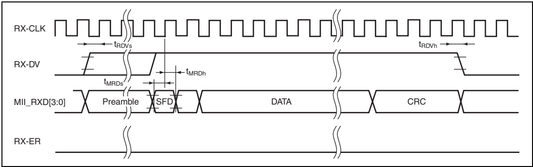
Figure 21.45 MII Reception Timing (Normal Operation)
