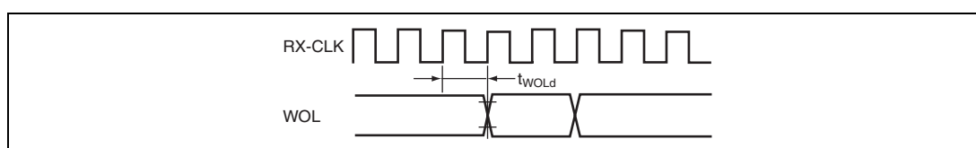
Figure 21.49 WOL Output Timing
