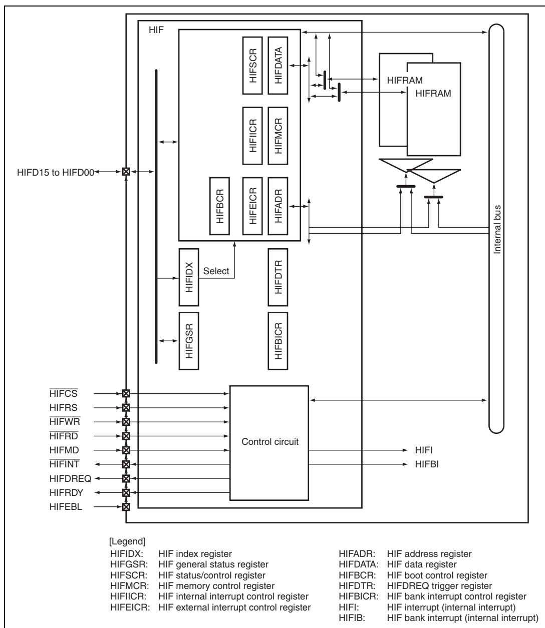
Figure 15.1 Block Diagram of HIF
