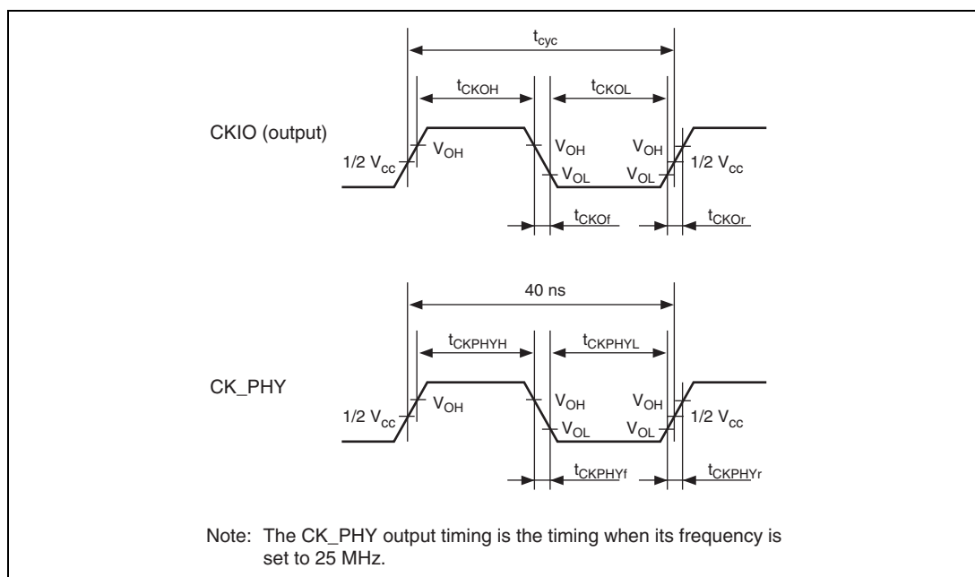
Figure 21.2 CKIO and CK_PHY Clock Output Timings
