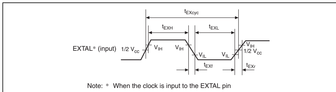
Figure 21.1 External Clock Input Timing
