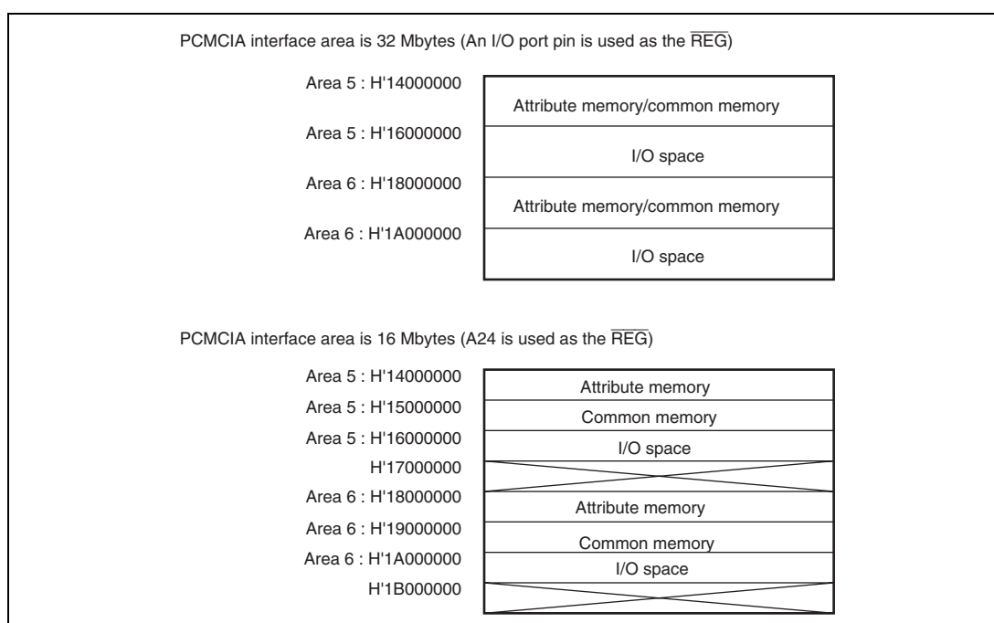
Figure 7.33 Example of PCMCIA Space Assignment (CS5BWCR.SA[1:0] = B'10, CS6BWCR.SA[1:0] = B'10)
