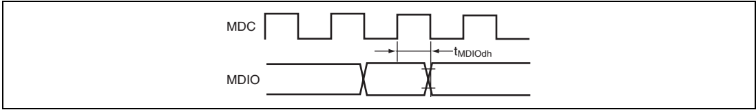
Figure 21.48 MDIO Output Timing
