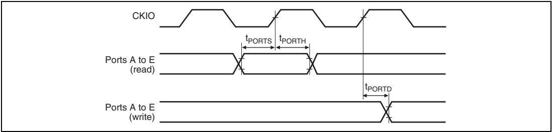
Figure 21.39 I/O Port Timing
