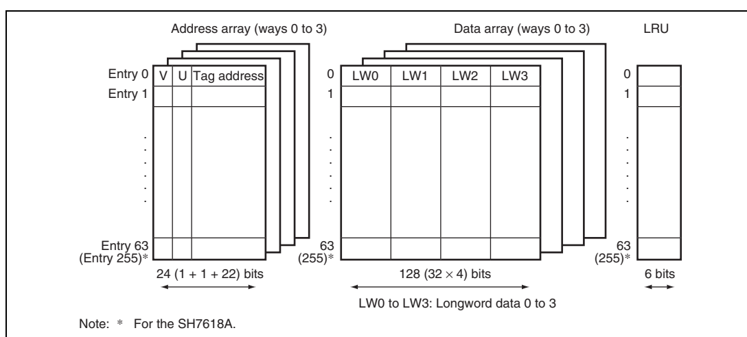
Figure 3.1 Cache Structure
