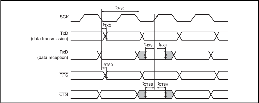
Figure 21.38 SCI Input/Output Timing in Clocked Synchronous Mode
