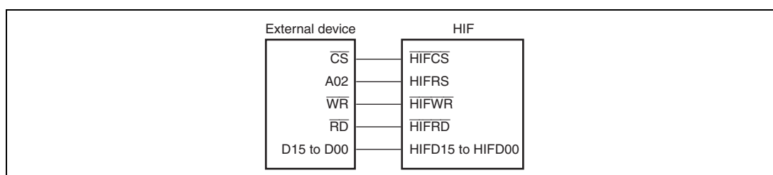
Figure 15.2 HIF Connection Example
