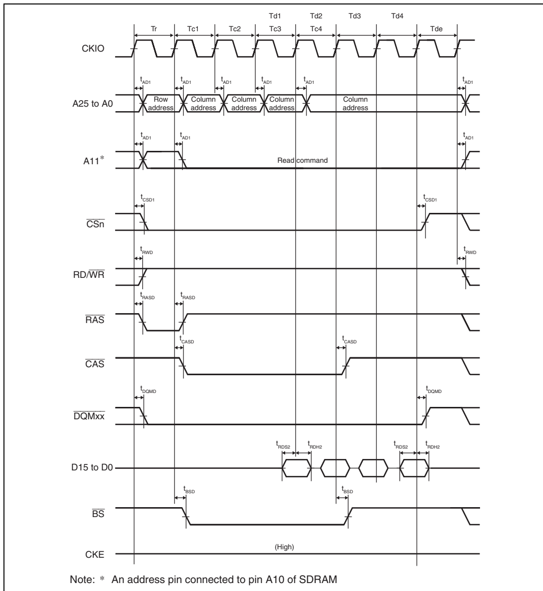
Figure 21.24 Synchronous DRAM Burst Read Bus Cycle (Single Read × 4) (Bank Active Mode: ACT + READ Commands, CAS Latency = 2, WTRCD = 0 Cycle)
