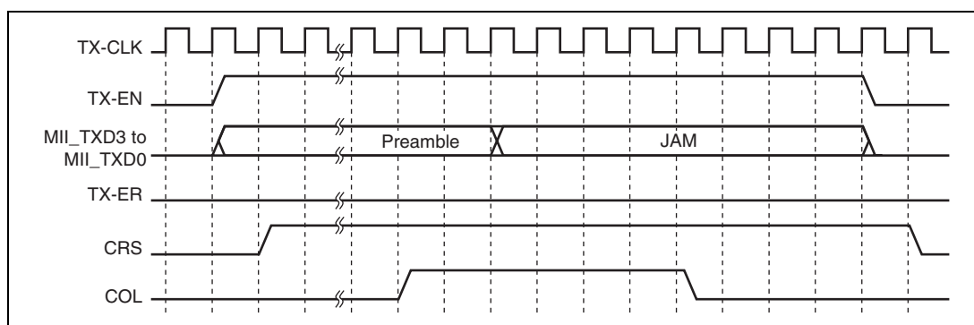
Figure 11.4 (2) MII Frame Transmit Timing (Collision)
