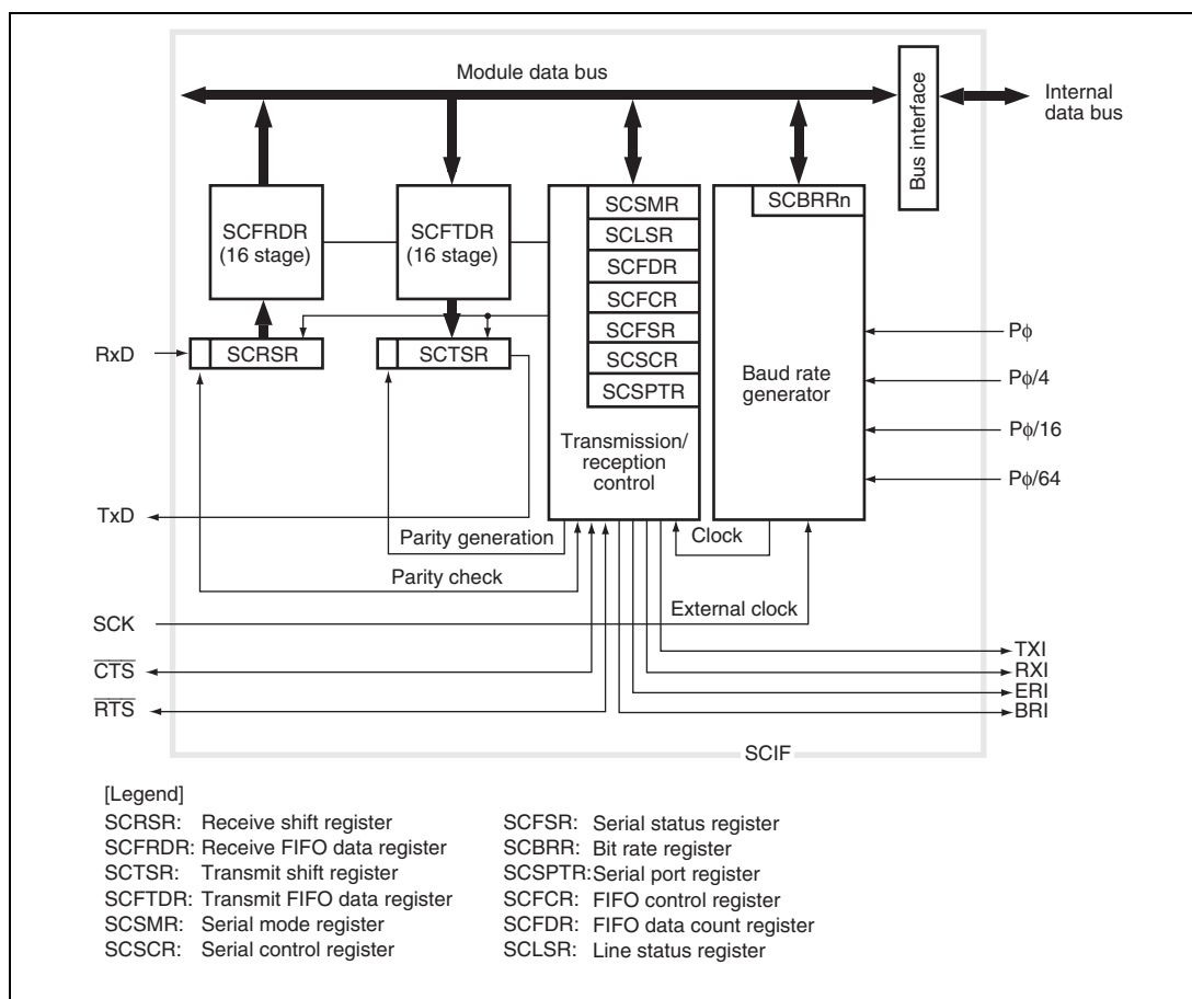
Figure 14.1 Block Diagram of SCIF
