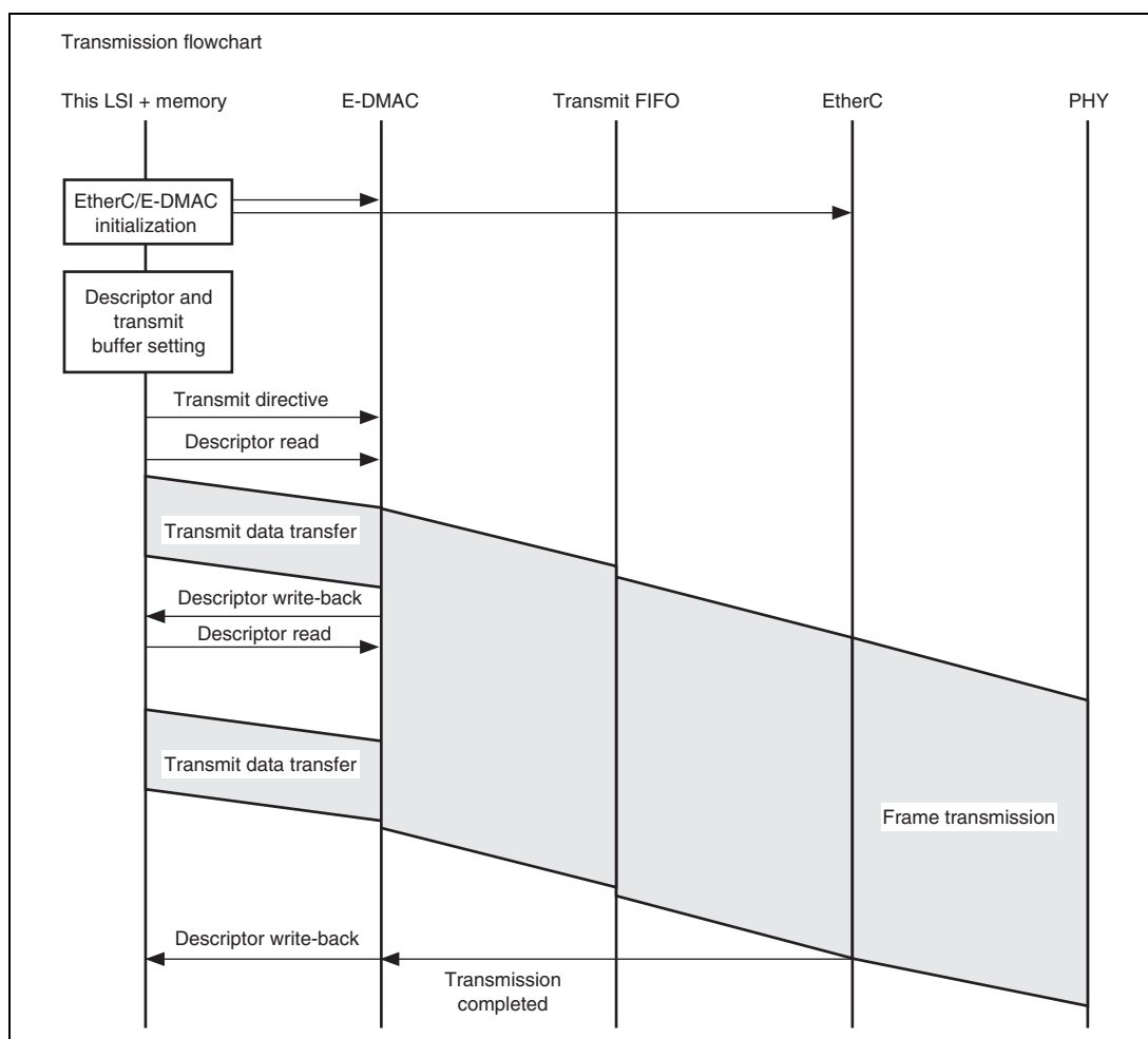
Figure 12.4 Sample Transmission Flowchart
