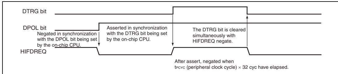
Figure 15.11 HIFDREQ Timing (When DMD = 1 and DPOL = 1)
