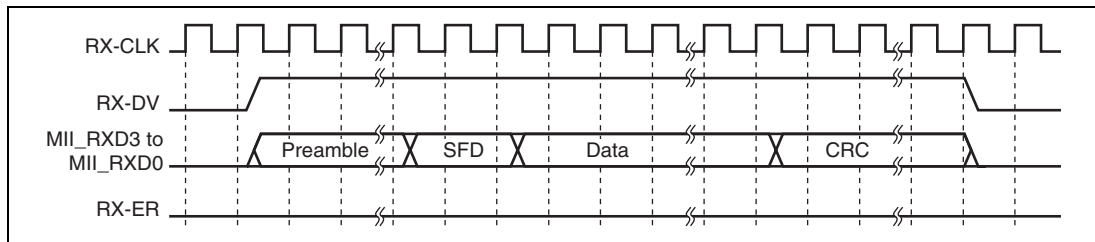
Figure 11.4 (4) MII Frame Receive Timing (Normal Reception)
