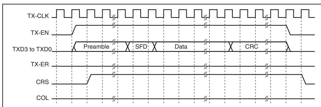
Figure 11.4 (1) MII Frame Transmit Timing (Normal Transmission)
