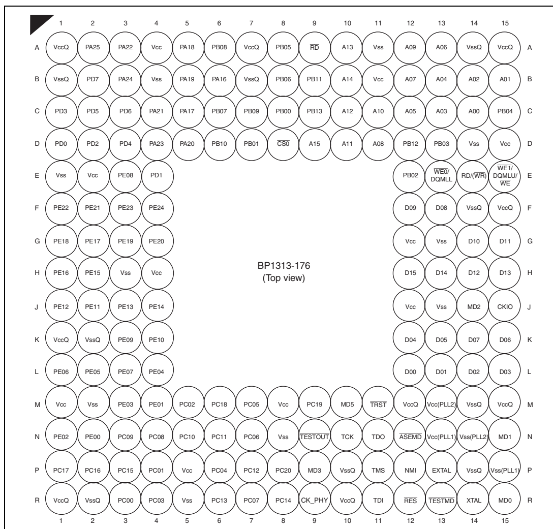
Figure 1.2 Pin Assignments
