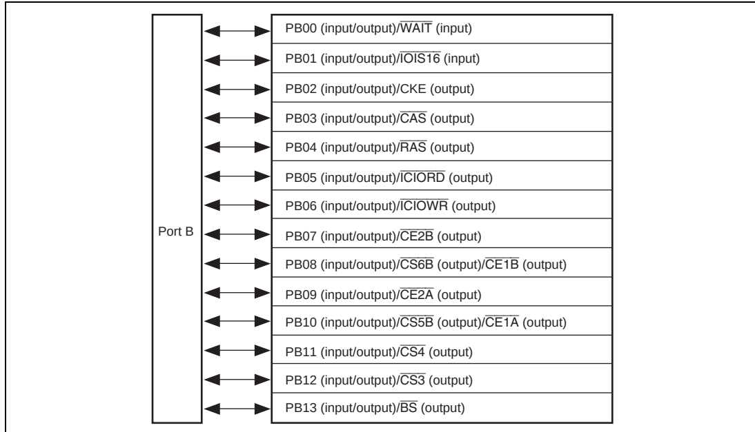
Figure 17.2 Port B
