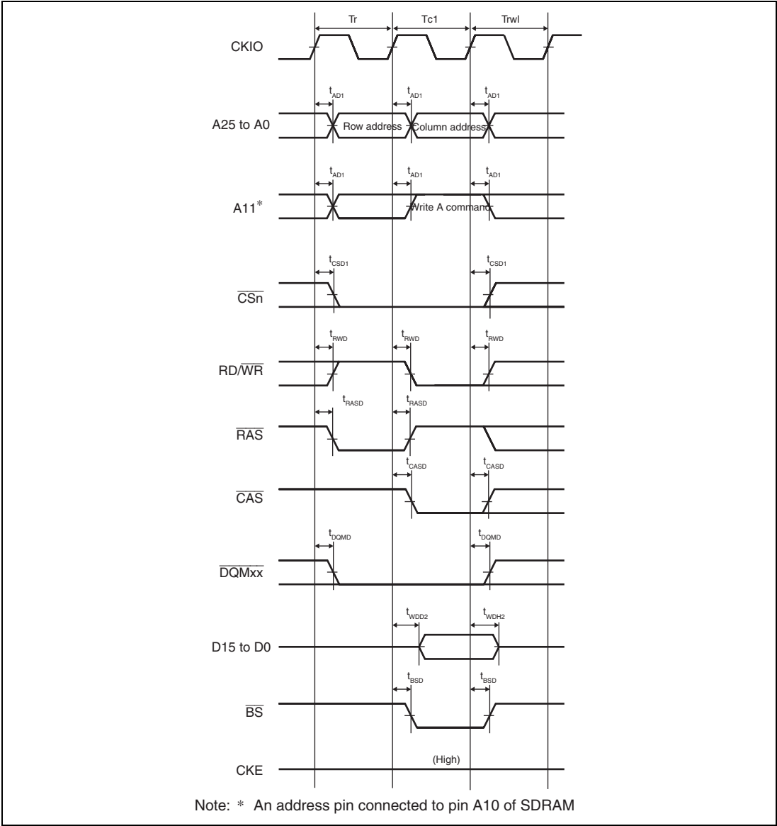
Figure 21.20 Synchronous DRAM Single Write Bus Cycle (Auto-Precharge, TRWL = 1 Cycle)
