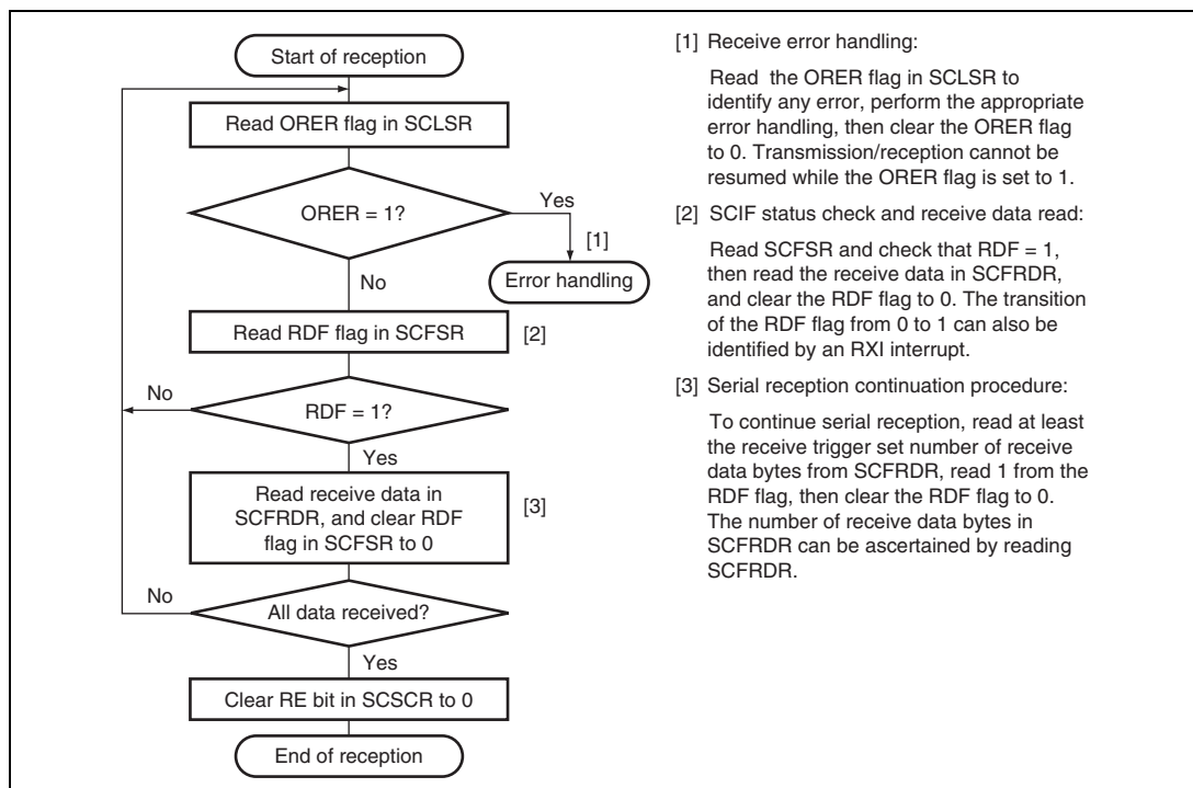
Figure 14.15 Sample Flowchart for Receiving Serial Data (1)
