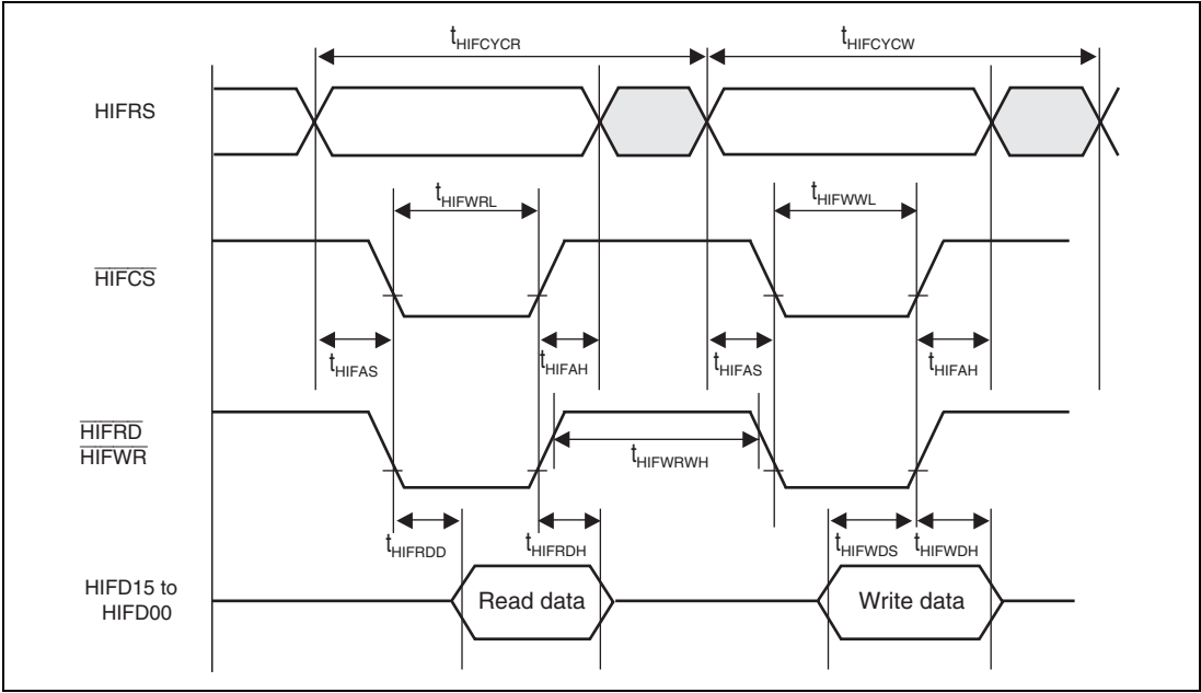
Figure 21.40 HIF Access Timing
