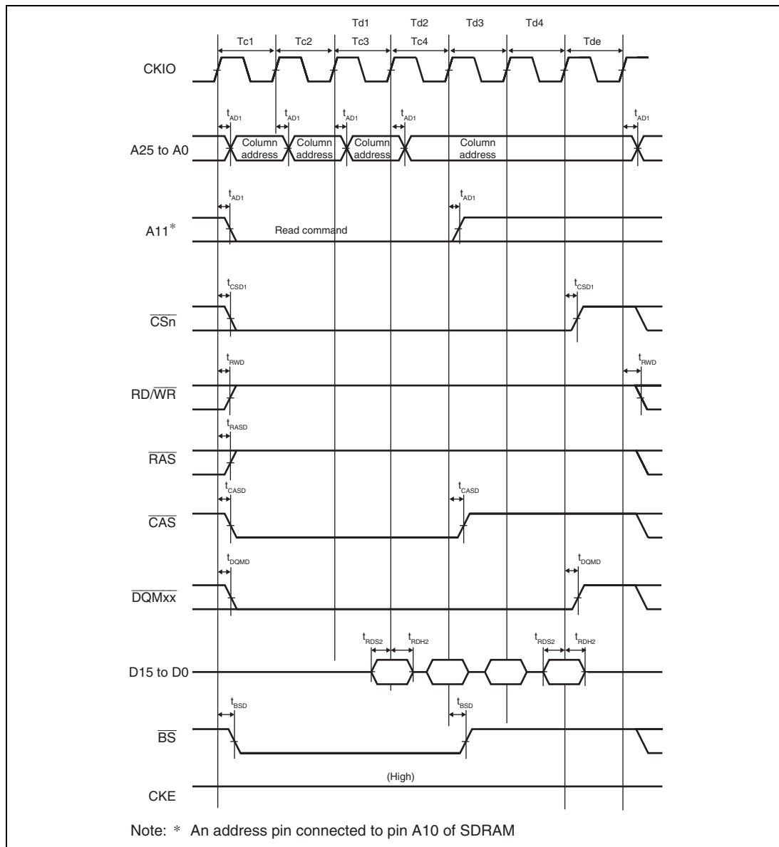
Figure 21.25 Synchronous DRAM Burst Read Bus Cycle (Single Read \times 4 ) (Bank Active Mode: READ Command, Same Row Address, CAS Latency = 2, WTRCD = 0 Cycle)
