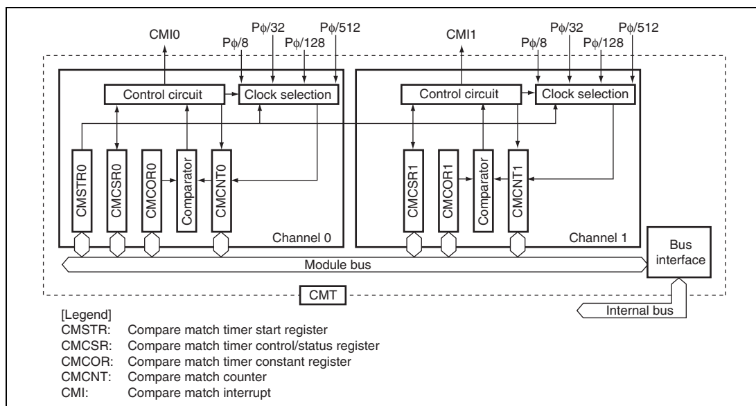
Figure 13.1 Block Diagram of Compare Match Timer
