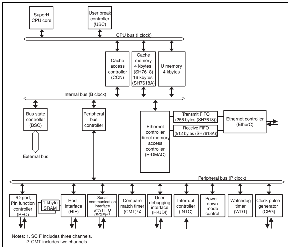
Figure 1.1 Block Diagram
