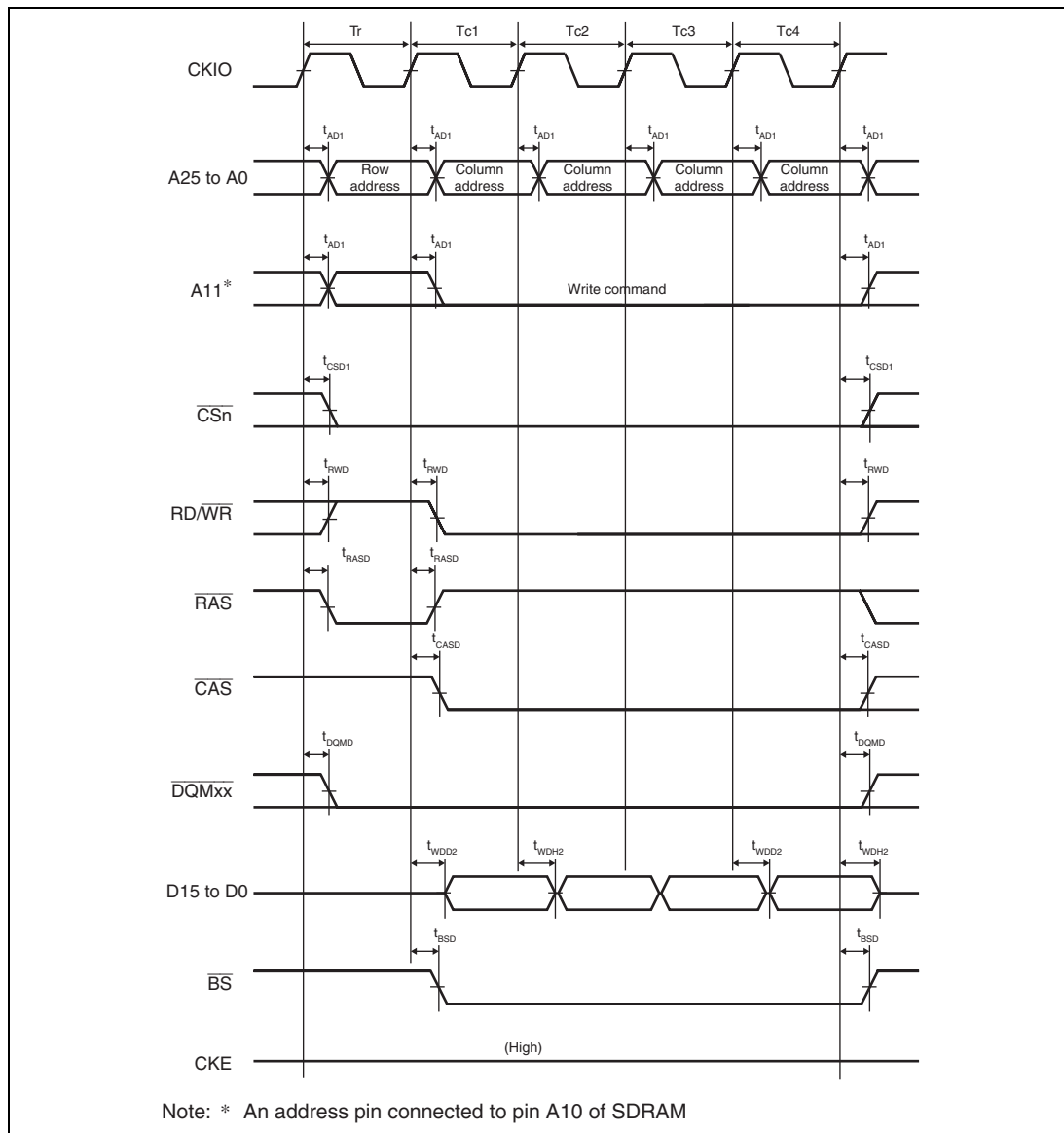
Figure 21.27 Synchronous DRAM Burst Write Bus Cycle (Single Write \times 4 ) (Bank Active Mode: ACT + WRITE Commands, WTRCD = 0 Cycle, TRWL = 0 Cycle)
