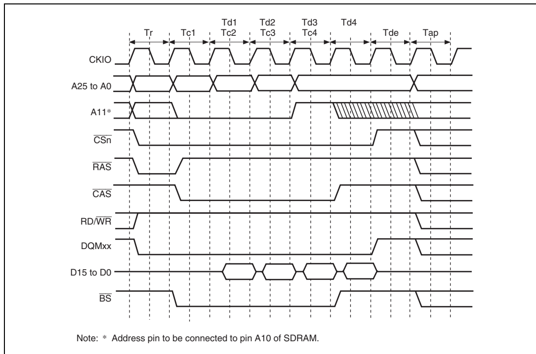
Figure 7.12 Burst Read Basic Timing (Auto Precharge)
