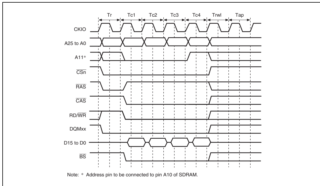
Figure 7.15 Basic Timing for Burst Write (Auto Precharge)
