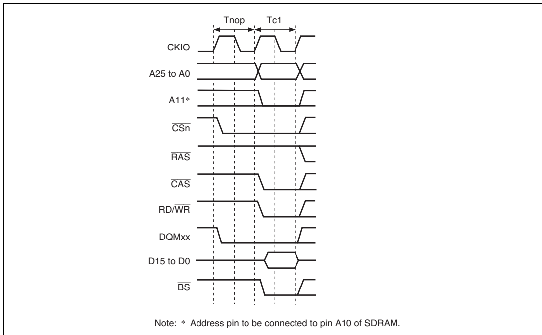
Figure 7.21 Single Write Timing (Bank Active, Same Row Address)
