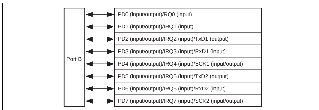
Figure 17.4 Port D
