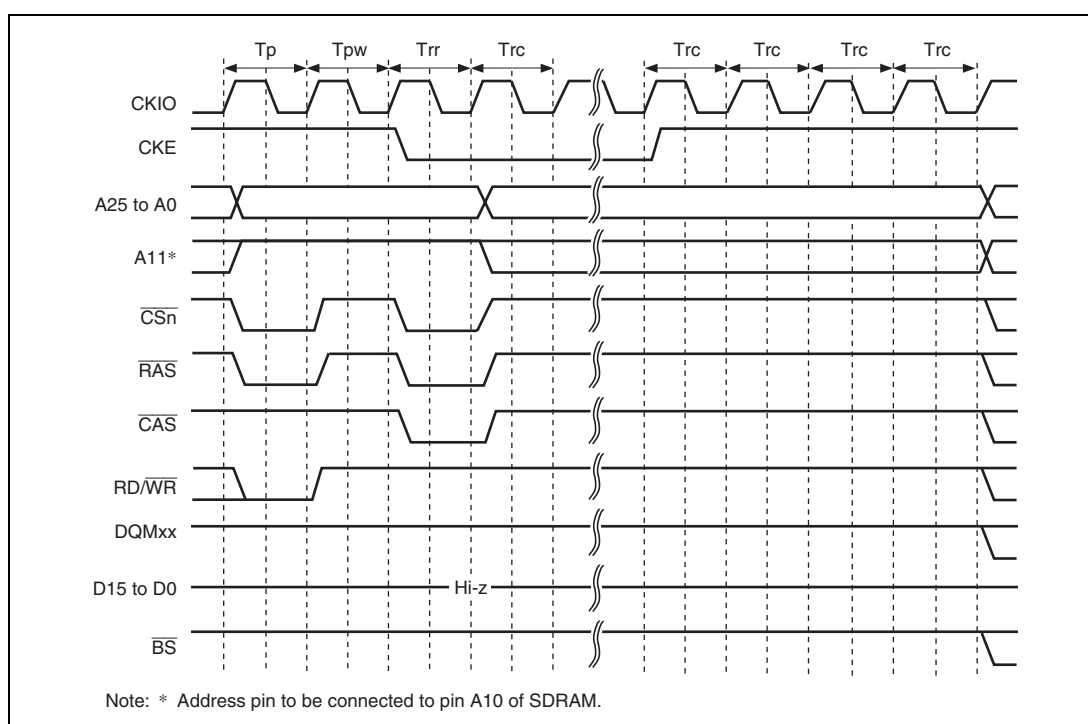
Figure 7.24 Self-Refreshing Timing
