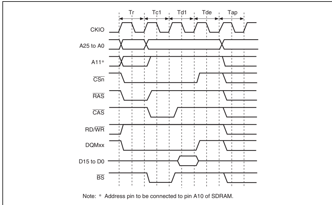
Figure 7.14 Basic Timing for Single Read (Auto Precharge)
