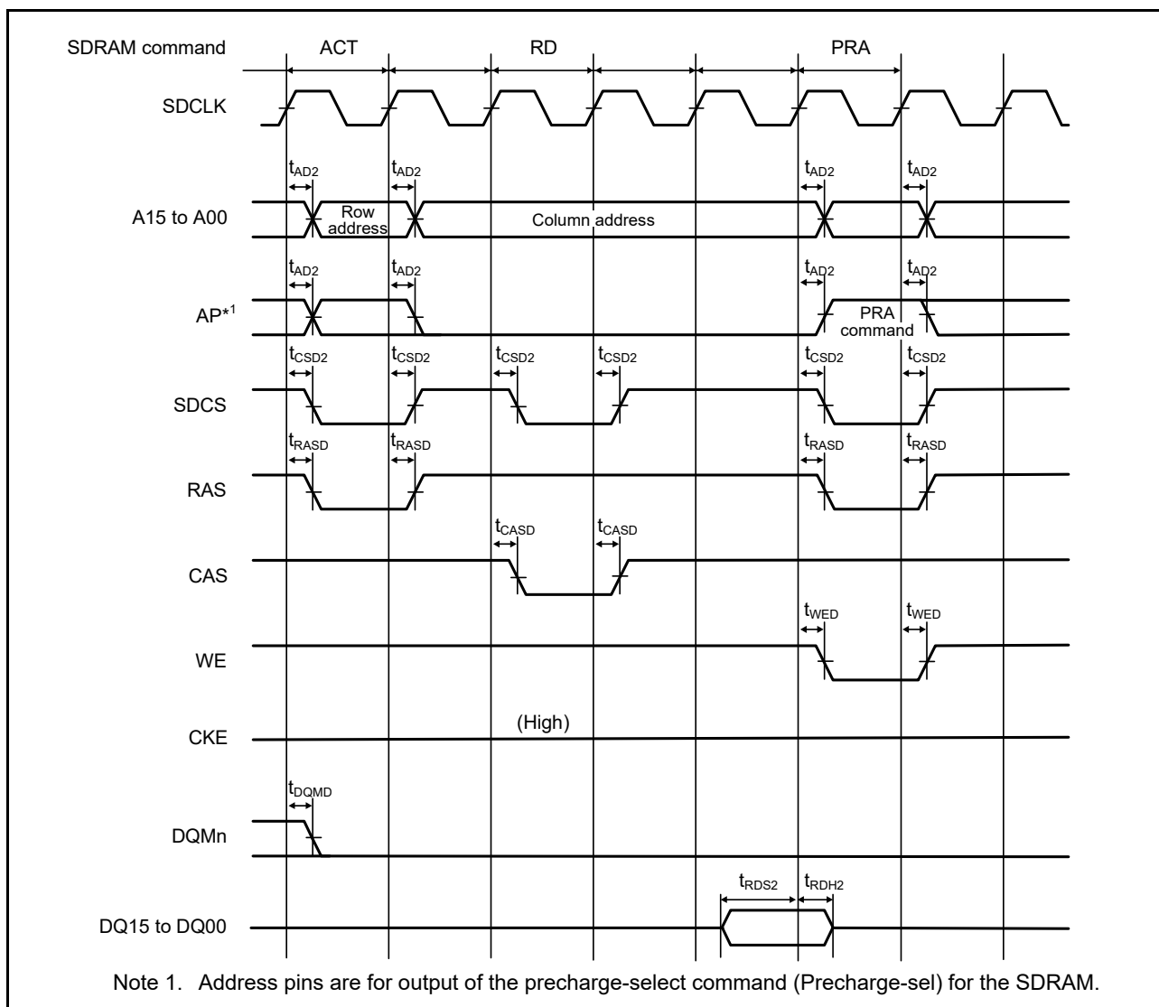
Figure 2.21 SDRAM single read timing
