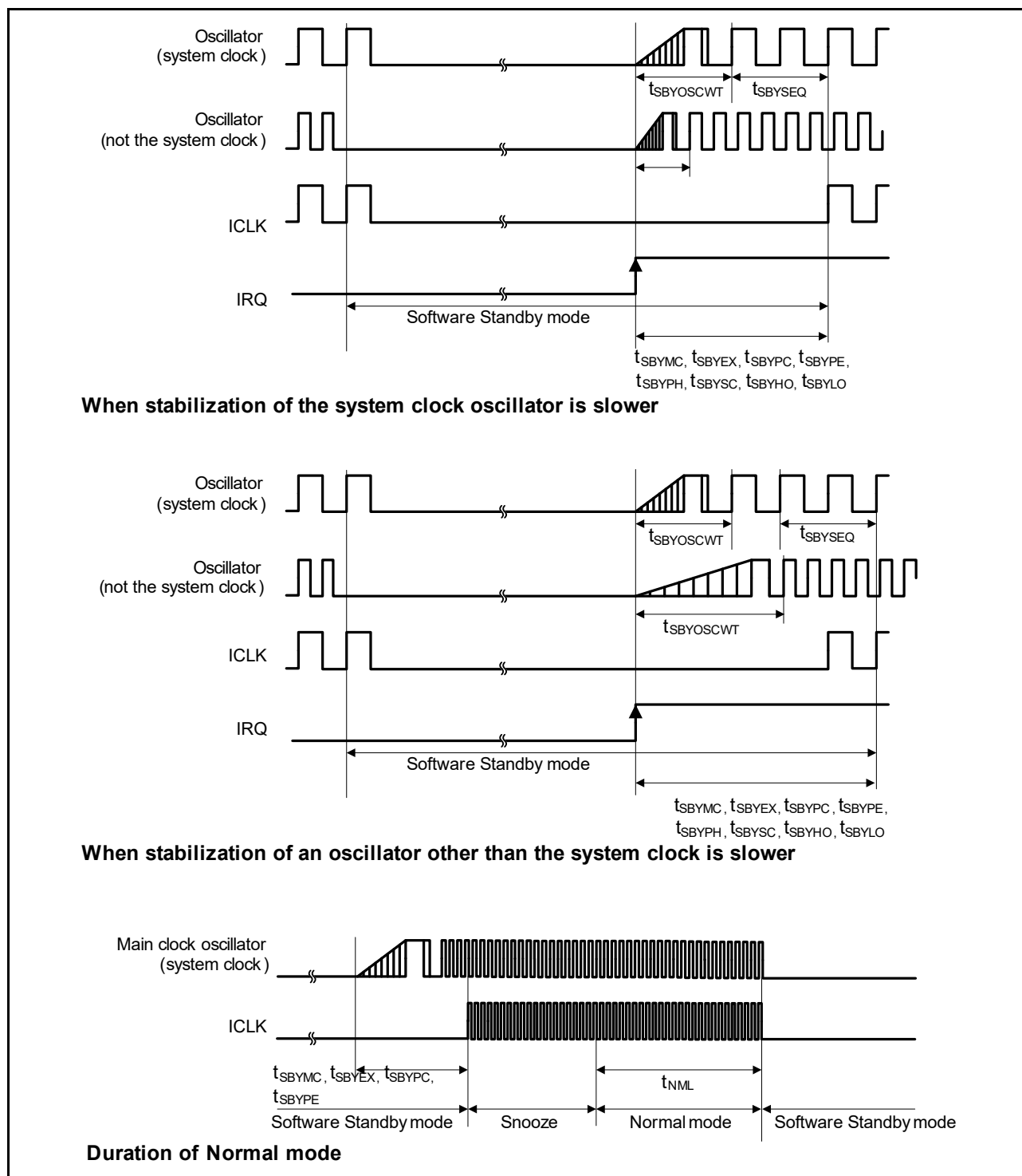
Figure 2.11 Software Standby mode cancellation timing and duration
