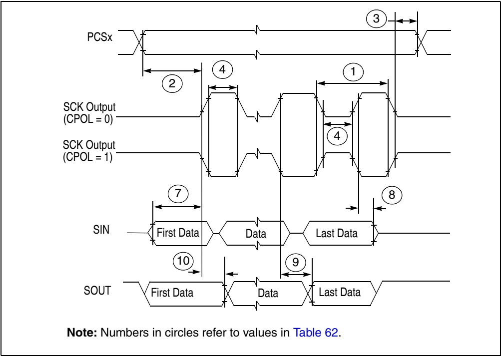
Figure 42. DSPI modified transfer format timing — master, CPHA = 0
