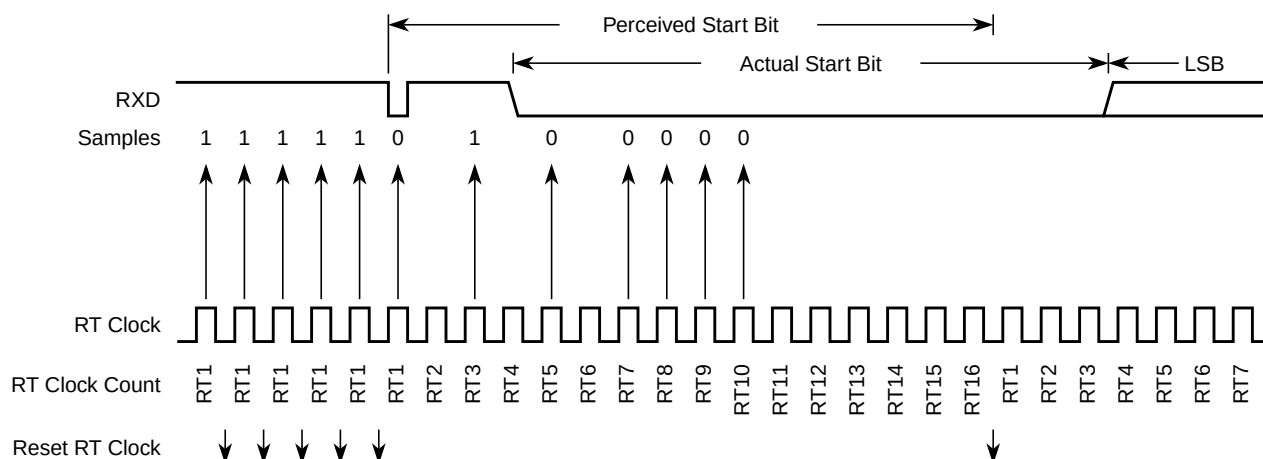
In Figure 15-23, verification sample at RT3 is high. The RT3 sample sets the noise flag. Although the perceived bit time is misaligned, the data samples RT8, RT9, and RT10 are within the bit time and data recovery is successful.
