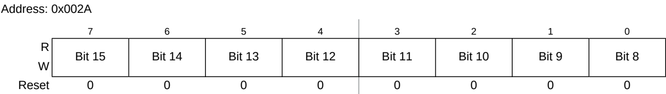
Figure 20-16. Debug Comparator Address Mid Register (DBGXAM)
