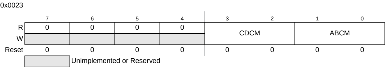
Figure 19-6. Debug Control Register2 (DBGC2)
