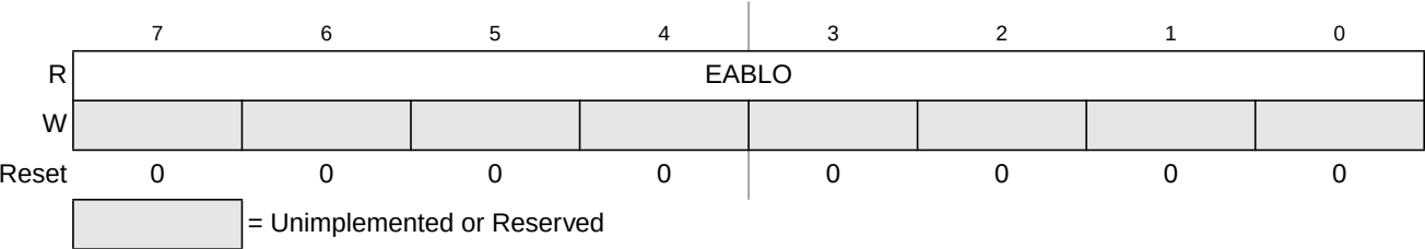
Figure 26-14. EEPROM Address Low Register (EADDRLO)
