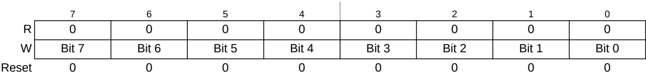
Figure 2-15. ARMCOP Register Diagram
