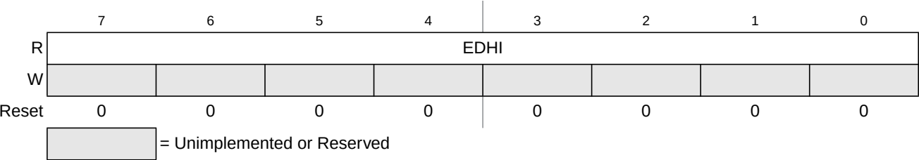
Figure 26-15. EEPROM Data High Register (EDATAHI)
