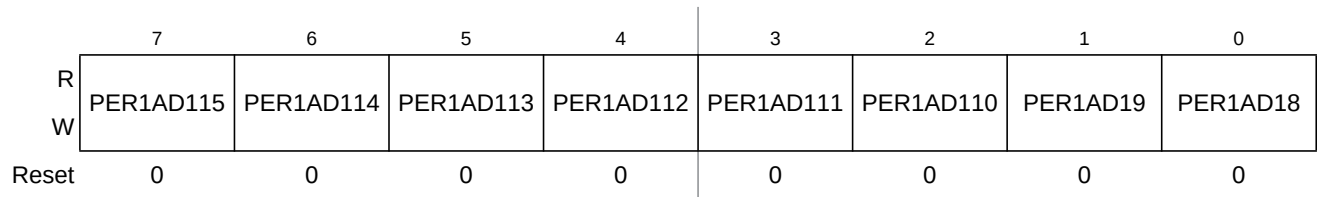
Figure 22-75. Port AD1 Pull Up Enable Register 1 (PER1AD1)
