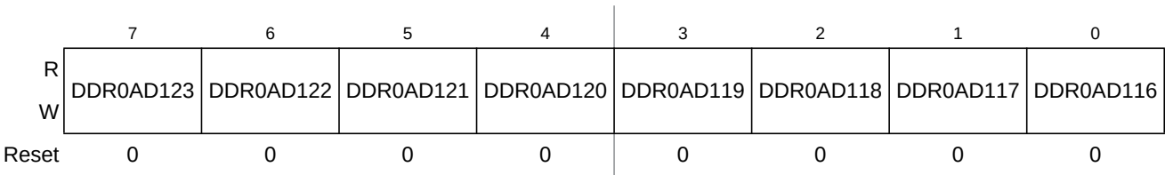
Figure 23-70. Port AD1 Data Direction Register 0 (DDR0AD1)
