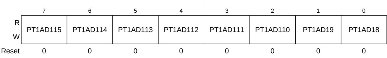
Figure 23-69. Port AD1 Data Register 1 (PT1AD1)
