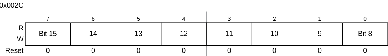
Figure 19-18. Debug Comparator Data High Register (DBGXDH)
