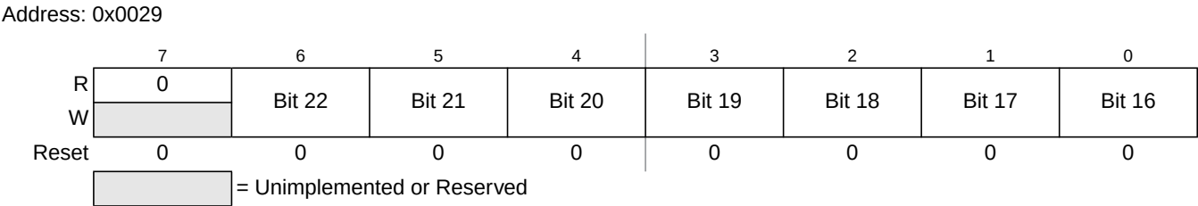
Figure 20-15. Debug Comparator Address High Register (DBGXAH)
