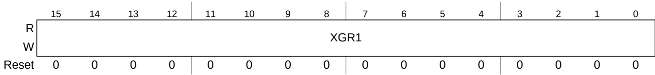
Figure 6-12. XGATE Register 1 (XGR1)
