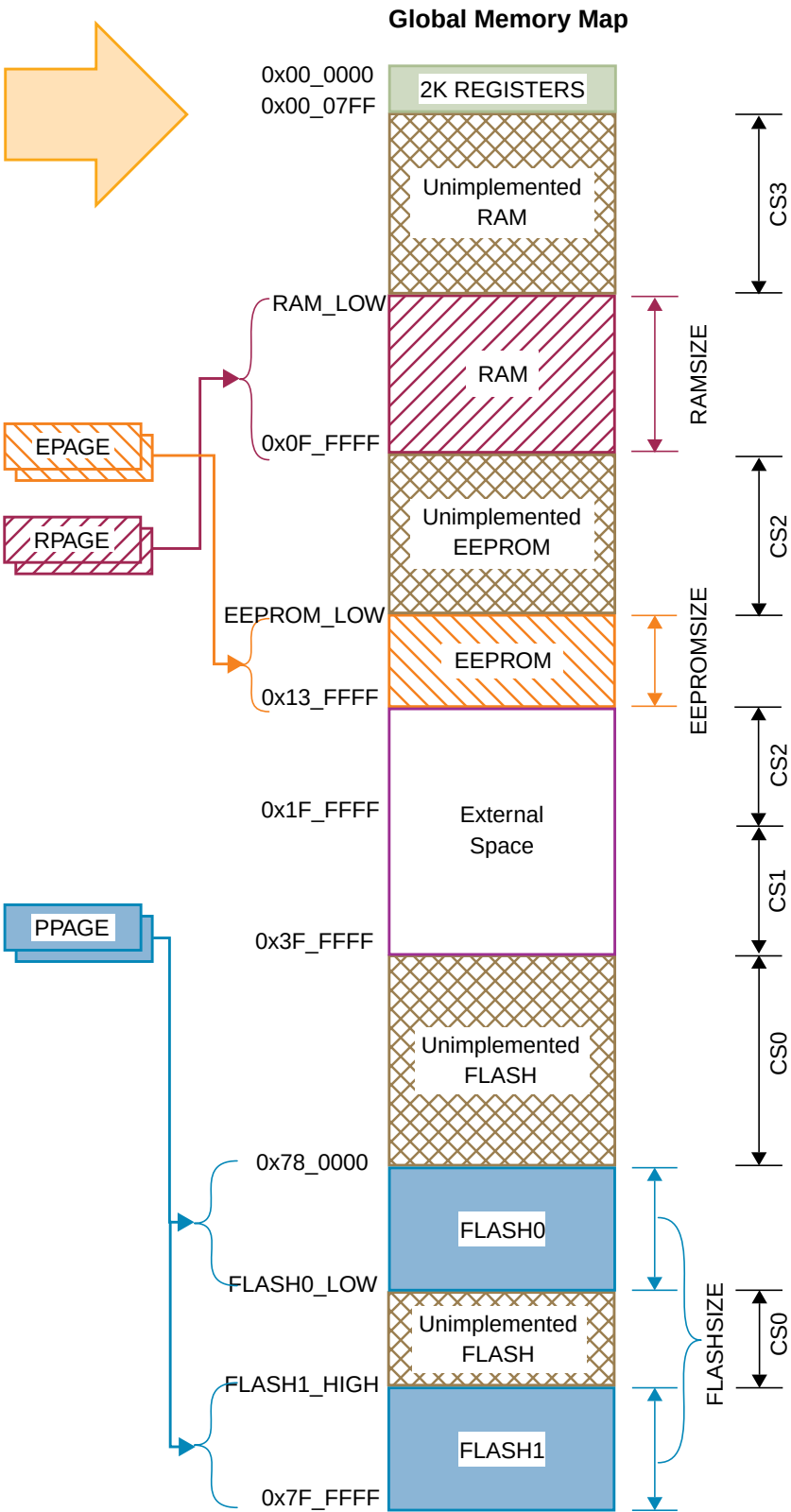
Figure 1-4. S12X CPU & BDM Global Address Mapping
