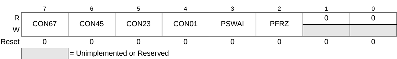
Figure 8-8. PWM Control Register (PWMCTL)
