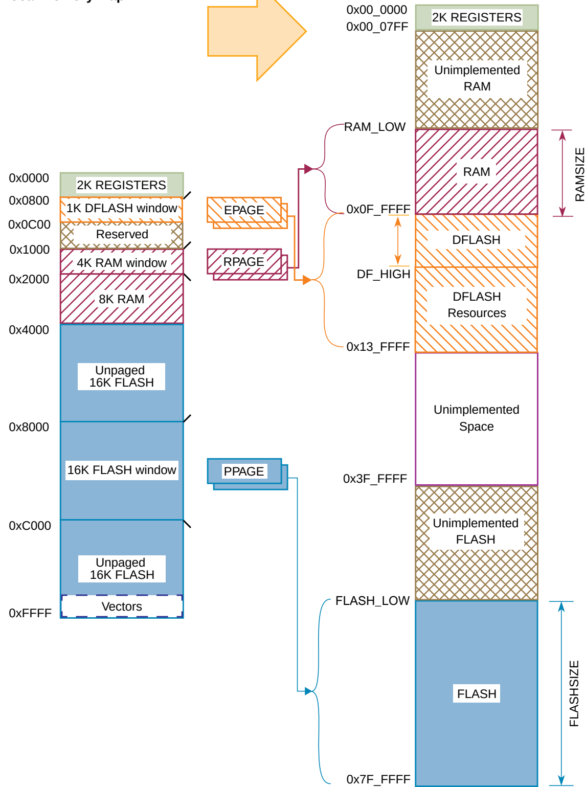
Figure 1-2. S12XS Family Global Memory Map
