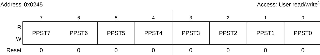
Figure 2-21. Port T Polarity Select Register (PPST)
