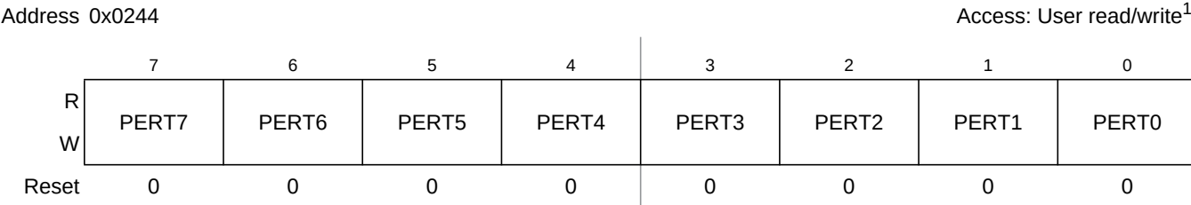
Figure 2-20. Port T Pull Device Enable Register (PERT)
