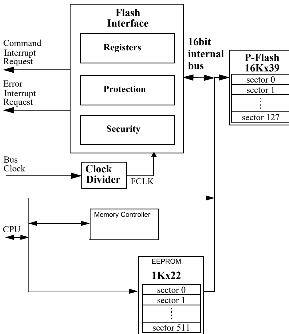
Figure 27-1. FTMRG64K1 Block Diagram
