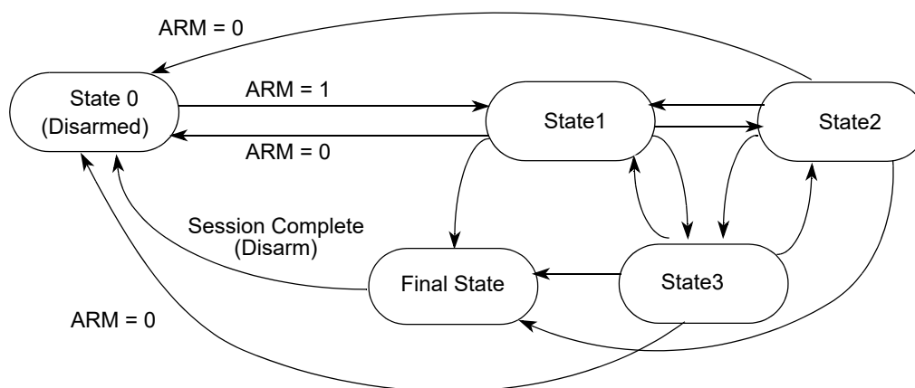
Figure 8-24. State Sequencer Diagram
