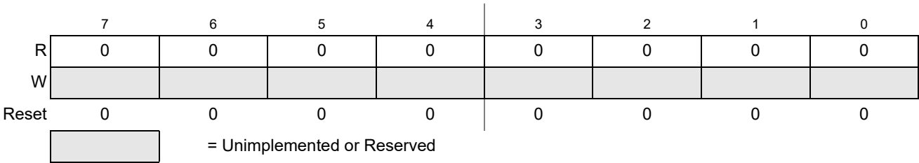
Figure 30-25. Flash Reserved7 Register (FRSV7)
