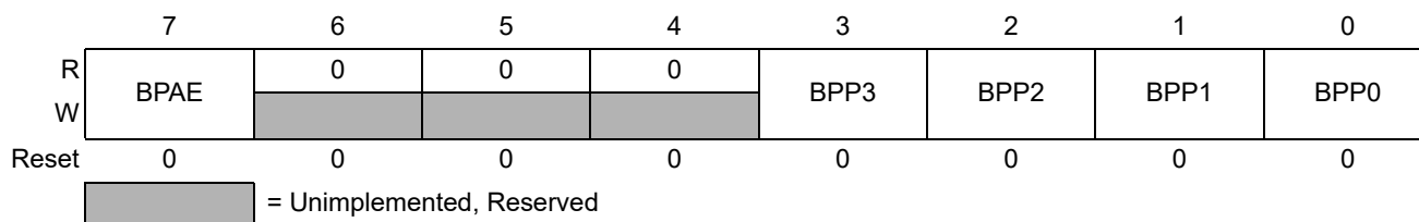
Figure 7-5. BDM Program Page Register (BDMPPR)
