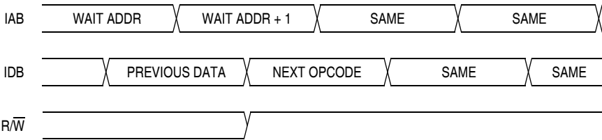
Figure 14-14. Wait Mode Entry Timing
