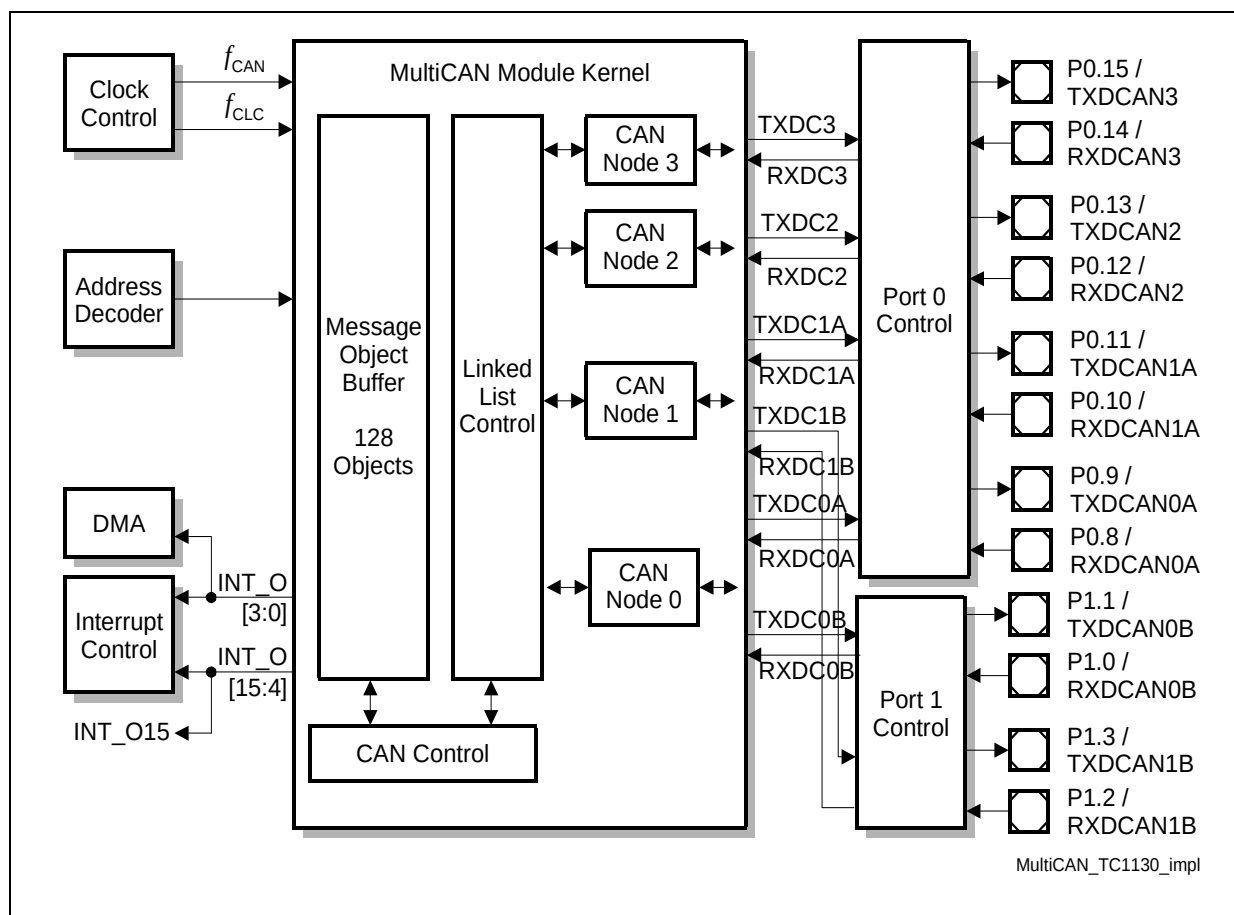
Figure 3-9 General Block Diagram of the MultiCAN Interface
