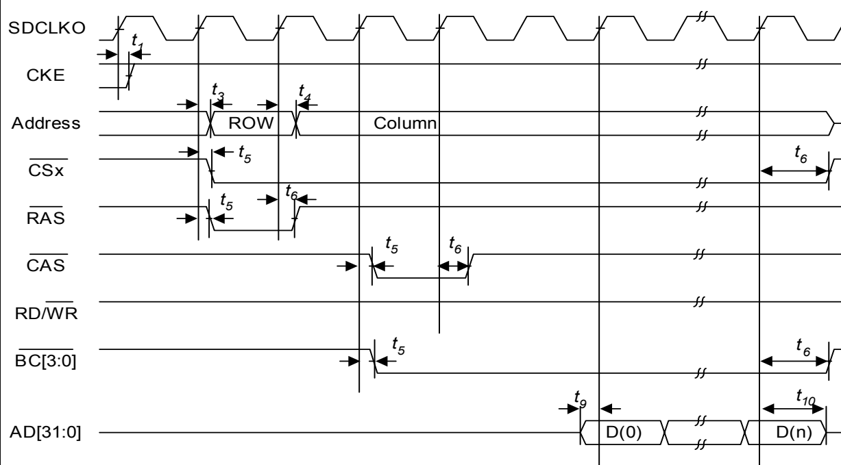
Figure 4-11 SDRAM Access Timing
