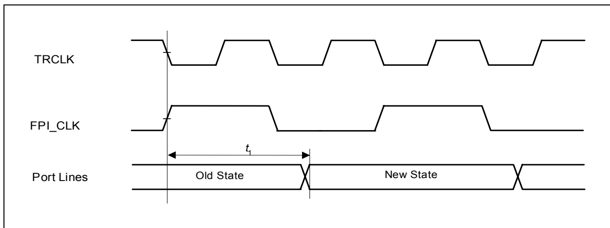
Figure 4-6 Port Timing
