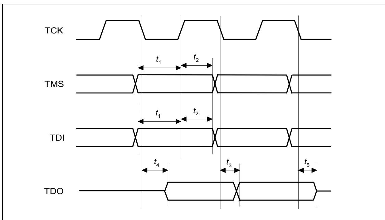
Figure 4-8 JTAG Timing
