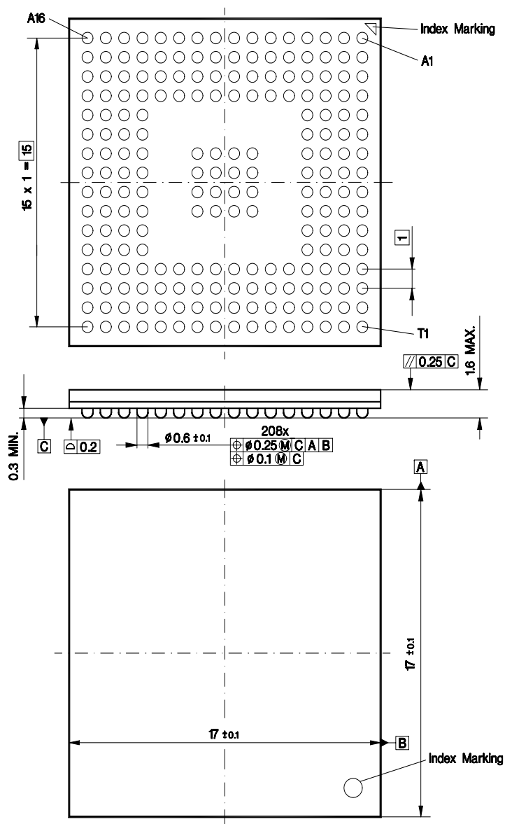
Figure 5-1 P-LBGA-208-2 Package
