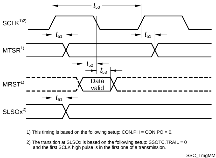
Figure 41 SSC Master Mode Timing
