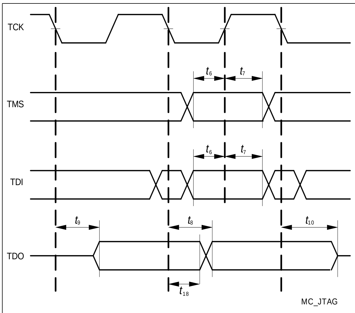
Figure 29 JTAG Timing
