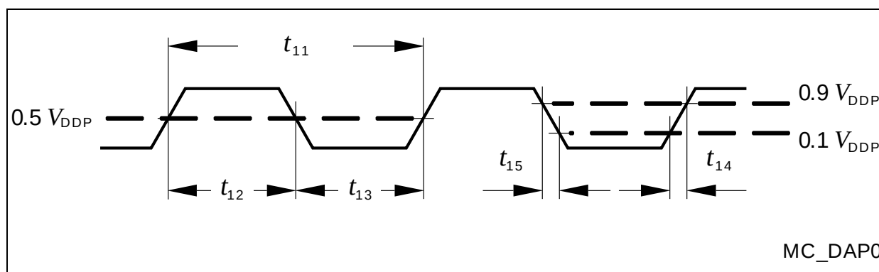
Figure 30 Test Clock Timing (DAP0)
