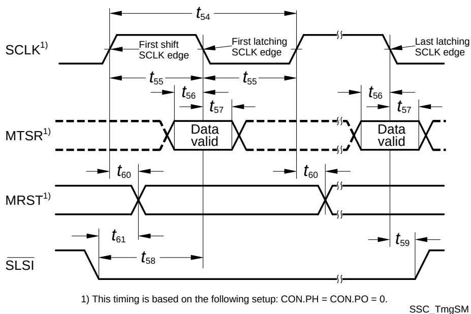
Figure 42 SSC Slave Mode Timing
