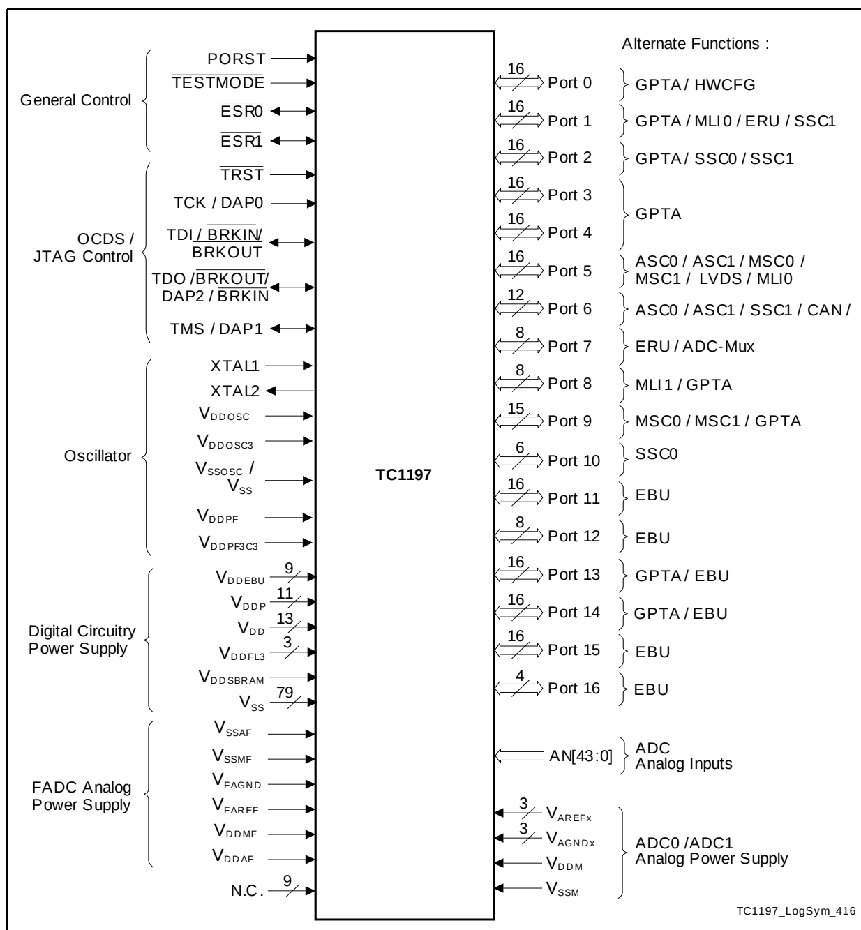
Figure 15 TC1197 Logic Symbol for the package variant PG-BGA-416-10.
