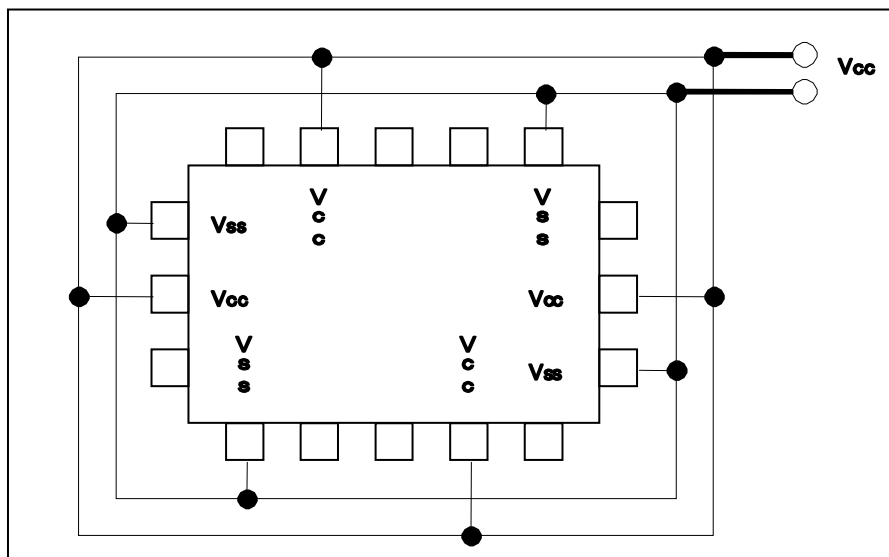
Figure 7-1 Pin Assignment
