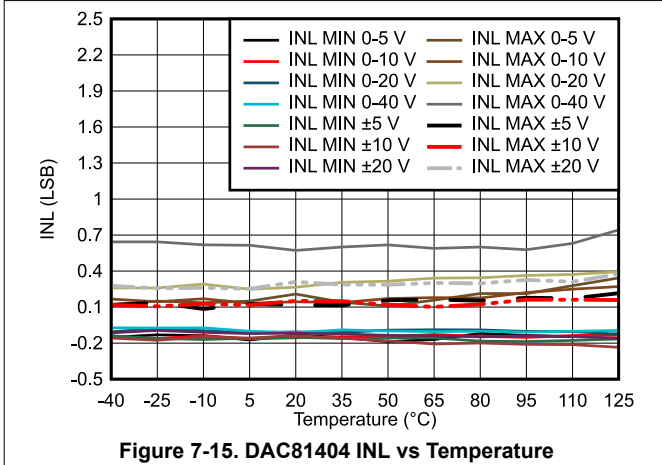
Figure 7-15. DAC81404 INL vs Temperature
