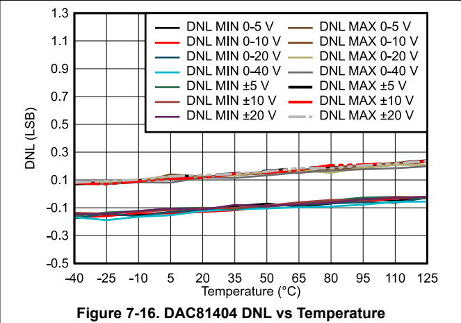
Figure 7-16. DAC81404 DNL vs Temperature
