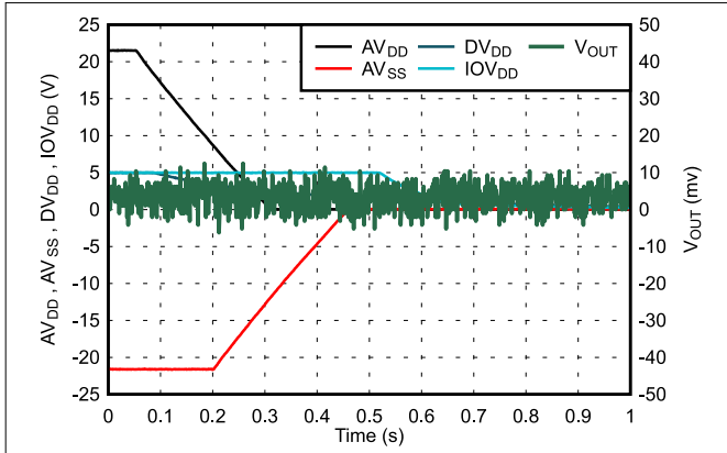
Figure 7-39. Power-Down Response
