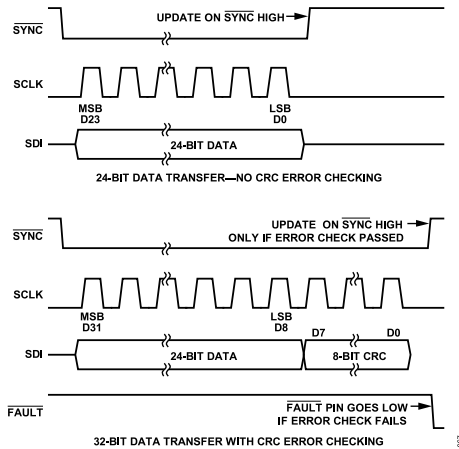
Figure 67. CRC Timing (Assume LDAC = 0)
