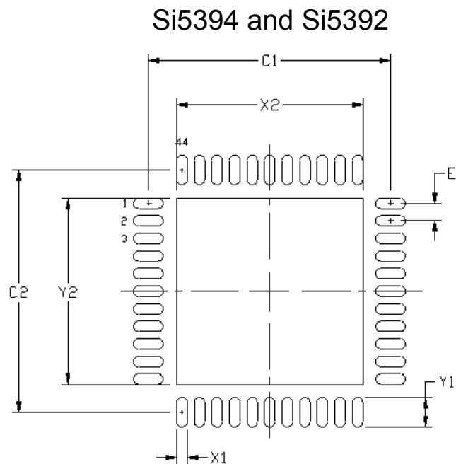
Figure 11.1. PCB Land Pattern
