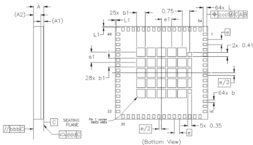
Figure 10.2. 64-Pin LGA
