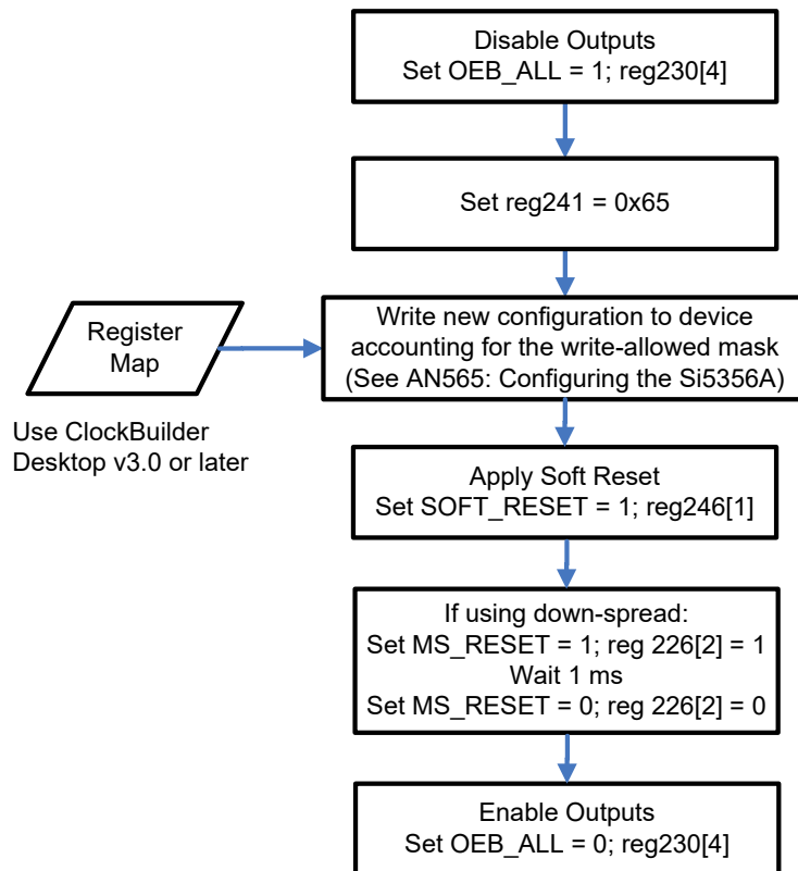
Figure 5. I²C Programming Procedure
